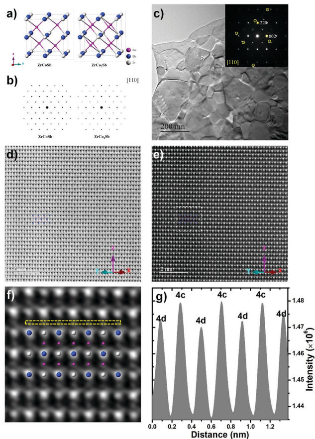
Fig. 8 (a) Lattice unit cells of half-Heusler \text{ZrCoSb} and full-Heusler \text{ZrCo}_2\text{Sb} . (b) The simulated electron diffraction patterns of \text{ZrCoSb} and \text{ZrCo}_2\text{Sb} with beam orientation along the [110] zone-axis. (c) Low-magnification TEM image of \text{ZrCoSb}_{0.7}\text{Sn}_{0.3} , the inset is the indexed selected area electron diffraction (SAED) pattern in [110] zone-axis. (d) Annular-bright-field scanning transmission electron microscopy (ABF-STEM), and (e) high-angle annular-dark-field scanning transmission electron microscopy (HAADF-STEM) image of \text{ZrCoSb}_{0.7}\text{Sn}_{0.3} [110] zone-axis. (f) The magnified HAADF-STEM image of (e), the crystal structure of full-Heusler is also inserted to show the occupation of both 4c and 4d positions. (g) The intensity profile is taken along the 4c/4d plane and integrated over the width of the atomic columns, as indicated by the yellow dashed box in (f). The alternating intensities suggest that the 4d sites are only partially occupied.
