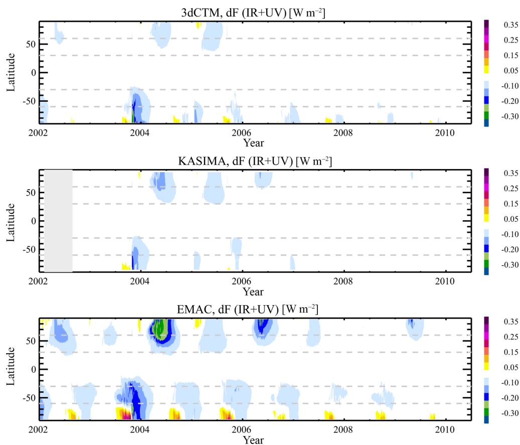
Figure 16. Daily changes in the net amount of energy absorbed or transmitted due to particle-induced ozone destruction in the stratosphere ( \text{W m}^{-2} ), derived from the difference of model runs with model runs without particle forcing, as a function of time and latitude.
