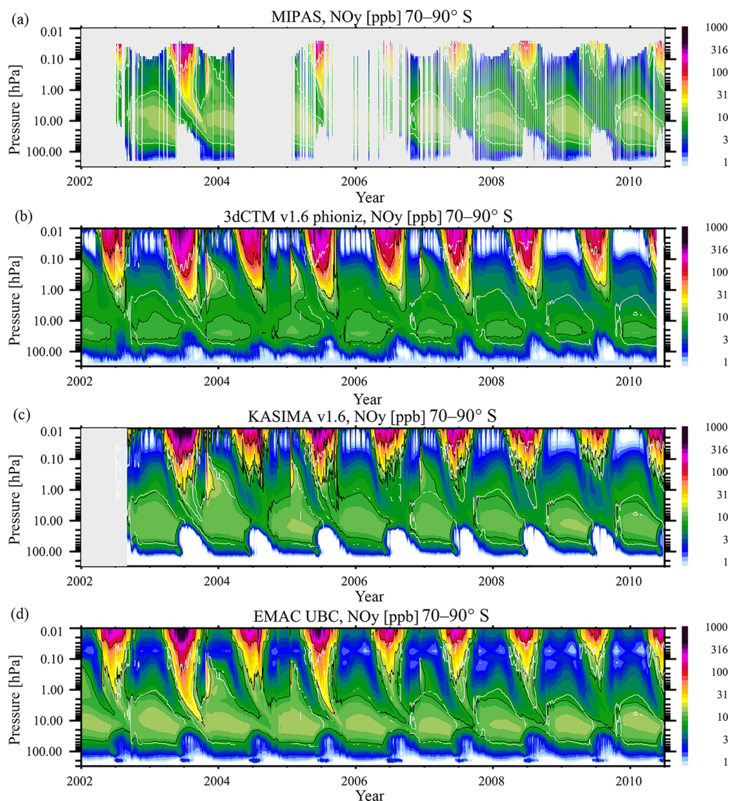
Figure 3. Southern Hemisphere temporal evolution of the volume mixing ratio of \text{NO}_y in all three models and MIPAS measurements in the full common altitude range. (a) MIPAS, (b) 3dCTM, (c) KASIMA, and (d) EMAC. The white contour lines refer to the respective MIPAS values (at 10, 20, 100, and 1000 ppb) smoothed over 7 days for clarity. In black are the respective model contours (not smoothed). The gray shaded areas in the first panel are periods without MIPAS data, and in the third panel, periods before the start of the KASIMA model run.
