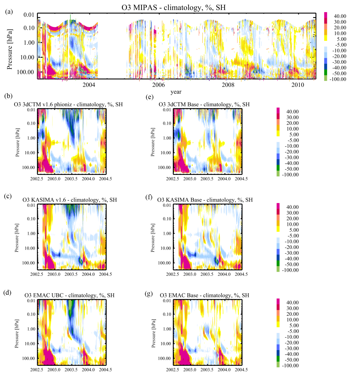
Figure 10. (a) Relative anomalies of MIPAS O 3 compared to a daily climatology derived from the 2006–2009 mean (%) for high southern latitudes (70–90° S) for the period 2002–mid-2010. (b–g) Relative anomalies for the model results, calculated in the same way for mid-2002 to mid-2004. Left: model runs including particle impact; right: model runs without particle impacts. From top to bottom: 3dCTM, KASIMA and EMAC.
