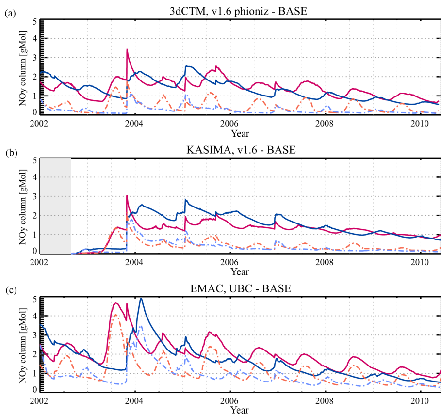
Figure 7. Total EPP \text{NO}_y (Gmol) in the middle atmosphere as the difference between model runs with and without particle forcings. From top to bottom: 3dCTM, KASIMA, and EMAC. Red: hemispheric amount in the Southern Hemisphere; blue: hemispheric amount in the Northern Hemisphere; solid lines, dark colors: 200–0.01 hPa (lower stratosphere to mesopause); dashed lines, light colors: 9–0.01 hPa (mid-stratosphere to mesopause). The gray shading in the second panel denotes the period at the start where KASIMA results were not yet available.
