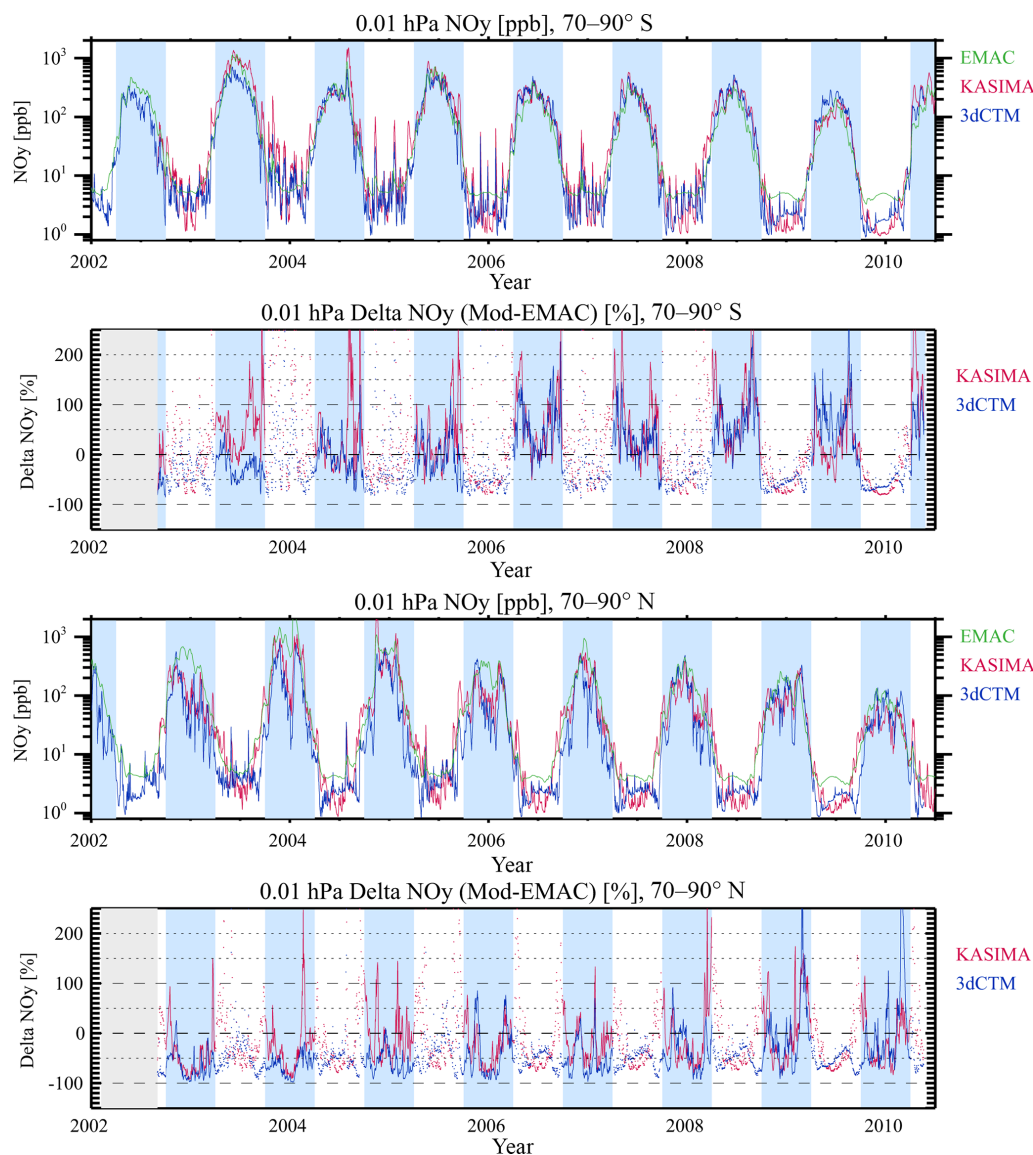
Figure 2. Temporal evolution of the volume mixing ratio of \text{NO}_y (ppb) from all three models at high southern and northern latitudes ( 70\text{--}90^\circ \text{S/N} ), at 0.01 hPa. Also shown are relative differences from KASIMA and 3dCTM to EMAC results (%). Light blue shading denotes winter in the Southern Hemisphere/Northern Hemisphere (second and third quarters of each year/first and fourth quarters of each year). The gray shading in the difference plots denotes the period at the start where KASIMA results were not yet available. To highlight differences in polar winter, differences in summer are shown as dots, while differences in winter are shown as solid lines. KASIMA: red; 3dCTM: blue; EMAC: green.
