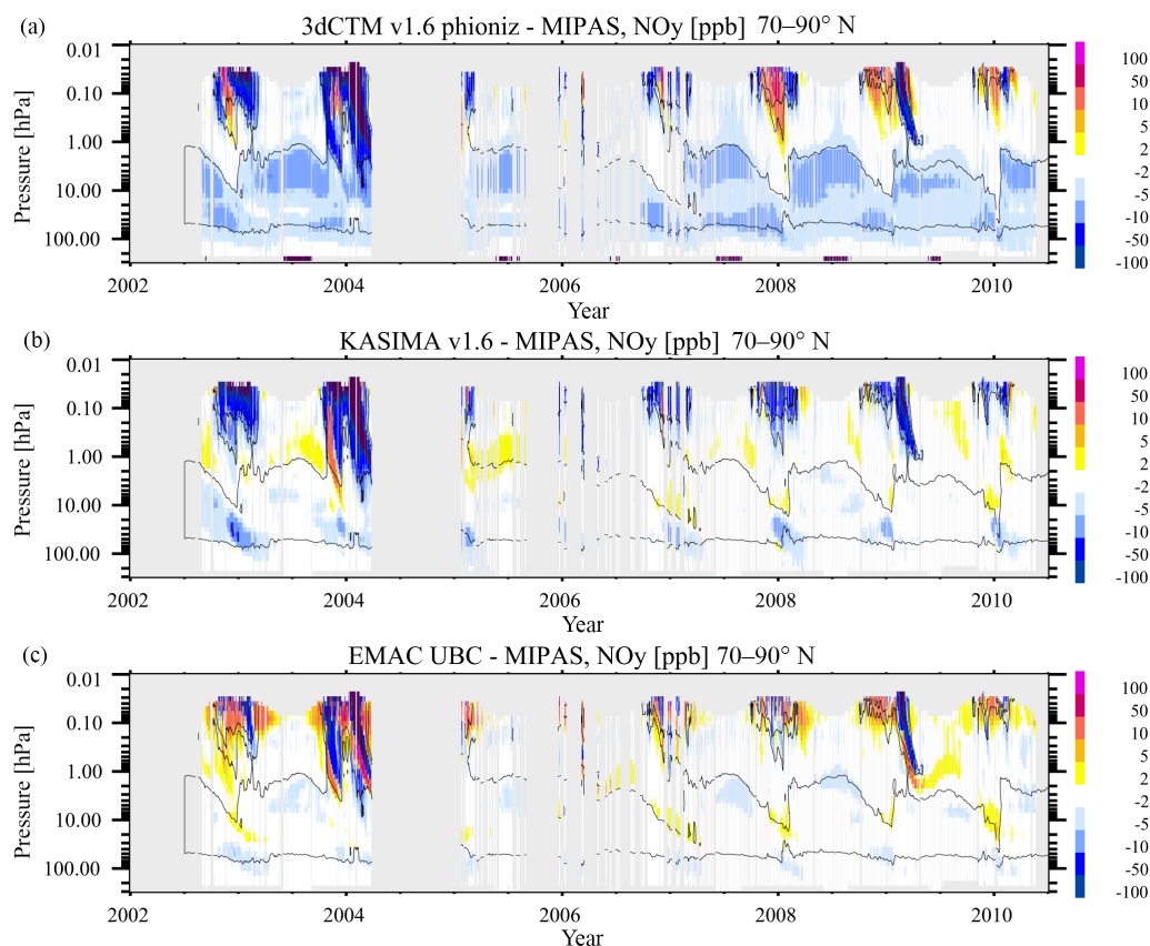
Figure 6. Absolute difference in \text{NO}_y (ppb) between models and MIPAS observations at high northern ( 70\text{--}90^\circ\text{N} ) latitudes. Model data have been interpolated to the vertical grid of the MIPAS data, and only days and altitudes are shown where MIPAS data are available and fulfill the averaging kernel criterion. From top to bottom: 3dCTM v1.6 phioniz, KASIMA v1.6, and EMAC UBC. The black lines show the 10, 20, and 3000 ppb contours of the MIPAS data, smoothed with a 7-day running mean for clarity. The gray shaded areas are periods without MIPAS data, and in the second panel the period before the start of the KASIMA model run is also shown.
