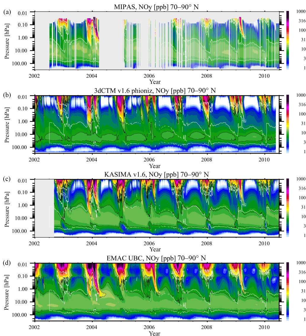
Figure 4. Northern Hemisphere temporal evolution of the volume mixing ratio of \text{NO}_y in all three models and MIPAS measurements in the full common altitude range. (a) MIPAS, (b) 3dCTM, (c) KASIMA, and (d) EMAC. The white contour lines refer to the respective MIPAS values (at 10, 20, 100, and 1000 ppb) smoothed over 7 days for clarity. In black are the respective model contours (not smoothed). The gray shaded areas in the first panel are periods without MIPAS data, and in the third panel, the period before the start of the KASIMA model run.
