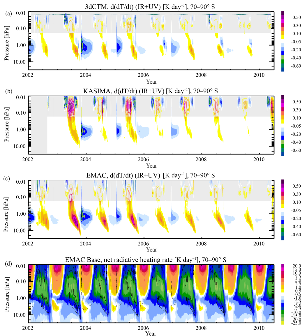
Figure 14. Changes in daily net radiative (shortwave and longwave) heating rates ( \text{K day}^{-1} ) due to particle-induced ozone changes derived from all three models ( a : 3dCTM; b : KASIMA; c : EMAC) at high southern latitudes ( 70\text{--}90^\circ\text{ S} ). ( d ) The net radiative heating rate (sum of the shortwave and longwave contributions) in the EMAC Base scenario ( \text{K day}^{-1} ). Black dashed lines are the -0.1 and -0.5 \text{ K day}^{-1} contours of the net radiative heating rate change in EMAC; black solid lines are the +0.1 and +0.5 \text{ K day}^{-1} contours.
