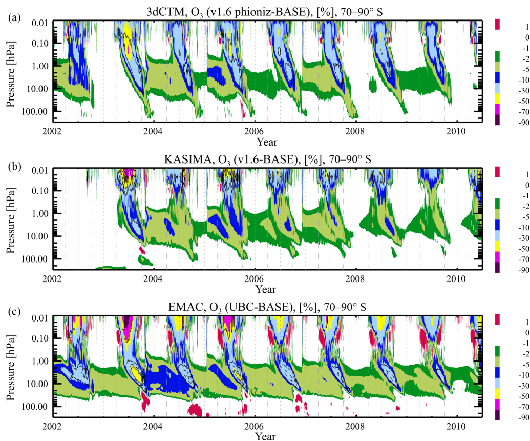
Figure 12. Relative ozone anomalies due to energetic particle precipitation at high southern latitudes (70–90° S), calculated as the difference of model runs with to without particle impact (%). (a) 3dCTM (v1.6 phioniz – Base), (b) KASIMA (v1.6 – Base), (c) EMAC (UBC – Base). The gray shaded area in the middle figure denotes the time period before the start of the KASIMA model runs. Dashed and dotted vertical gray lines mark zero, one-quarter, one-half, and three-quarters of each year. The thin black contours refer to -1.5 (solid), -1 (dashed) and -0.5 (solid) ppm.
