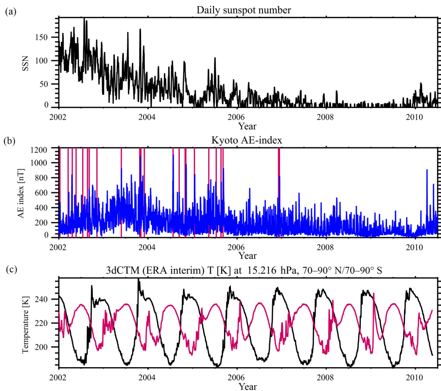
Figure 1. (a) Daily sunspot number from www.ngdc.noaa.gov/stp/spidr.html , May 2012. (b) Daily mean AE index from the Kyoto database ( http://wdc.kugi.kyoto-u.ac.jp , February 2016). Red lines denote days of strong solar proton events as given by http://umbra.nascom.nasa.gov/SEP/ , February 2017 (see text). For events lasting more than 1 day, only the first day is marked. (c) Temperature in the mid-stratosphere (15.216 hPa) at high southern (black, 70–90° S) and high northern (red, 70–90° N) latitudes. Data are taken from output of the 3dCTM, but originate from ERA-40. The tick marks here and in all the following figures mark the first day of a year.
