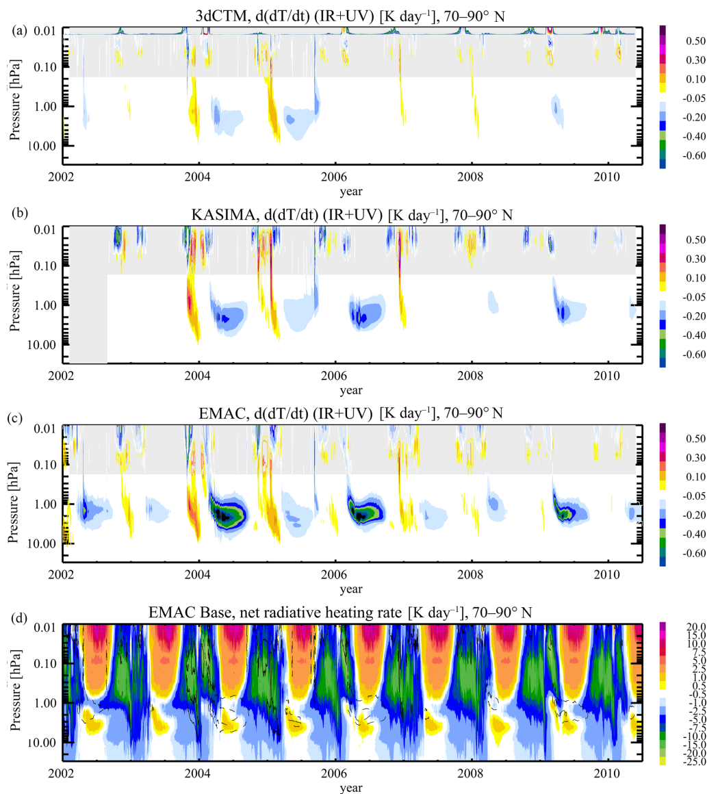
Figure 15. Changes in daily net radiative (shortwave and longwave) heating rates ( \text{K day}^{-1} ) due to particle-induced ozone changes derived from all three models ( a : 3dCTM; b : KASIMA; c : EMAC) at high northern latitudes ( 70\text{--}90^\circ\text{N} ). ( d ) The net radiative heating rate (sum of the shortwave and longwave contributions) in the EMAC Base scenario ( \text{K day}^{-1} ). Black dashed lines are the -0.1 and -0.5 \text{ K day}^{-1} contours of the net radiative heating rate change in EMAC; black solid lines are the +0.1 and +0.5 \text{ K day}^{-1} contours.
