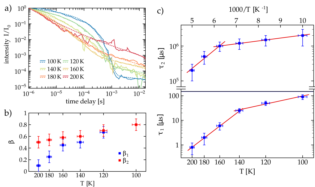
Figure 7. (a) Normalized time-dependent photoluminescence of 7 mol % Mg:CLN for various temperatures (continuous line) and stretched-exponential fits (dashed lines) under nanosecond-pulsed UV illumination. (b) Plots of \beta_1 and \beta_2 from these fits over temperature. (c) Arrhenius plots of lifetimes \tau_1 and \tau_2 (logarithmic plots over 1/T ). These diagrams are reproduced from our previous publication T. Kämpfe et al., Phys. Rev. B 2016 , 93 , 174116 [19]; for this publication, new fits have been made for all parts of the curves in (c).
