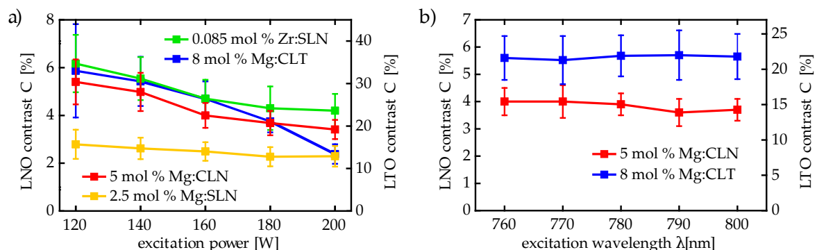
Figure 13. (a) Power dependence of domain contrasts for 5 mol % Mg:CLN, 2.5 mol % Mg:SLN, 0.085 mol % Zr:SLN and 8 mol % Mg:CLT, recorded with three-photon femtosecond excitation at 790 nm. (b) Excitation wavelength dependence of domain contrasts of 5 mol % Mg:CLN and 8 mol % Mg:CLT with total emitted photoluminescence intensity kept constant.
