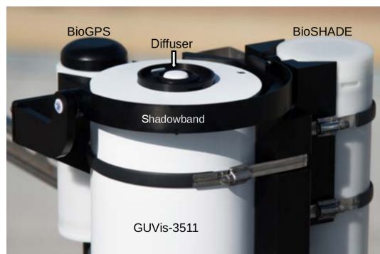
Figure 1. The radiometer GUVis-3511 (center) with the BioSHADE accessory (right), which drives the shadowband. The BioGPS accessory is shown in the background on the left. The small white dome in the center of the radiometer top is the diffuser, which covers the filtered detectors.
