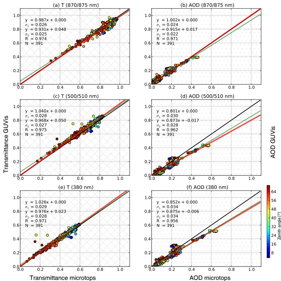
Figure 9. As in Fig. 6 but for the comparison of the GUVis and Microtops instruments during PS83.
