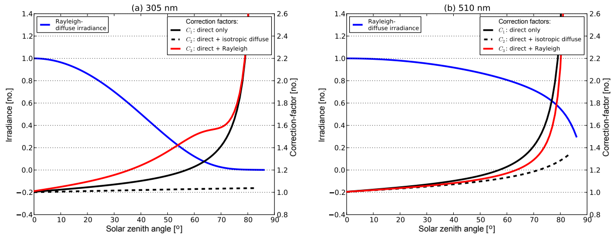
Figure 4. Factors for motion correction measurements of the 305 and 510 nm GUVis channels. The two panels show the calculated diffuse irradiance (blue, left y axis), which is normalized to its maximum. The three correction factors are shown with respect to the right y axis, calculated for an inclination of 6^\circ of the ship towards the sun's azimuth angle (e.g., high swell). The direct only (black solid) correction factor refers to C_1 described by Bannehr and Schwiesow (1993). The correction factors C_2 (black dashed) and C_3 (red) are calculated taking direct and diffuse irradiance into account. For C_2 , an isotropic diffuse radiance distribution is assumed. C_3 is calculated assuming Rayleigh scattering.
