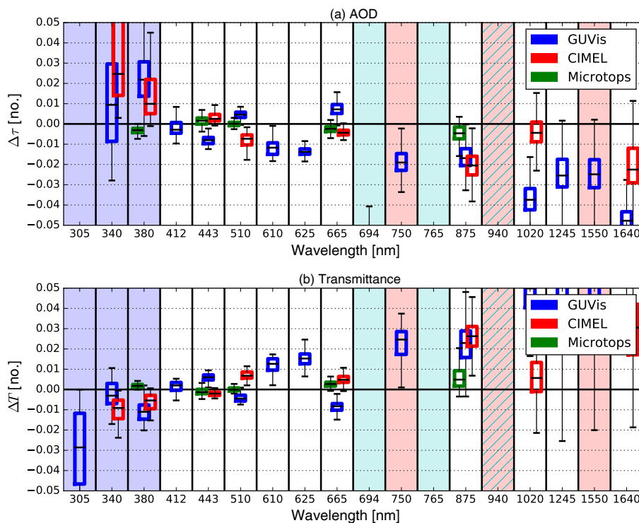
Figure 12. The panels show (a) AOD and (b) transmittance observations compared to values calculated with Eq. (25), which are expressed as difference of calculated and observed value. The Ångström exponent and curvature term are derived from a least-squared fit of the instrument AOD with 500 nm as the basis wavelength. The observations took place during the Melpitz Column experiment from May to July 2015 for the Cimel and GUVIs instruments and at PS83 for the Microtops instrument. The channels are color-coded for known calibration or correction issues. Blue indicates issues with the radiation inlet, red channels rely on soft-coated filters, and channels marked with cyan are not corrected for gas absorption of \text{H}_2\text{O} and \text{O}_2 . The data are displayed in a box and whisker plot. Shown are the median, boxes extending to the 25th percentile, and whiskers extending to the 75th percentile of the data.
