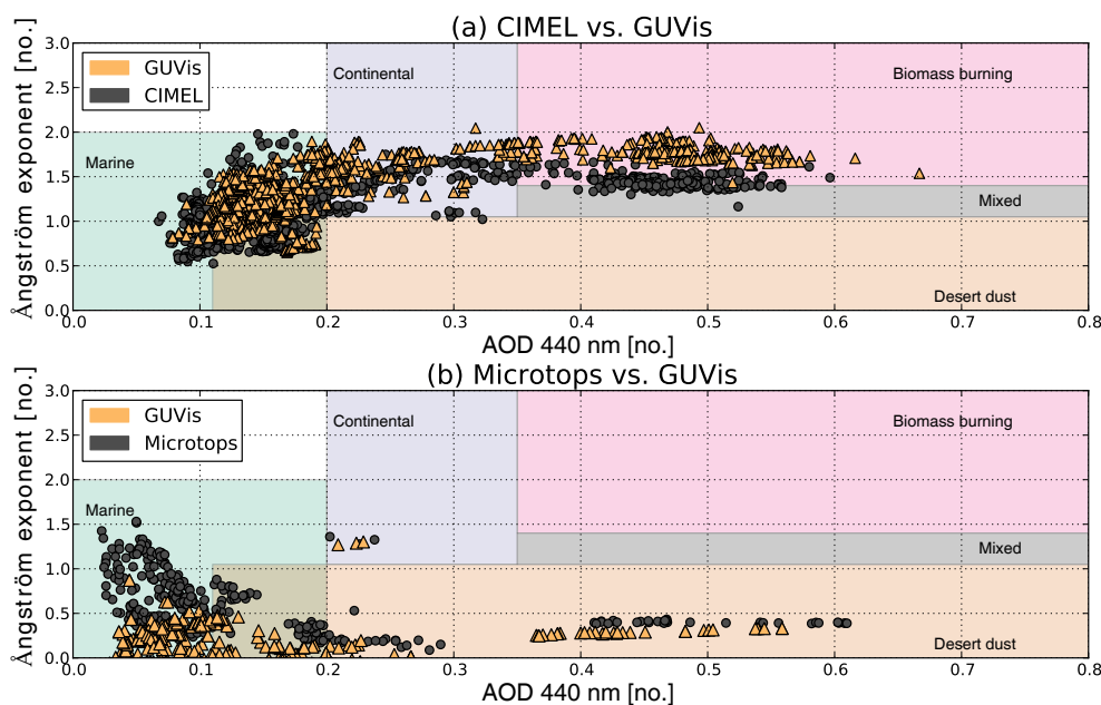
Figure 11. The panels show (a) land-side and (b) shipborne observations using the Ångström exponent (440–870 nm) and the AOD at 440 nm for aerosol classification as described by Toledano et al. (2007). Sunphotometer observations (grey) are compared to GUVIs observations (orange).
