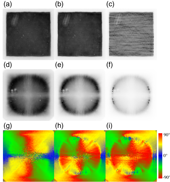
Figure 3: (Color online) Near- and far-field images for device #2 below and above threshold. Heat sink temperature T=0\text{ }^{\circ}\text{C} and driving current 13.5 mA (a,d,g), 15.5 mA (b,e,h), and 16.0 mA (c,f,i). The white spots in (a,b) result from debris on the neutral density filters. The color code is the same as in Fig. 2. These images correspond to the transition shown in Fig. 6.
