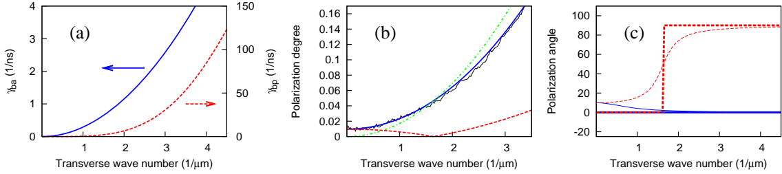
Figure 8: (Color online) (a) The amplitude \gamma_{ba} (blue, solid line) and phase \gamma_{bp} (red, dashed line) anisotropy induced by the Bragg reflector. (b) The degree of polarization for the parameters of device #1 (see Fig. 4) and k_y = 0 according to theoretical calculations. The polarization degree inside the cavity is indicated by the red dashed line, outside the cavity by the blue solid line. The corresponding experimental curve is depicted by the black line. The extra-cavity polarization in the “pure filtering limit” (i.e. assuming completely unpolarized light inside the cavity) is indicated by the green dot-dashed line. (c) The polarization direction inside (red dashed lines) and outside (blue solid lines) the cavity for the intra-cavity anisotropy favoring x -polarization (thick lines, as in panel b) or an anisotropy favoring a polarization direction of 10^\circ (thin lines).
