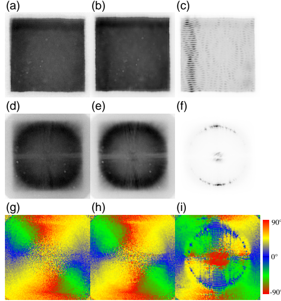
Figure 2: (Color online) Near- and far-field images for device #1 below and above threshold. Heat sink temperature T=0^\circ\text{C} and driving current 12.0 mA (a,d,g), 13.5 mA (b,e,h), and 15.6 mA (c,f,i). The color-code of the polarization direction distribution (lowest row) is shown by the bar on the lower right. These images correspond to the transition shown in Fig. 5.
