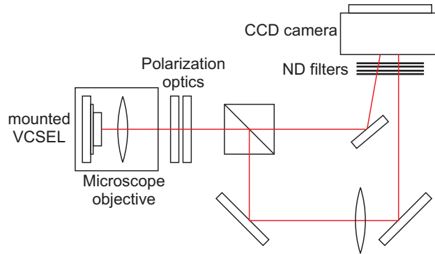
Figure 1: (Color online) Experimental setup. The VCSEL is set into an air-tight box to avoid condensation water. Polarization optics: half-wave plate and linear polarizer.
