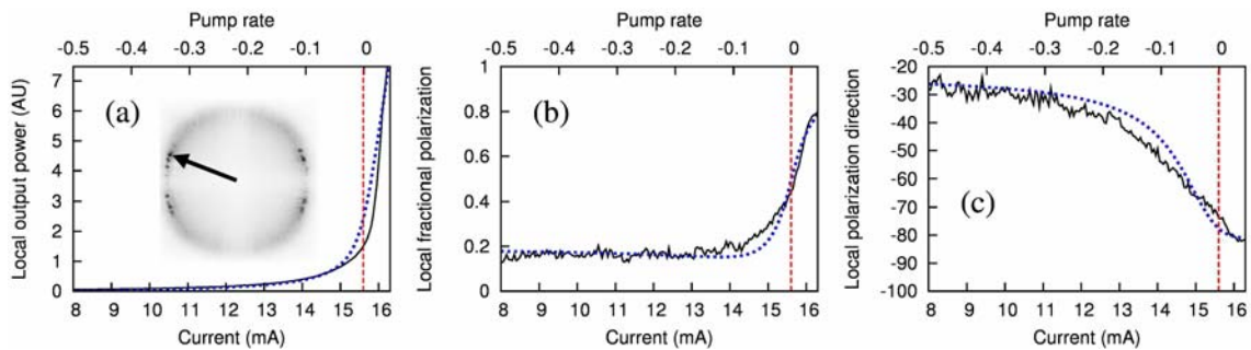
Figure 6: (Color online) Transition from spontaneous emission to lasing emission of the spot depicted in the inset in (a) for device #2. (a) Local intensity in dependence on driving current. (b) Degree of polarization. (c) Local polarization direction. All denotations are analogous to Fig. 5.
