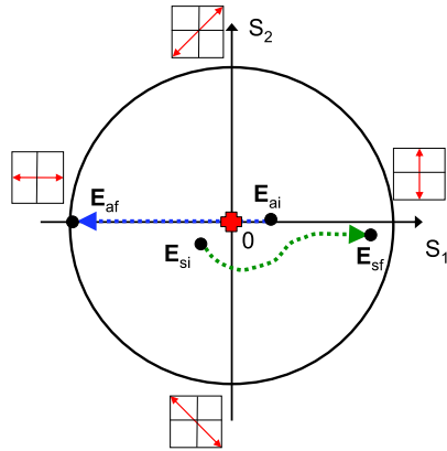
Figure 7: (Color online) Different types of transitions from non-lasing to lasing state in the space of Stokes parameters ( S_1, S_2 ): Abrupt transition (blue straight dashed arrow from \mathbf{E}_{ai} to \mathbf{E}_{af} , corresponds to device #1) and smooth transition (green curved dashed arrow from \mathbf{E}_{si} to \mathbf{E}_{sf} , corresponds to device #2). The initial polarization state for the abrupt transition \mathbf{E}_{ai} is orthogonally polarized to the final one \mathbf{E}_{af} , whereas for the initial \mathbf{E}_{si} and final \mathbf{E}_{sf} states for the smooth transition this is not the case. For convenience, the polarizations directions for different quadrants of ( S_1, S_2 )-plane are shown by red arrows in the black boxes. The red cross in the center corresponds to a fully unpolarized state ( p = 0 ) whereas the black circle shows the fully polarized state ( p = 1 ).
