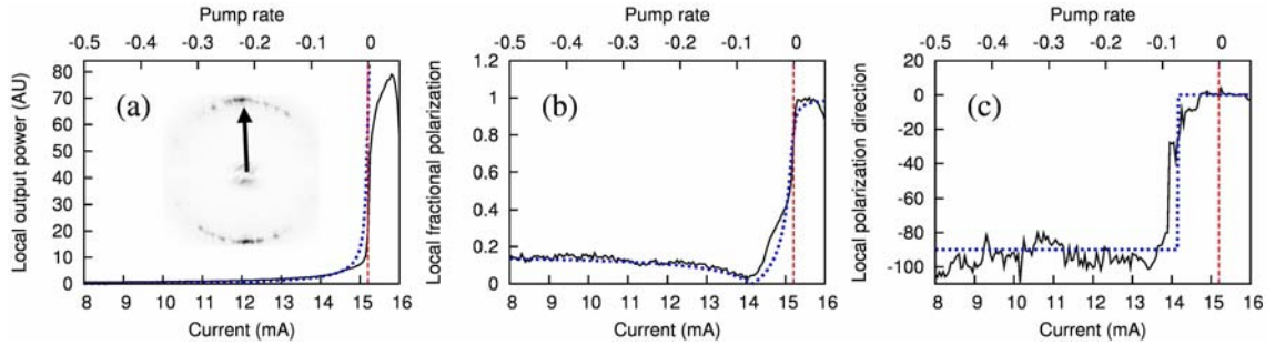
Figure 5: (Color online) Transition from spontaneous emission to lasing emission of the spot depicted in the inset in (a) for device #1. The black, solid curves are experimental data, the blue, dashed ones are calculated from Eqs. (9)-(12). (a) Local intensity in dependence on driving current. The threshold, indicated by the vertical red dashed line, is derived from a linear fit to the steep slope of the intensity. (b) Degree of polarization. (c) Local polarization direction. The change of polarization is evident about 1.5 mA below threshold.
