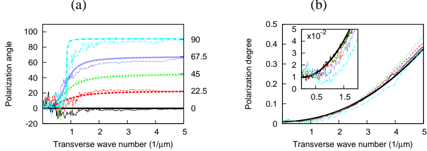
Figure 4: (Color online) Radial cuts (at 0^\circ (black solid line), 22.5^\circ (red long-dashed line), 45^\circ (green small-dashed line), 67.5^\circ (blue dotted line), and 90^\circ (cyan dot-dashed line)) through the far-field distribution of the spontaneous emission for device #1. T=0^\circ\text{C} , I=10\text{ mA} . (a) Polarization in dependence on the transverse wave number k_{\perp} showing the validity of the 0^\circ -rule for k_{\perp} > 2 \mu\text{m}^{-1} . The thick lines indicate the polarization expected from the theory developed in Sect. 4. (b) Fractional polarization in dependence on k_{\perp} for the same cuts as in (a). The part near k_{\perp} \approx 0 is shown in the inset.
