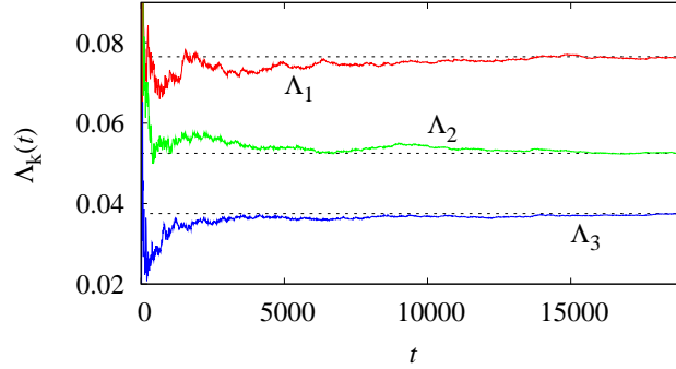
Figure 3: Stabilization of the leading three finite-time Lyapunov exponents calculated along chimera trajectories of increasing lengths. Parameters: N = 30 , R = 10 , and \alpha = 1.46 .
