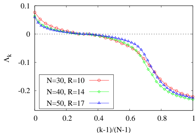
Figure 2: Lyapunov spectra computed for chimera trajectories of (1).
