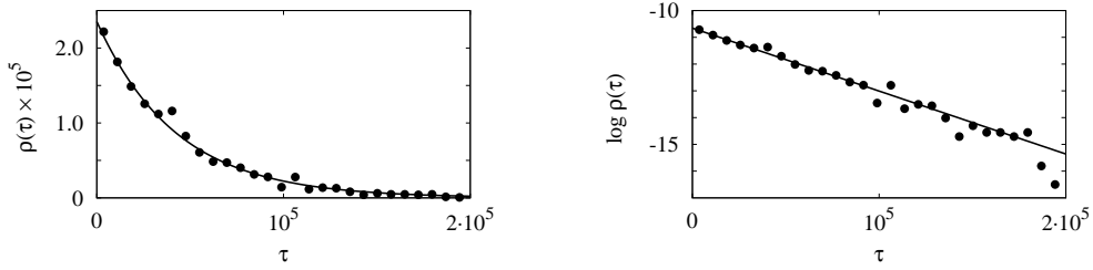
Figure 5: Histogram of collapse times (circles) in natural (left panel) and logarithmic (right panel) scale with fitted exponential distribution (solid line). Parameters as in Fig. 4.
