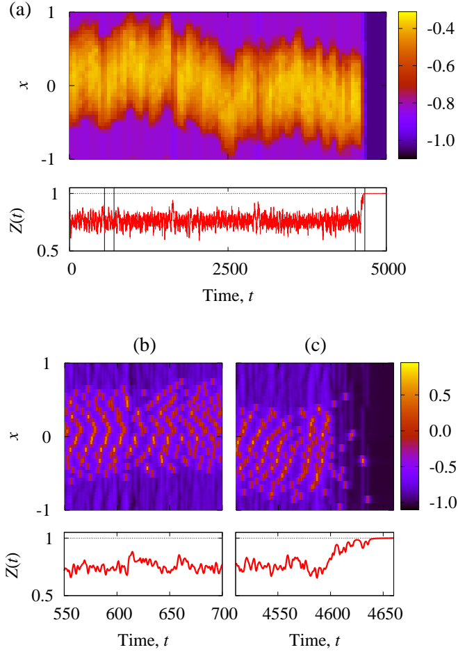
Figure 4: The chimera’s collapse: (a) space time plot of averaged phase velocities and global mean field Z(t) for a chimera trajectory that collapses after approx. 4600 time units to the completely coherent state (dark region: slow coherent motion). Panels (b) and (c) show a magnification of segments well before the collapse and directly at the collapse. Parameters: N = 40 , R = 14 , and \alpha = 1.46 .
