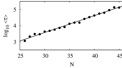
Figure 6: Average lifetimes of chimera states for increasing N from numerical simulations (circles); fitted exponential growth (solid line). Parameters: R/N \approx 0.35 , and \alpha = 1.46 .
