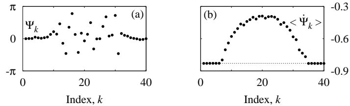
Figure 1: (a) Phase snapshot of a chimera state observed in system (1); (b) time-averaged frequencies. Parameters: N = 40 , R = 14 , and \alpha = 1.46 .
