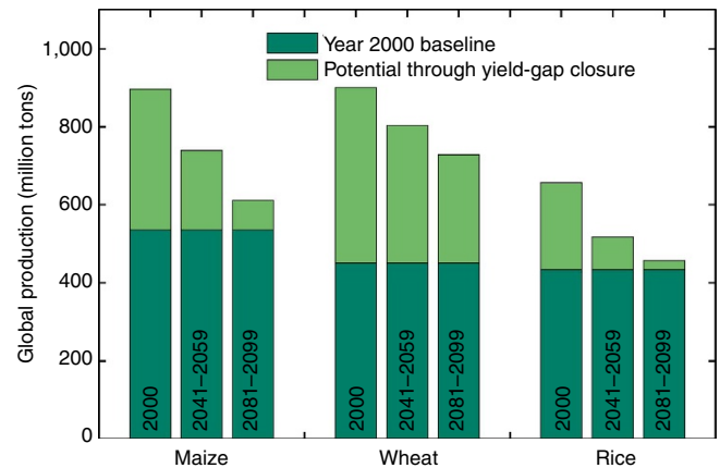
Figure 3 | The effect of climate change on production increases through agricultural intensification. The potential increases in global production of maize, wheat and rice that could be achieved by closing the yield gap (difference between actual and attainable yields) on current cropland are plotted for baseline, mid-century, and end-of-century climates (light green bars). For reference, these bars are imposed on top of actual production for ca. year 2000 (dark green bars), as calculated based on actual yields from Mueller et al. 4 and cropland area from Monfreda et al. 18 .
