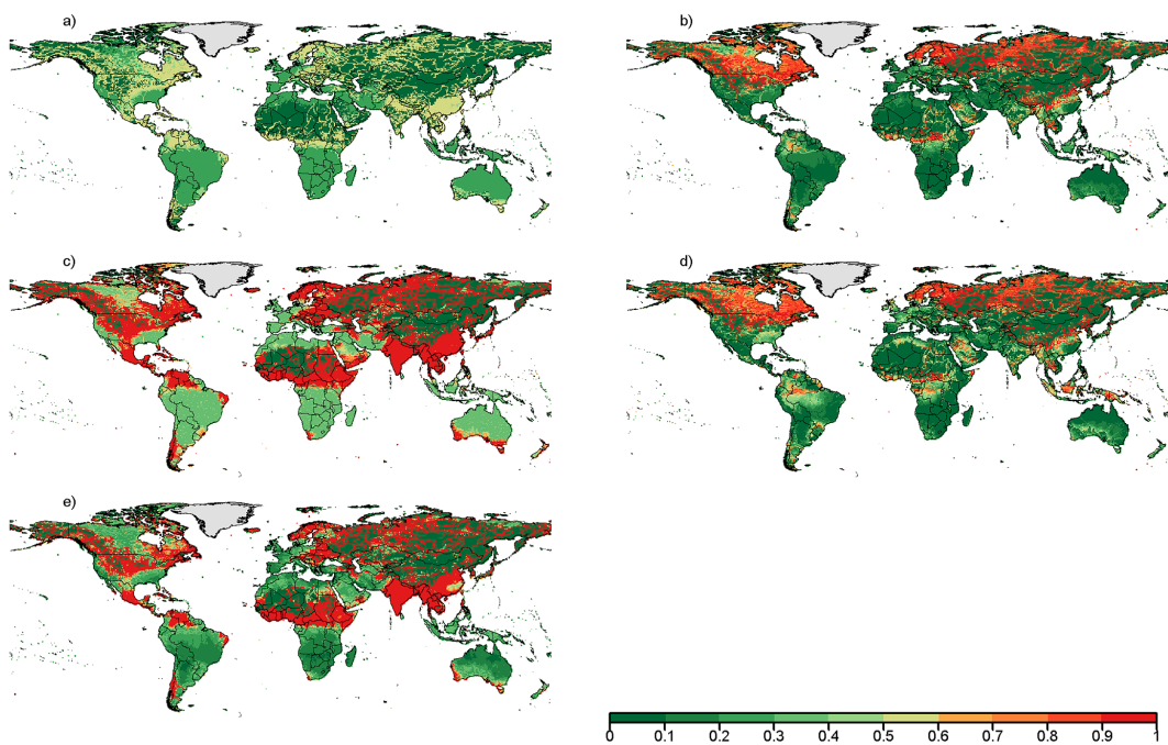
Figure 5. Ratios of monthly environmental flow to monthly actual flow (January) for the (a) variable monthly flow, (b) Smakhtin, (c) Tennant, (d) Q_{90}\text{-}Q_{50} , and (e) Tennant environmental flow methods.
