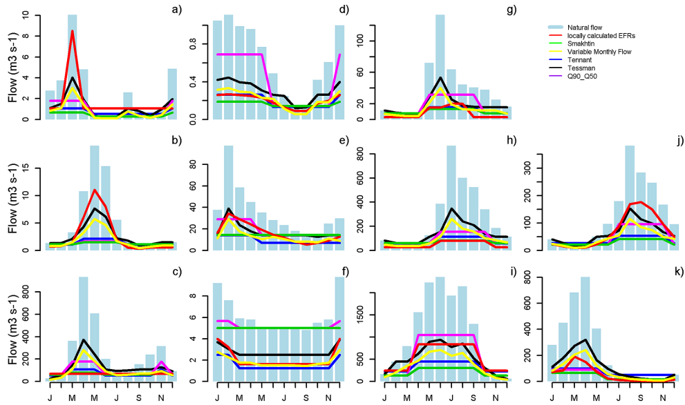
Figure 2. Comparison of EF methods with locally calculated EFRs in different case studies (a) Bill Williams River, USA, (b) Sharh Chai River, Iran (c) Ipswich River, US, (d) Silvan River, Spain, (e) Osborne Dam, Zimbabwe (f) Huasco River, Chile (g) Vojm Dam, Sweden, (h) Newhalen River, Alaska, (i) Hong Kong stream, China, (j) La Nga River, Vietnam, and (k) Great Ruaha River, Tanzania. Observed or simulated natural flows from the case studies are presented in light blue, except for the natural flows (c) and (e) which were simulated with LPJmL.
