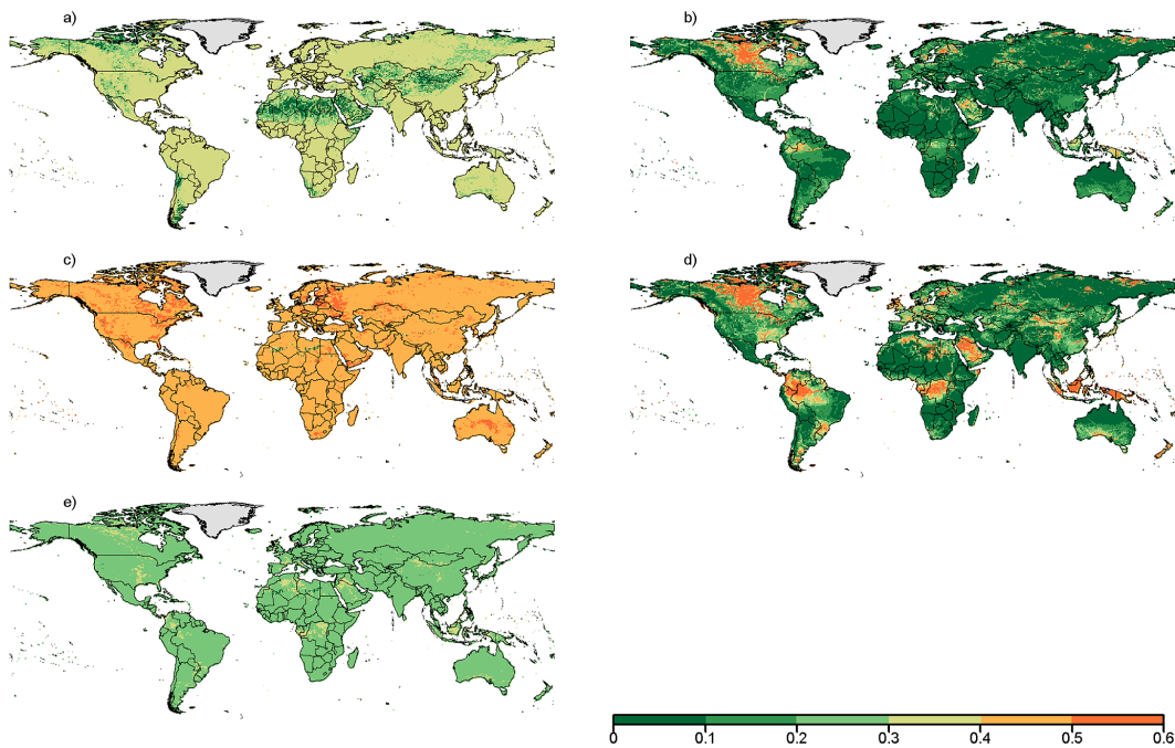
Figure 4. Ratios of annual environmental flow to annual natural flow calculated using the (a) variable monthly flow, (b) Smakhtin, (c) Tennant, (d) Q_{90}\text{-}Q_{50} , and (e) Tennant environmental flow methods.
