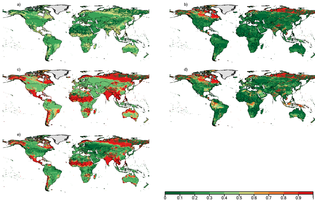
Figure 6. Ratios of monthly environmental flow to monthly actual flow (April) for the (a) variable monthly flow, (b) Smakhtin, (c) Tessmann, (d) Q_{90} – Q_{50} , and (e) Tennant environmental flow methods.
