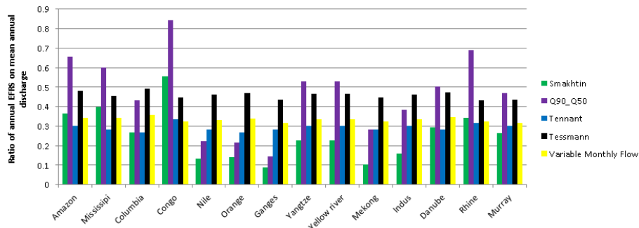
Figure 7. Comparison of the five environmental flow methods at the outlets of 14 river basins.
