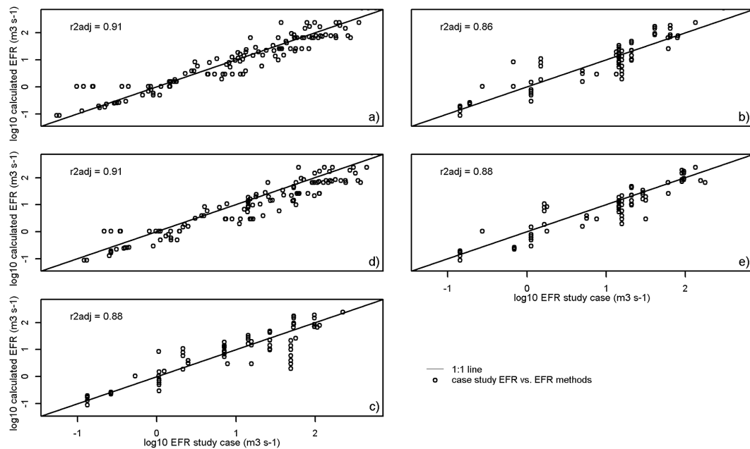
Figure 3. Relation between the monthly calculated EFRs and the locally calculated monthly EFRs of 11 case studies with the (a) variable monthly flow, (b) Smakhtin, (c) Tessmann, (d) Q_{90\_Q_{50}} , and (e) Tennant methods. In each subfigure, each dot represents EFRs for one month and for one case study.
