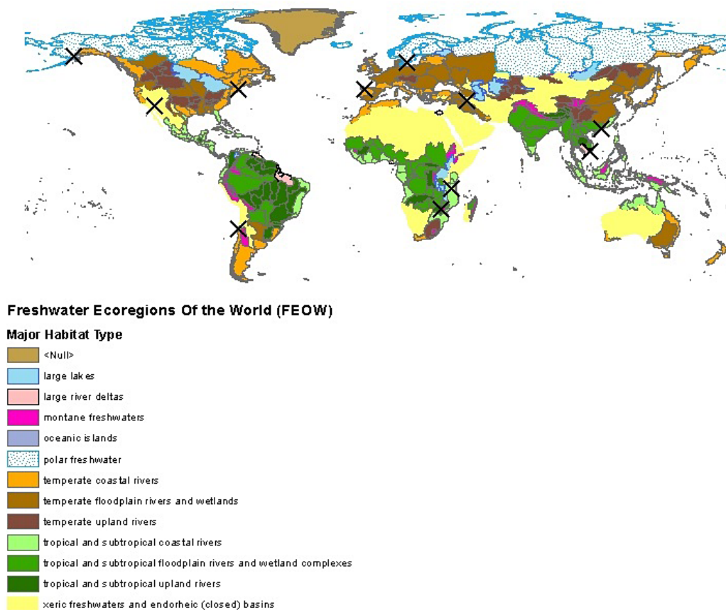
Figure 1. Locations of the 11 case studies where environmental flow requirements (EFRs) were locally defined.
