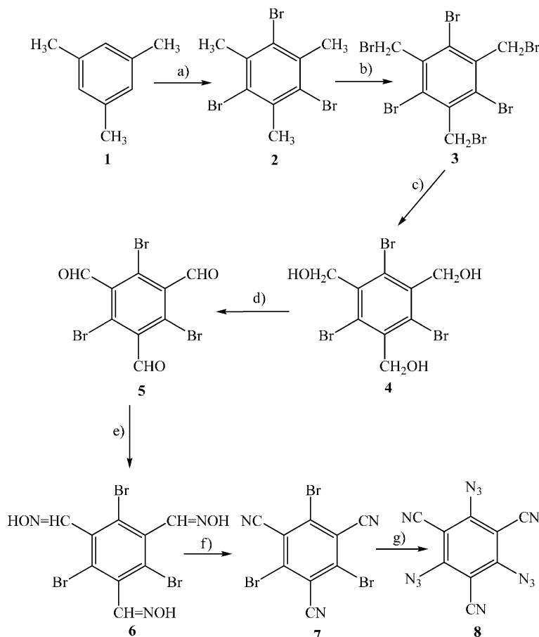
Scheme 1. Stepwise preparation of 1,3,5-triazido-2,4,6-tricyanobenzene. a) \text{Br}_2 , \text{AlBr}_3 , 0^\circ\text{C} \rightarrow 20^\circ\text{C} , 12 h; b) \text{Br}_2 , 1,2-dibromo-ethane, \Delta , 20 h; c) 1. \text{KOAc} , \text{DMF} , 80^\circ\text{C} , 20 h, 2. \text{KOH} , \text{H}_2\text{O} , 90^\circ\text{C} , 20 h; d) \text{NaOCl} , \text{KBr} , \text{TEMPO} (2,2,6,6-tetramethyl-piperidin-1-oxyl), \text{DCM} ( \text{CH}_2\text{Cl}_2 )/ \text{H}_2\text{O} , r. t., 3 d; e) \text{NaOAc} , \text{H}_2\text{N-OH}\cdot\text{H}_2\text{O} , \text{EtOH} , 60^\circ\text{C} , 2 h; f) \text{Ac}_2\text{O} , \Delta , 6 h; g) \text{NaN}_3 , \text{CH}_3\text{CN} , \Delta , 1 h.
