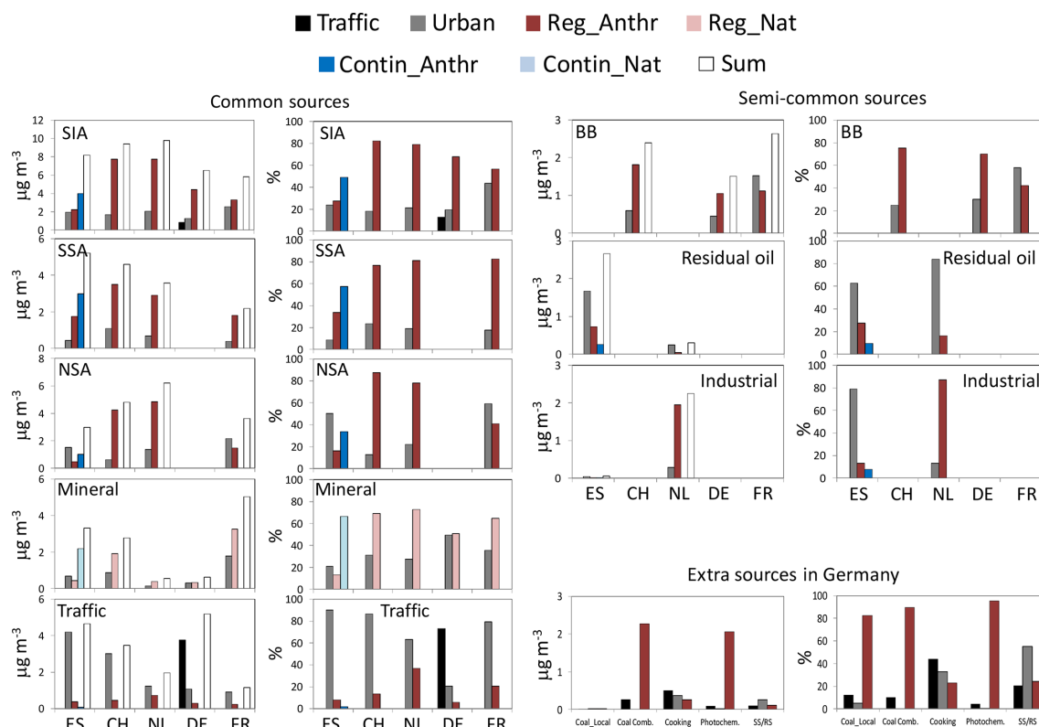
Figure 6. Lenschow's approach applied to the PM 10 (PM 2.5 in the Netherlands) PMF source contributions. Annual means are reported. ES: Spain; CH: Switzerland; NL: the Netherlands; DE: Germany; FR: France. In all countries, with the exception of Spain, Reg_Anthr and Reg_Nat are the sum of the regional and continental increments. Lenschow's approach applied to the PM 10 (PM 2.5 in the Netherlands) PMF source contributions. Annual means are reported. ES: Spain; CH: Switzerland; NL: the Netherlands; DE: Germany; FR: France. In all countries, with the exception of Spain, Reg_Anthr and Reg_Nat are the sum of the regional and continental increments.
