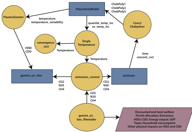
Fig. 3b. The exchange of variables between models in the bespoke framework generator (BFG2) for the PLASIM-ENTSem_GEMINI-E3 coupling. This diagram is generated automatically from the BFG2. The circles denote transformations, the rectangles denote models and the parallelogram denotes outputs from the model. Arrows indicate the direction of data flow within the coupling. Model names within these figures are slightly different from the text as they are program names for example: gemini_e3 is GEMINI-E3.
