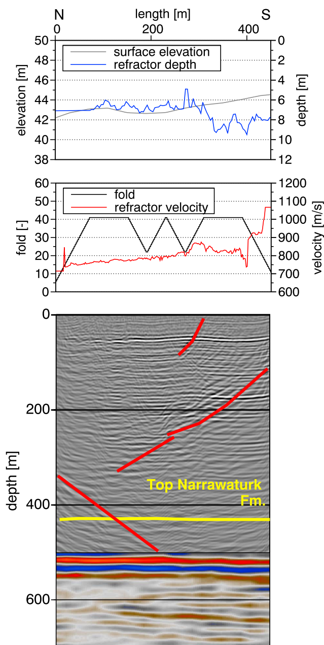
Figure 17. Detailed structure of PROFILE 3. (top) Surface elevation and refractor properties from the shear wave data. (bottom) Interpretation of the high-resolution shear wave image at sea level datum.
