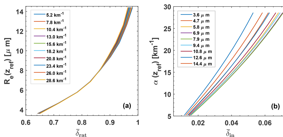
Figure 8. Two-step approach to derive R_e(z_{\text{ref}}) and \alpha(z_{\text{ref}}) from \bar{\delta}_{\text{rat}}(z_{\text{bot}}, z_{\text{ref}}) and \bar{\delta}_{\text{in}}(z_{\text{bot}}, z_{\text{ref}}) for a liquid cloud layer with z_{\text{bot}} = 3 km and z_{\text{ref}} = 3.075 km. In the first step (a), \bar{\delta}_{\text{rat}} is used to determine R_e(z_{\text{ref}}) by means of Eq. (26), and in the second step (b), \bar{\delta}_{\text{in}} and R_e (from step 1) are used to determine \alpha(z_{\text{ref}}) with Eq. (27). In (a), all simulations with all available combinations of R_e – \alpha profile pairs are shown to indicate the low impact of \alpha (given as numbers) on the retrieval. In (b), the relationship between \bar{\delta}_{\text{in}} and \alpha for nine R_e values (given as numbers) are shown to indicate the comparably large influence of R_e on the \alpha retrieval.
