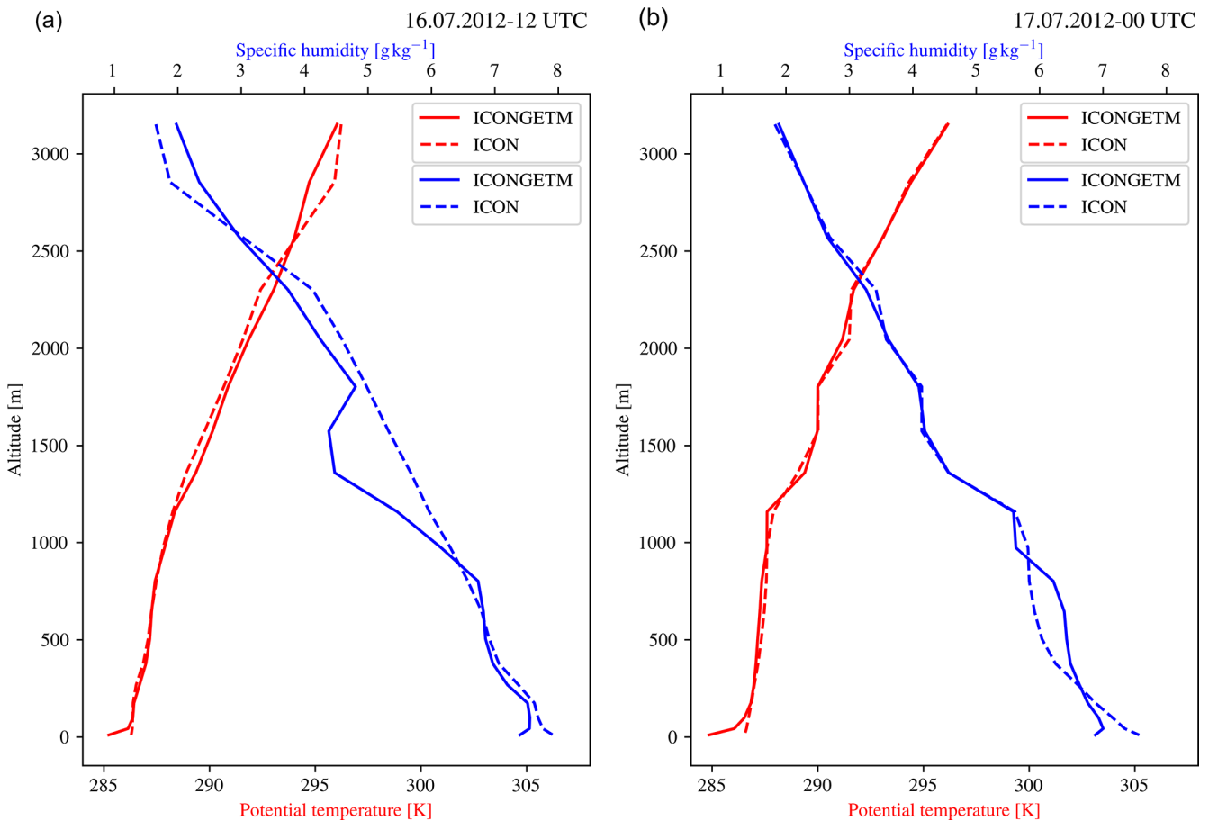
Figure 12. Atmospheric vertical profiles of potential temperature and specific humidity from the two-way coupled ICONGETM run and the uncoupled/one-way coupled ICON run for 16 (a) and 17 (b) July 2012 at 12:00 and 00:00 UTC, respectively. The profiles are obtained south-east of the island of Öland; see black star in Fig. 8.
