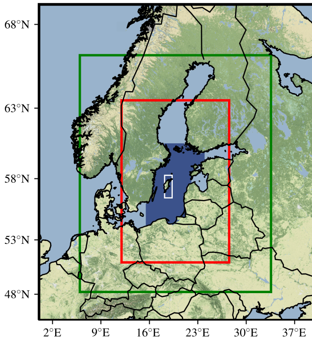
Figure 2. Nesting of different ICON domains with effective resolutions of 9.89 km (black frame), 4.93 km (green frame) and 2.47 km (red frame) over the Baltic Sea region. The dark-blue area in the central Baltic Sea represents the model domain of GETM. The white rectangle frames the area shown in Fig. 3.
