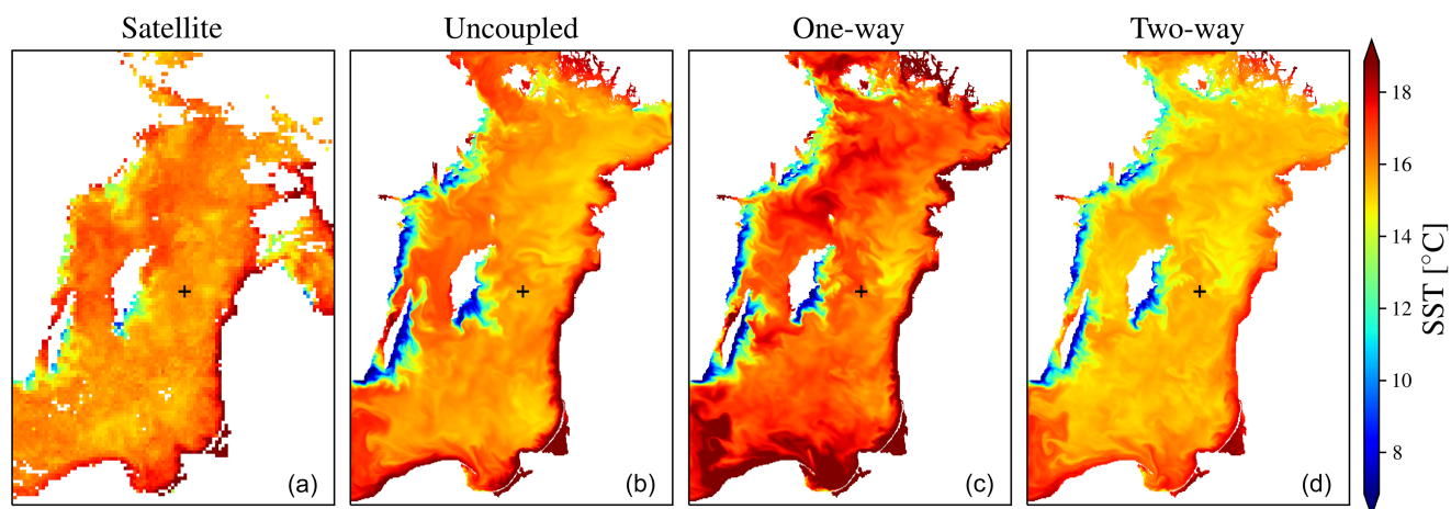
Figure 13. Daily mean sea surface temperature from satellites (a) and simulated by GETM in the uncoupled (b), one-way (c) and two-way (d) coupled simulation for 16 July 2012. The colour bar is identical to Fig. 7. The SST derived from satellite data was provided by the Federal Maritime and Hydrographic Agency of Germany (BSH). The black cross marks the position of station TF271 in the Eastern Gotland Basin.
