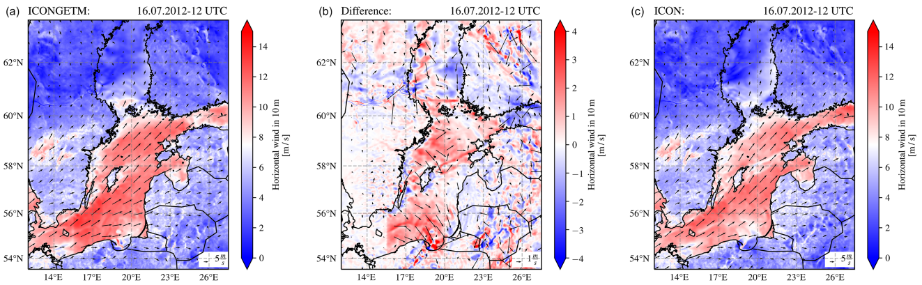
Figure 11. Horizontal wind field at 10 m height from the two-way coupled ICONGETM simulation (a) and the uncoupled/one-way coupled ICON simulation (c) as well as the difference ICONGETM minus ICON (b) for 16 July 2012 12:00 UTC. Displayed are the wind vectors (reference vector at the bottom of the figure, units of \text{m s}^{-1} ) and the wind speed (coloured).
