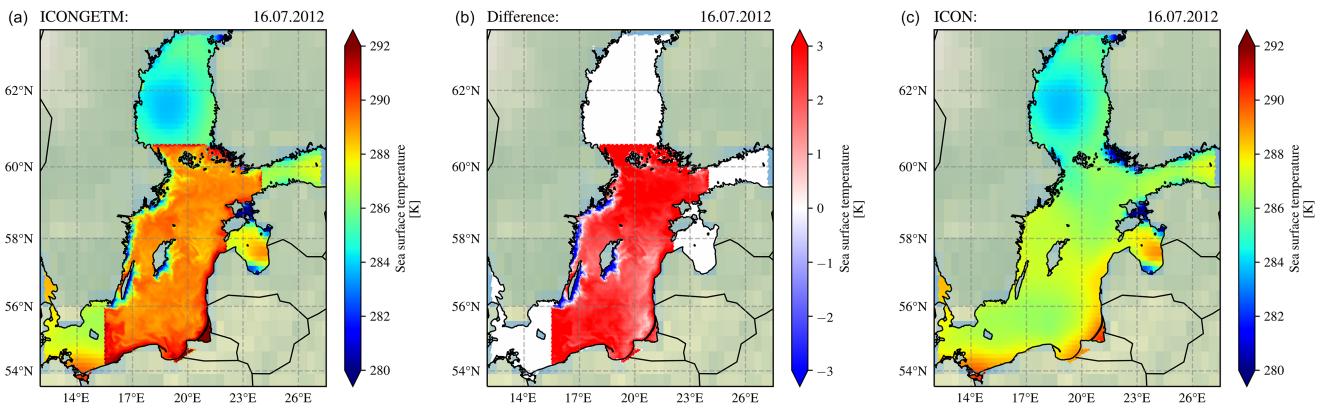
Figure 7. Daily mean sea surface temperature (SST) from the two-way coupled ICONGETM run (a) and the uncoupled/one-way coupled ICON run (c) as well as the difference ICONGETM minus ICON (b) for 16 July 2012. Outside the domain of simulated SST in the central Baltic Sea, the two-way coupled ICONGETM run also uses the prescribed ICON-internal SST.
