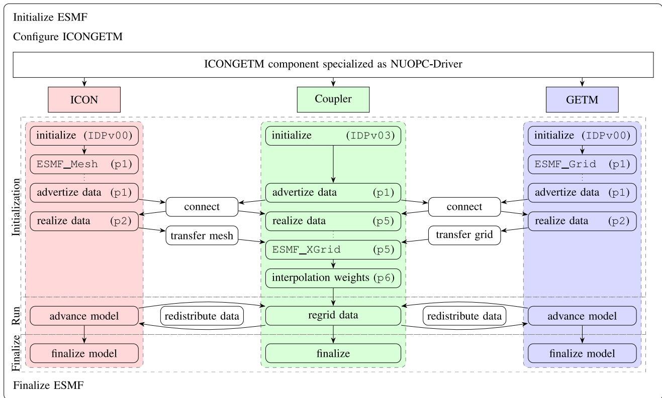
Figure 1. Structure of ICONGETM. The ICONGETM component created by the main program is specialized as NUOPC-Driver and consists of NUOPC-Model components for ICON and GETM as well as an NUOPC-Mediator for the Coupler. For all components the implemented specialized routines for initialization, run and finalization are indicated. The initialization phases of the NUOPC layer are given in parentheses. Automated generic NUOPC operations are represented by arrows. In the pdf version of this article the central NUOPC components presented in the figure are linked to the corresponding locations in the source code.
