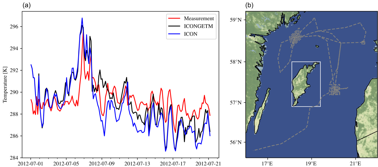
Figure 9. Air temperature at 29.1 m height in the central Baltic Sea over the period 1–21 July 2012 (a). Compared are model results from the two-way coupled ICONGETM and uncoupled/one-way coupled ICON simulations with measurements onboard the RV Meteor ; ship track shown in (b). The white frame shows the island of Gotland, similar to Fig. 2.
