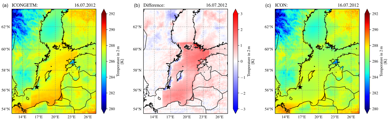
Figure 8. Daily mean 2 m air temperature from the two-way coupled ICONGETM simulation (a) and the uncoupled/one-way coupled ICON simulation (c) as well as the difference ICONGETM minus ICON (b) for 16 July 2012. The black star south-east of the island of Öland marks the position of the vertical profiles shown in Fig. 12.
