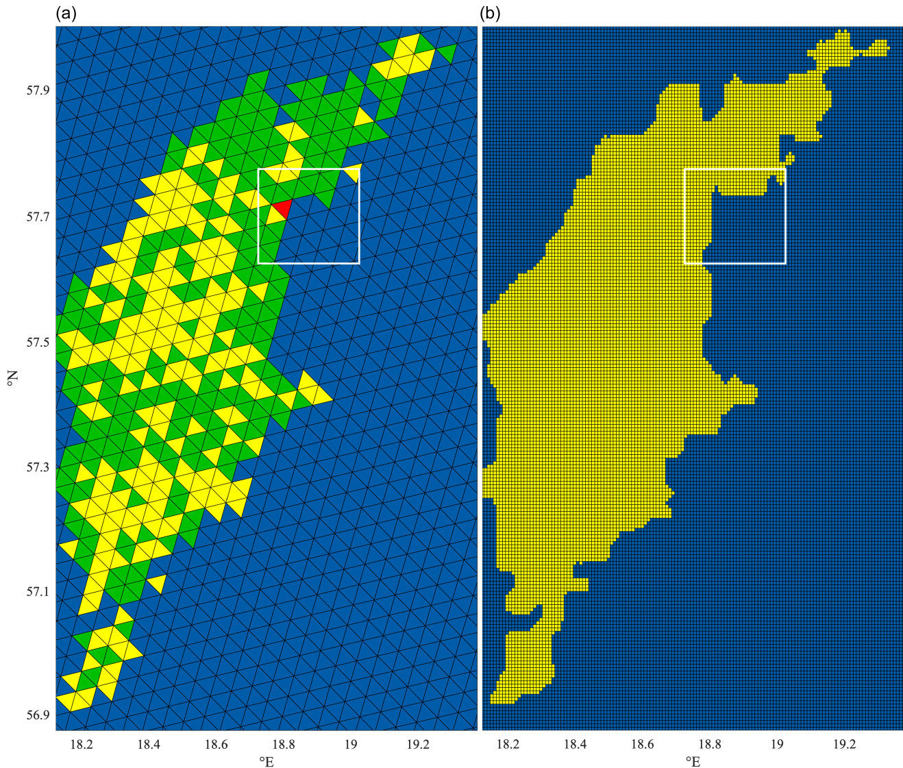
Figure 3. Triangular grid with an effective resolution of 2.47 km used in ICON (a) and rectangular grid with a resolution of approximately 600 m used in GETM (b) over the island of Gotland in the central Baltic Sea; see Fig. 2. In the ICON grid, the different colouring represents cells that consist of more than 50% of ocean (blue), forest (green), urban areas (red) or non-specific land classifications (yellow). GETM only distinguishes between ocean (blue) and land (yellow). The white rectangles frame the area shown in Fig. 4.
