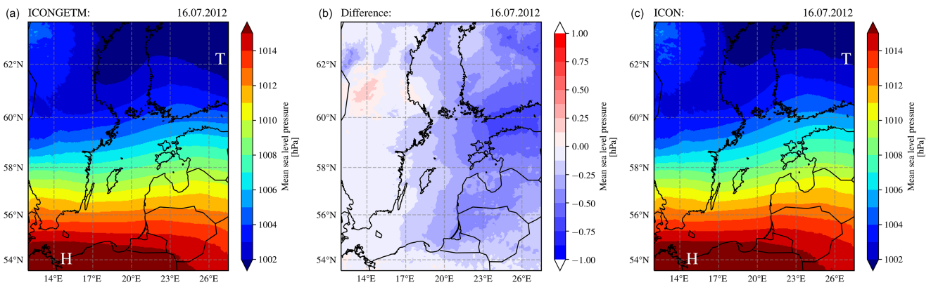
Figure 10. Daily mean sea level pressure from the two-way coupled ICONGETM simulation (a) and the uncoupled/one-way coupled ICON simulation (c) as well as the difference ICONGETM minus ICON (b) for 16 July 2012. “T” and “H” mark surface lows and highs, respectively.
