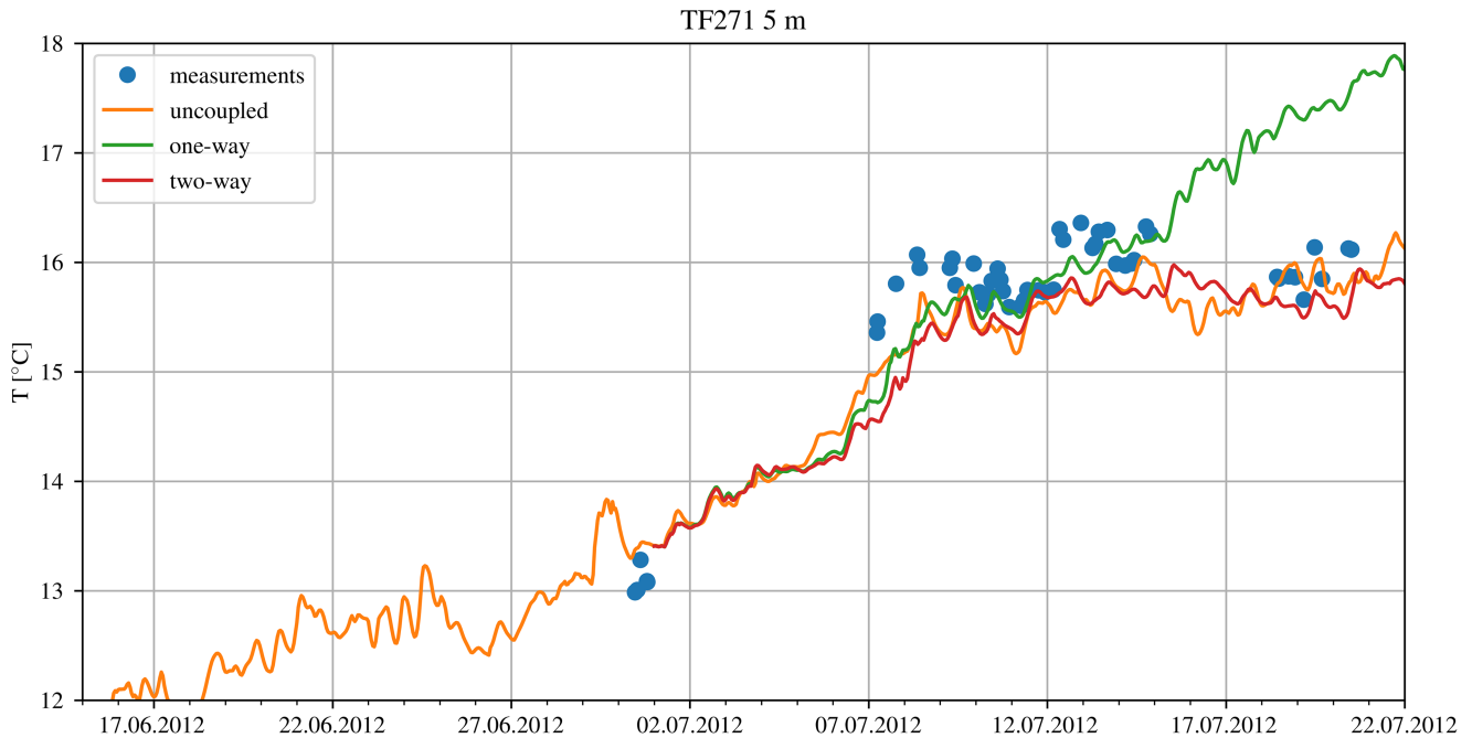
Figure 14. Temperature in 5 m depth at station TF271 (see black cross in Fig. 13) from CTD measurements and the three model simulations. The one- and two-way coupled simulations are started at 1 July 2012, after the uncoupled spin-up period.
