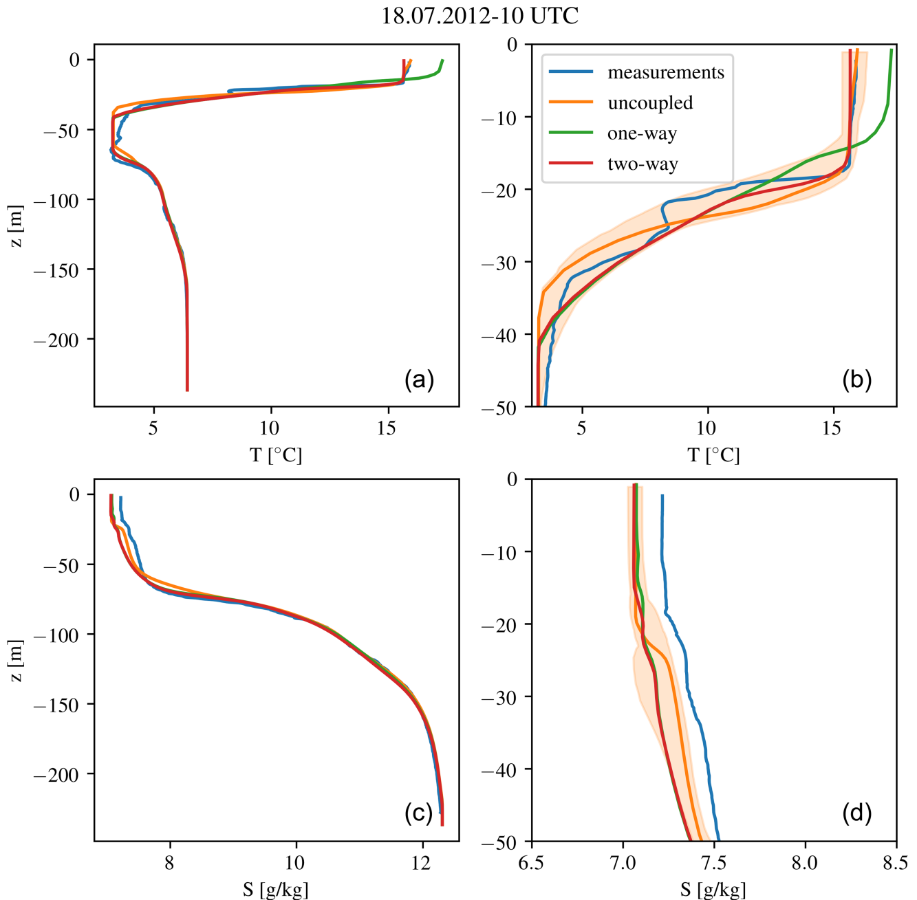
Figure 15. Temperature and salinity profiles at station TF271 from CTD measurements and the three model simulations. Panels (a) and (c) depict the whole water column; (b) and (d) are a zoom towards the sea surface. The light-orange-shaded area depicts the variability of the uncoupled simulation within an 8 d interval (14–21 July 2012).
