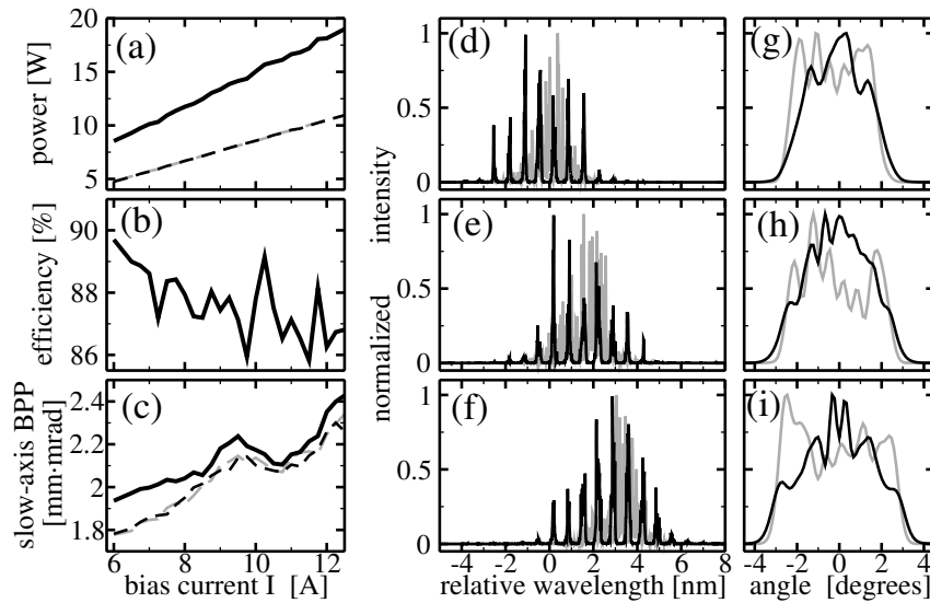
Figure 5: Power of the combined beam and the separate emissions (a), beam coupling efficiency (b), and slow-axis BPP factors of the beams (c) as functions of bias current applied at each of two emitters. Black solid: combined beam after the external mirror. Black and grey thin dashed: emission of BAL_1 and BAL_2 at corresponding front facet. (d), (g): optical spectra and angular representations of the combined beam after the external mirror (black) and of the solitary BAL without optical feedback (grey) for I = 6 A, that is applied to each emitter. (e), (h): same for I = 9 A. (f), (i): same for I = 12 A.
