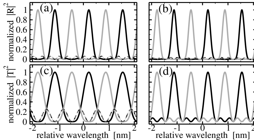
Figure 9: Normalized reflection (a,b) and transmission (c,d) spectra of the EC determined in Fig. 1 with an additional BC of the same length (a,c) or a twice longer BC and a PBS (b,d) just before the outcoupling mirror. Black and grey curves represent filtering of the fields emitted by BAL 1 and BAL 2 , respectively. Thick solid: self-feedback (a,b) and corresponding main transmission components (c,d). Thin dashed: cross-feedback (a,b) and the transmission of the BAL 1 (BAL 2 ) emission at the complimentary y - ( x -) polarized component, respectively (c). Parameters the same as in Fig. 3.
