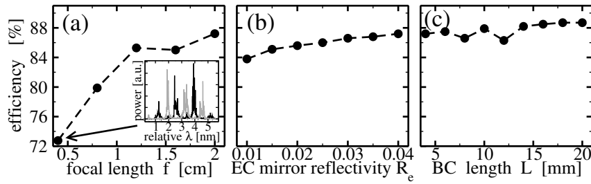
Figure 6: The efficiency of the beam combining as functions of the focal length of SAC lenses f for L = 4 mm, R_e = 0.04 (a), the EC mirror reflectivity R_e for L = 4 mm, f = 2 cm (b), and the BC length L for R_e = 0.04 , f = 2 cm (c). The inset in (a) shows optical spectra of BAL 1 (black) and BAL 2 (grey) for f = 4 mm.
