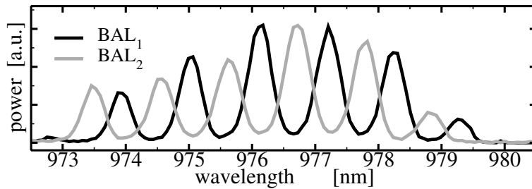
Figure 7: Optical spectra of the emission from separately activated BAL 1 and BAL 2 after the external mirror.
