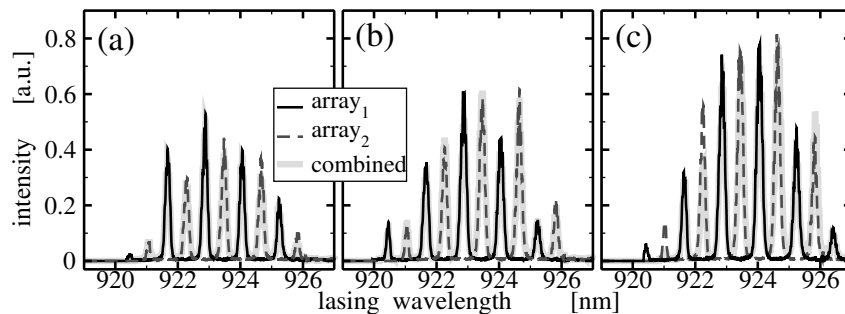
Figure 8: Optical spectra of the separately activated BAL arrays (thin black solid and dashed) and the combined beam (thick grey) for 100 A (a), 150 A (b), and 200 A (c) bias currents applied to each laser bar during 200 \mu s long intervals at 50 Hz repetition rate. Each array consists of 23 4 mm-long emitters having 200 \mu m wide contacts and 400 \mu m pitch width.
