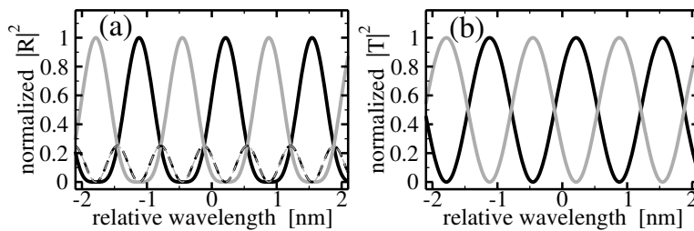
Figure 3: Normalized reflection (a) and transmission (b) spectra of the EC from Fig. 1. Black and grey: filtering of the fields emitted by BAL 1 and BAL 2 , respectively. Thick solid and thin dashed in (a): self- and cross- feedback.
