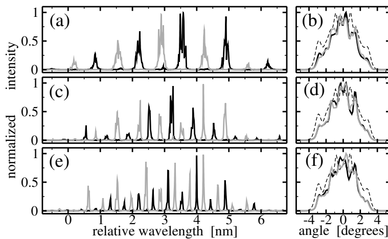
Figure 4: Dependence of the BAL emission on the length L of the BC within the EC. (a) and (b): L = 4 mm. (c) and (d): L = 8 mm. (e) and (f): L = 12 mm. In all cases f = 2 cm and R_e = 0.04 . Left and right panels: optical spectra and angular representations of the emissions. Solid black and grey: emission at the front facet of BAL_1 and BAL_2 , respectively. Thin dashed: combined beam after the external mirror.
