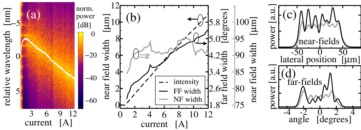
Figure 2: Simulations of the solitary BAL. Mapping of the optical spectra with an indication of the mean wavelength (a), mean emission intensity (dashed) and width (95 % of the power content) of the far (black solid) and near (grey solid) fields (b) as functions of the emitter current I , near (c) and far (d) fields for I = 8 A (grey) and I = 10 A (black).
