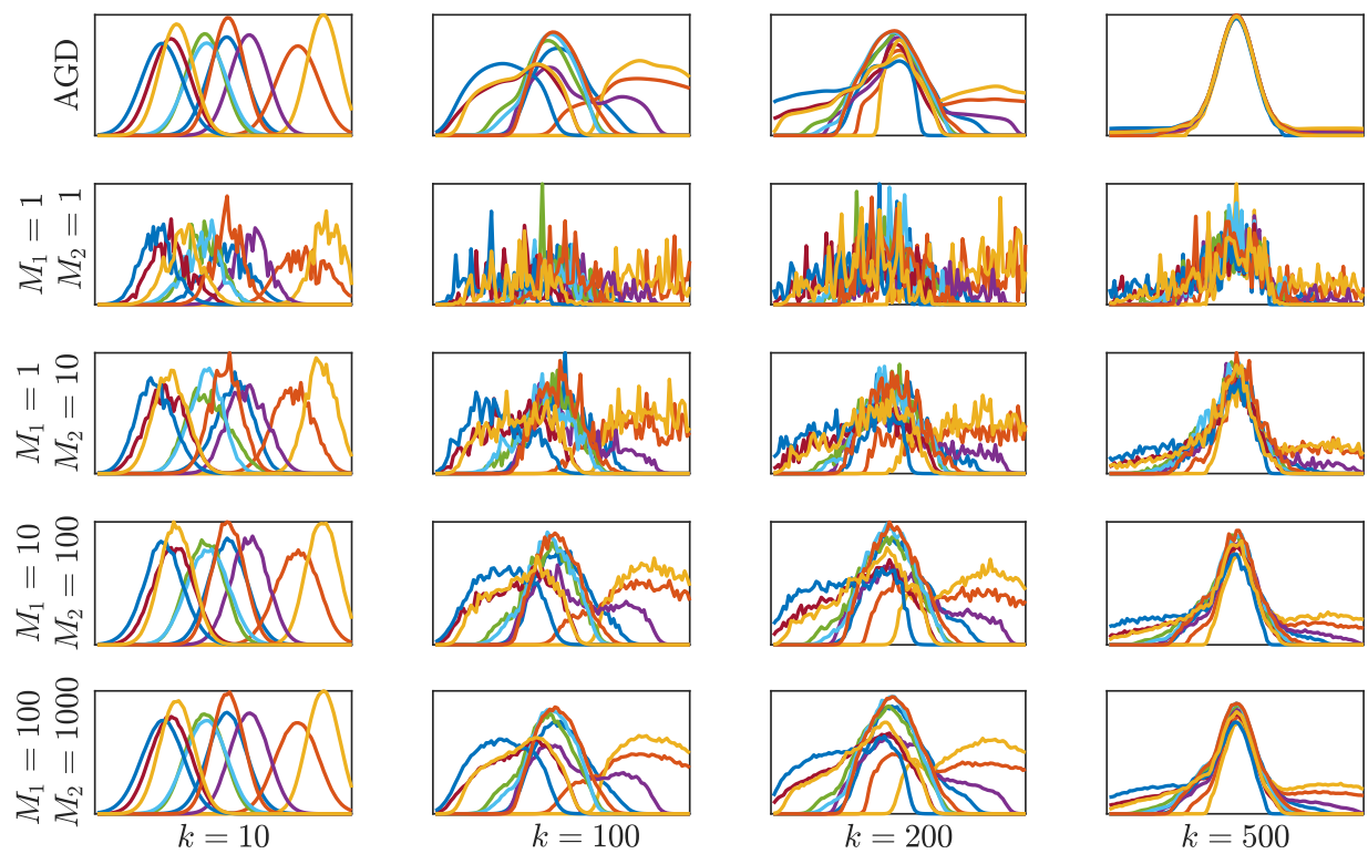
Figure 3: The iterates generated by Algorithm 2.
