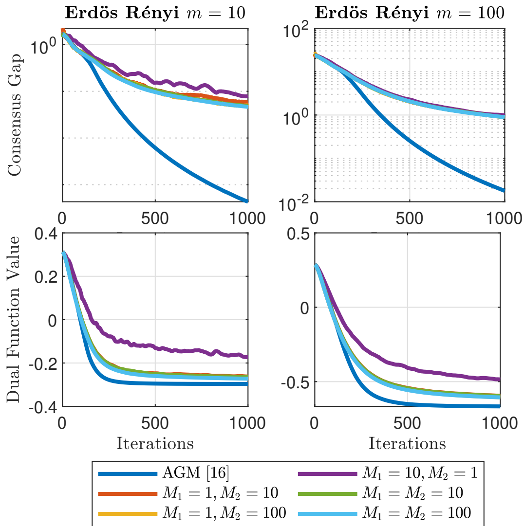
Figure 2: Consensus gap and dual function values generated by Algorithm 2.
