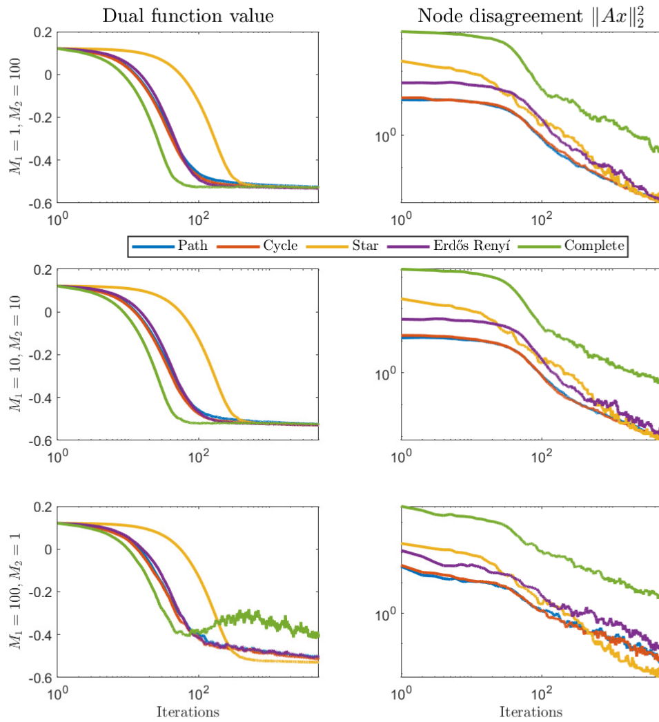
Figure 5: The dual function value and node disagreement of the iterates generated by Algorithm 2 on five different graphs, namely: path, cycle, star, Erdős-Renyí, and complete graphs, with 30 nodes each. Moreover, we show the effects of different number of samples per iterations. For each network, we test M_1 = 1 and M_2 = 100 , M_1 = 10 and M_2 = 10 , and M_1 = 100 and M_2 = 1 .
