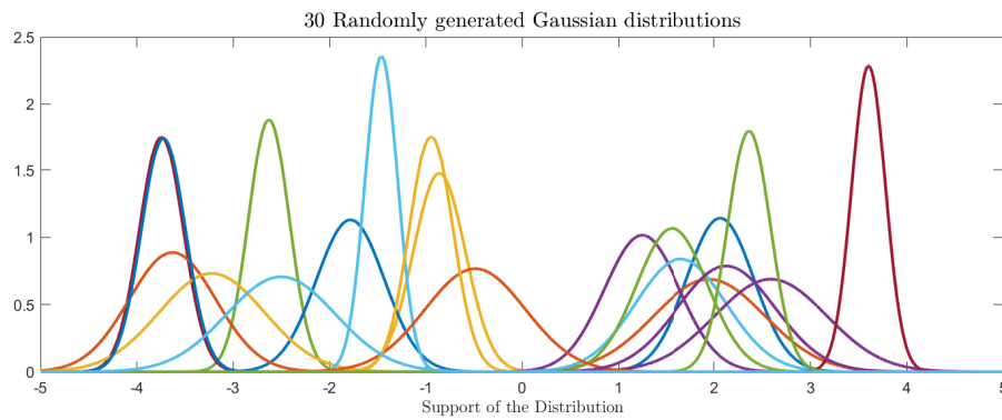
Figure 4: The randomly generated Gaussian distributions. Each distribution is assigned to each agent.
