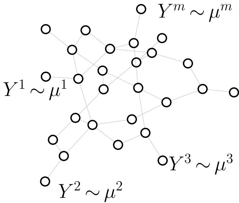
Figure 1: A network of agents, where each agent is able to sample from a different distribution, i.e., agent i \in V samples from \mu^i .
