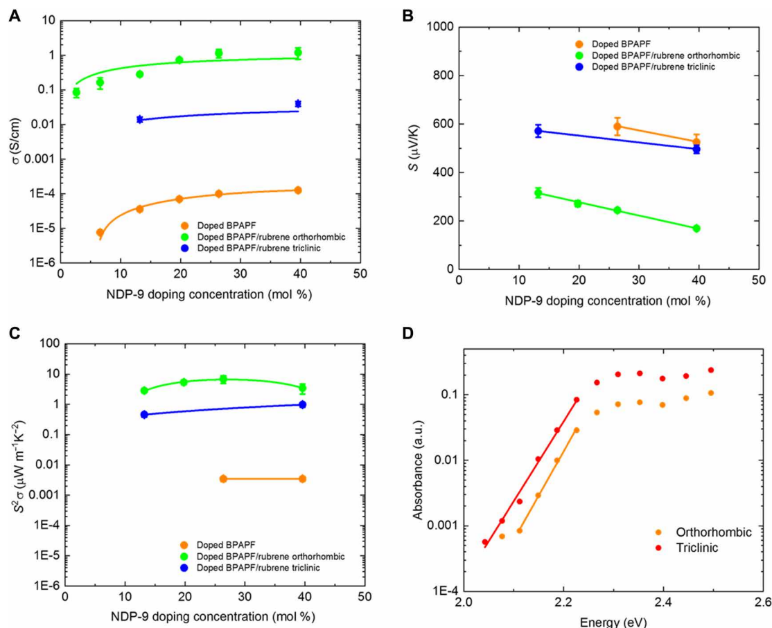
Fig. 2. Thermoelectric and photothermal deflectivity measurements of modulation-doped rubrene crystalline thin films. (A to C) Conductivity, Seebeck coefficient, and thermoelectric power factor dependence on the doping concentration. The conductivity and Seebeck coefficients were taken at 30°C. The blue, green, and orange solid lines are guides for the eye. (D) Photothermal deflection spectroscopy of triclinic ( U_e = 82 \pm 4 meV) and orthorhombic platelet ( U_e = 74 \pm 3 meV) rubrene crystalline thin films. The straight lines are fits of the Urbach tails. a.u., arbitrary units.
