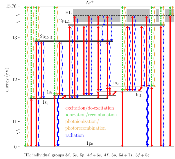
Figure 1. Argon kinetic scheme used in the model.
