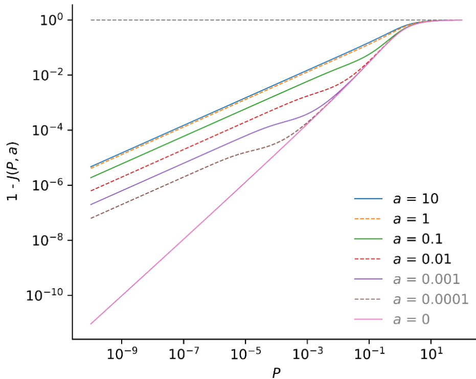
Figure 1. Dependence of the expression (1 - J(P, a)) , where J is given by Equation (16) on the variable P for various values of a which is the Lorentz-to-Doppler width ratio in the Voigt spectral line shape.
