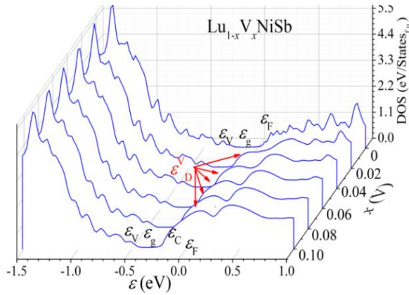
Fig. 4. Modeling the distribution of the density of electronic states DOS of \text{Lu}_{1-x}\text{V}_x\text{NiSb} in the absence of magnetic ordering.
