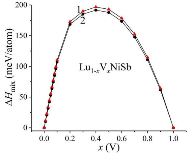
Fig. 1. Modeling of changes in the values of the mixing enthalpy \Delta H_{\text{mix}} of \text{Lu}_{1-x}\text{V}_x\text{NiSb} in the presence of (1) and the absence (2) of a magnetic moment on V atoms.
