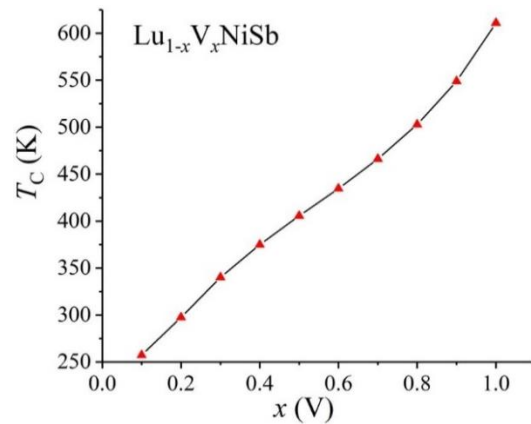
Fig. 5. Modeling of changes in the Curie temperature T_C values of the \text{Lu}_{1-x}\text{V}_x\text{NiSb} in the presence of magnetic ordering.
