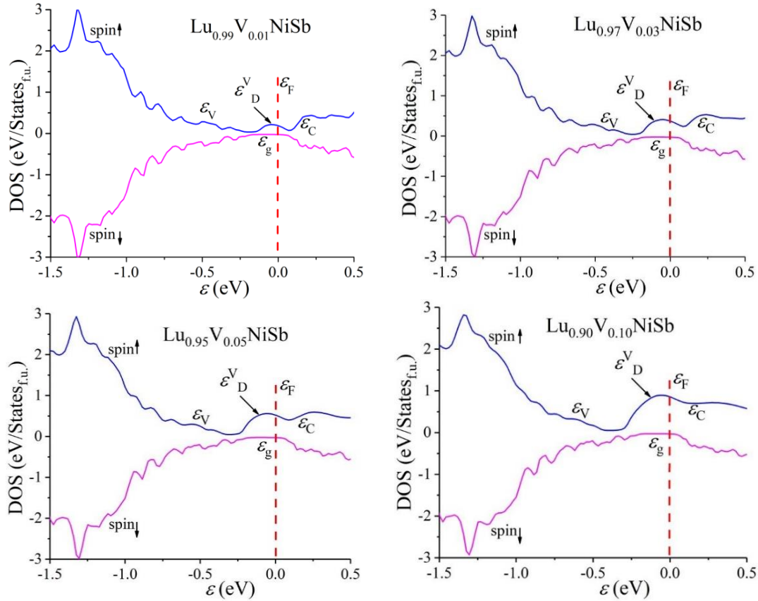
Fig. 3. Modeling of the distribution of the density of electronic states DOS of \text{Lu}_{1-x}\text{V}_x\text{NiSb} when available magnetic ordering.
