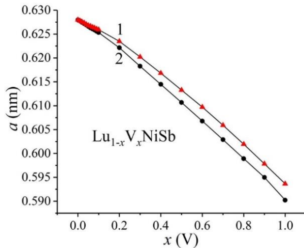
Fig. 2. Modeling of changes in the values of the unit cell parameter a(x) of \text{Lu}_{1-x}\text{V}_x\text{NiSb} in the presence (1) and absence (2) of the magnetic moment on V atoms.
