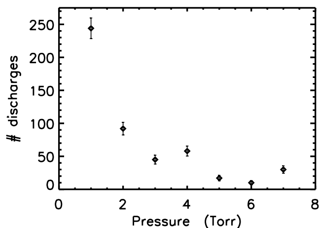
Figure 6. Number of discharges observed as a function of pressure for the vertical drop apparatus; 200 individual dust drops were made for each of the pressures shown. As with the horizontal mixing apparatus, the number of discharges decreases with increasing pressure.
