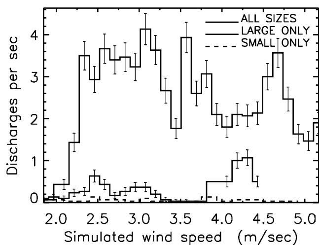
Figure 4. Discharge rate from the horizontal mixing apparatus as a function of wind speed for three particle-size distributions. A significant number of discharges occur only when there is a mixture of particle sizes. While the discharge rates presented here are for a pressure of 8 Torr, similar results are obtained at other pressures.
