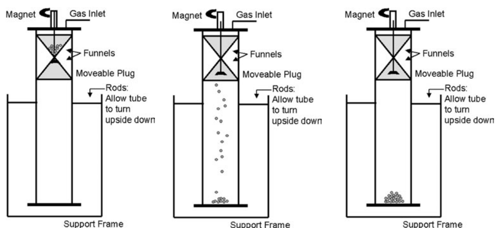
Figure 2. Schematic diagram of the vertical drop apparatus. Three time steps are shown to demonstrate the vertical fall of the dust. The glass tube flips upside down to reset the experiment.
