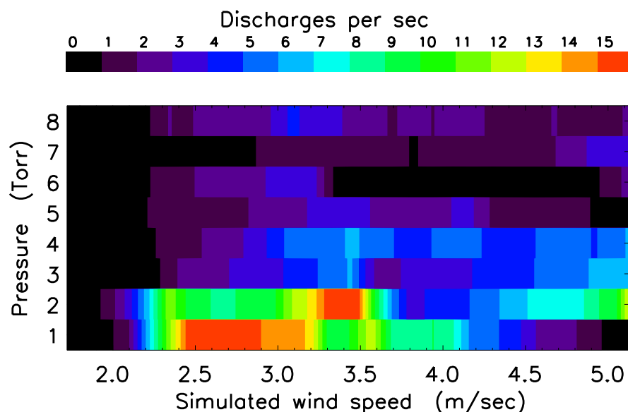
Figure 3. Discharge rates from the horizontal mixing apparatus as a function of pressure and simulated wind speed. The key above the plot denotes the colours representing different discharge rates.
