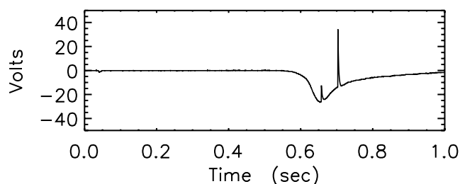
Figure 5. A typical voltage reading for a single dust drop in the vertical drop apparatus for a pressure of 4 Torr. The broad negative dip is a signature of the charged dust hitting the bottom of the experiment. The larger, negatively charged JSC-Mars-1 particles begin arriving at the bottom of the chamber after \approx 0.55 s, and the lighter, positively charged glass microballoons approach the bottom of the chamber \approx 0.1 s later. The narrow spikes represent electrical discharges.
