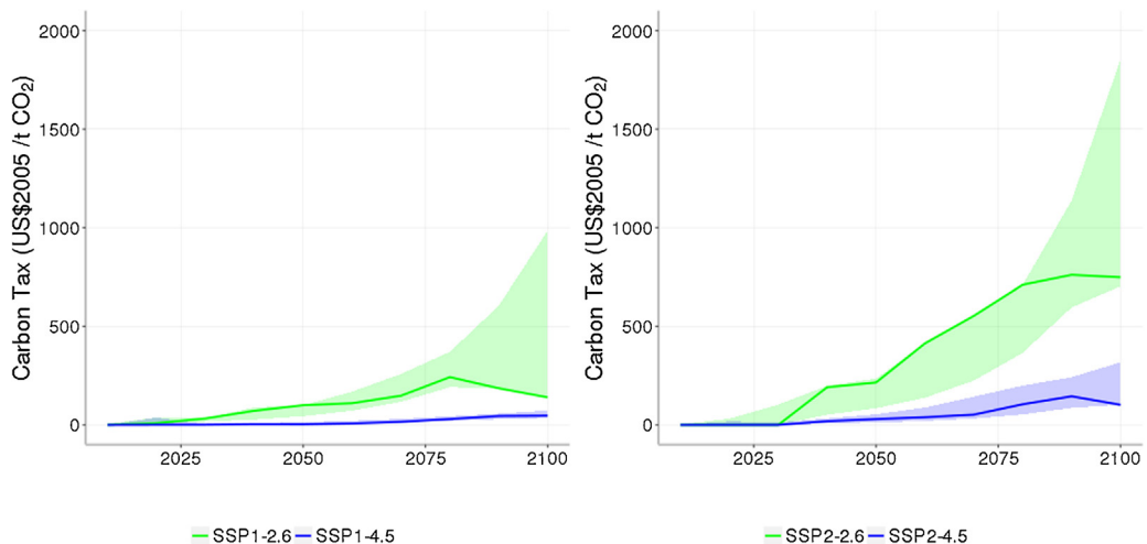
Fig. 12. Carbon price for reaching radiative forcing targets of 4.5 and 2.6 W/m 2 for SSP1 (left) and SSP2 (right). The area indicate the range of results of the other IAM scenarios for the specific SSP (see references in Section 2).
