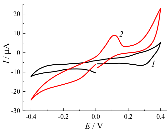
Figure 12. CV curves obtained at 20 mV/s from SPE/TiO 2 modified by 3 \mu L CuI-PPy (drop coating) in buffer (1) and 250 ppm of glutaraldehyde (GLU) solution (2) at pH 8.
