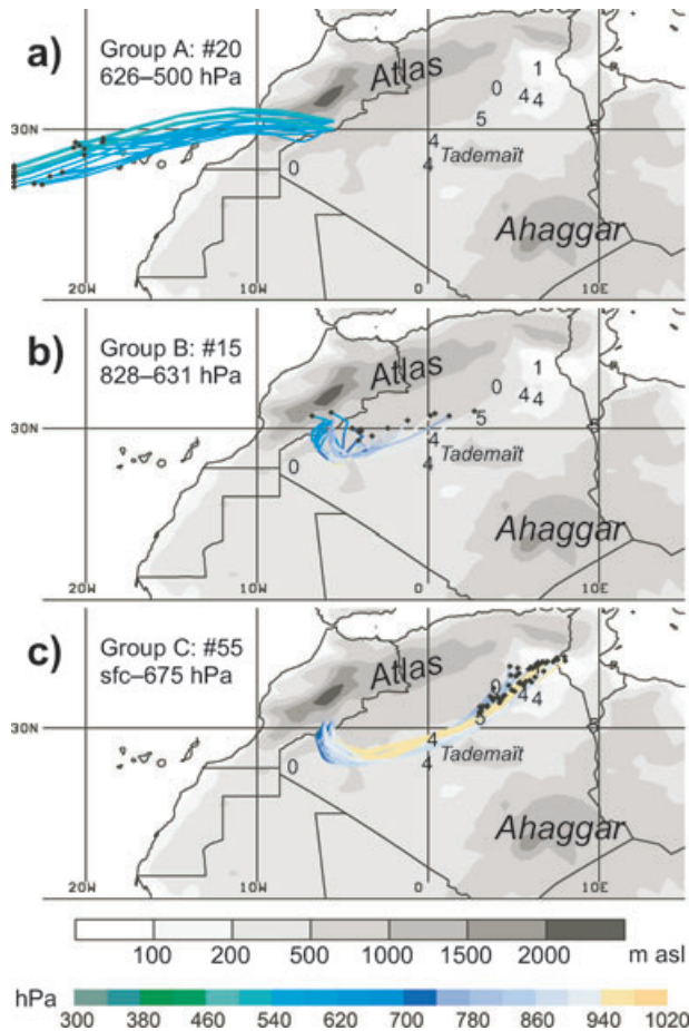
Fig. 7. Case I: Two-day backward trajectories started from the 3-D box 30.0°N–30.5°N, 6.0°W–5.5°W, surface–500 hPa at 1200 UTC 3 June 2006. The 90 trajectories were subjectively assigned to three groups with similar behaviour. The trajectories are colour-coded with pressure (in hPa) according to the legend at the bottom. Trajectory origins are marked with black circles. Grey shading indicates the elevation of the ECMWF topography at 0.5° horizontal resolution. The number of reports of 'dust or sand raised by the wind' at synoptic stations near the trajectory tracks during the first day (eight synoptic hours from 1200 UTC 1 June to 0900 UTC 2 June 2006) are given as numbers. For information on the used stations, see Table 1.
