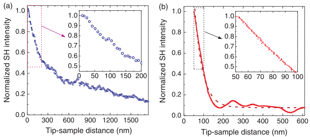
Figure 17. SH approach curves in (a) the non-modulated case and (b) with tip/sample distance demodulation.
