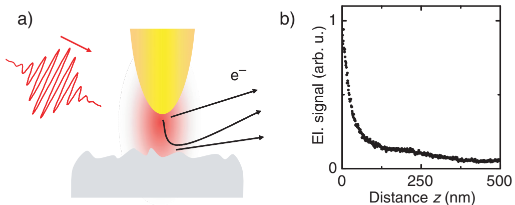
Figure 25. (a) Concept of the tip-enhanced electron emission microscope, indicating possible contrast mechanisms due to (i) a modification of the electron yield from the tip, (ii) local electron emission from the sample induced by the enhanced fields near the tip end, (iii) single or multiple scattering of electrons at the tip and/or the sample. (b) Dependence of the electron signal on the tip-to-sample distance z when approaching a gold surface.
