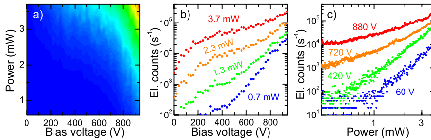
Figure 22. (a) Power- and voltage-dependent electron emission. (b) Voltage dependent curves at four different incident powers. (c) Power-dependent curves at four different bias voltages.
