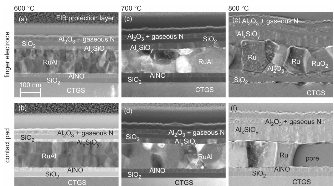
Figure 4. STEM images (predominant orientation contrast) of a finger electrode (upper row) and the contact pad (lower row) after annealing at (a,b) 600 °C, (c,d) 700 °C, and (e,f) 800 °C (192 h).
