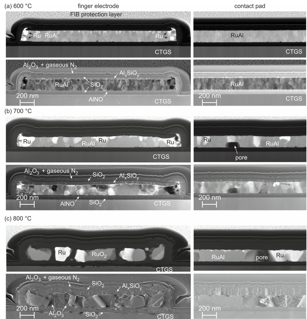
Figure 3. STEM images of a finger electrode and of the contact pad after annealing at (a) 600 °C, (b) 700 °C, and (c) 800 °C (192 h). Upper row: image with predominant element contrast; lower row: image with predominant orientation contrast.
