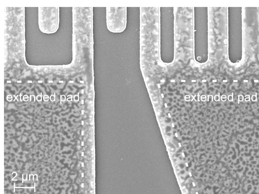
Figure 5. SEM image of the sample annealed at 800 °C for 192 h. The white dashed line serves as a guide to the eye for the transition of the strongly oxidized edge of the extended pads and the less degraded inner region.
