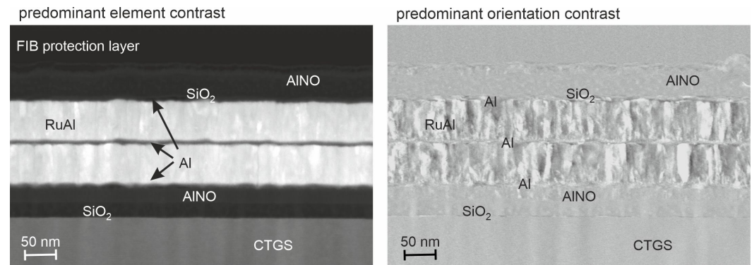
Figure 1. STEM images of a cross-section of the as-prepared electrodes with predominant element (left) and orientation (right) contrast, respectively.
