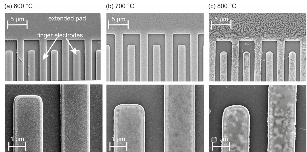
Figure 2. SEM images (20 kV, InLens) of parts of the narrow finger electrodes and extended pad with two different magnifications after annealing at (a) 600 °C, (b) 700 °C, and (c) 800 °C (192 h, air).
