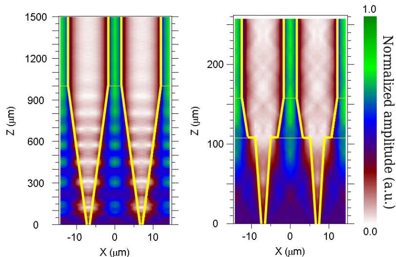
Figure 6. Illustration of simulated coupling between the free propagation regions (FPR) and the waveguide array with standard linear tapers (left) and discontinuous MMI tapers (right). The beating pattern in the left image indicates two-mode interference. Waveguide core boundaries are highlighted in yellow colour.
