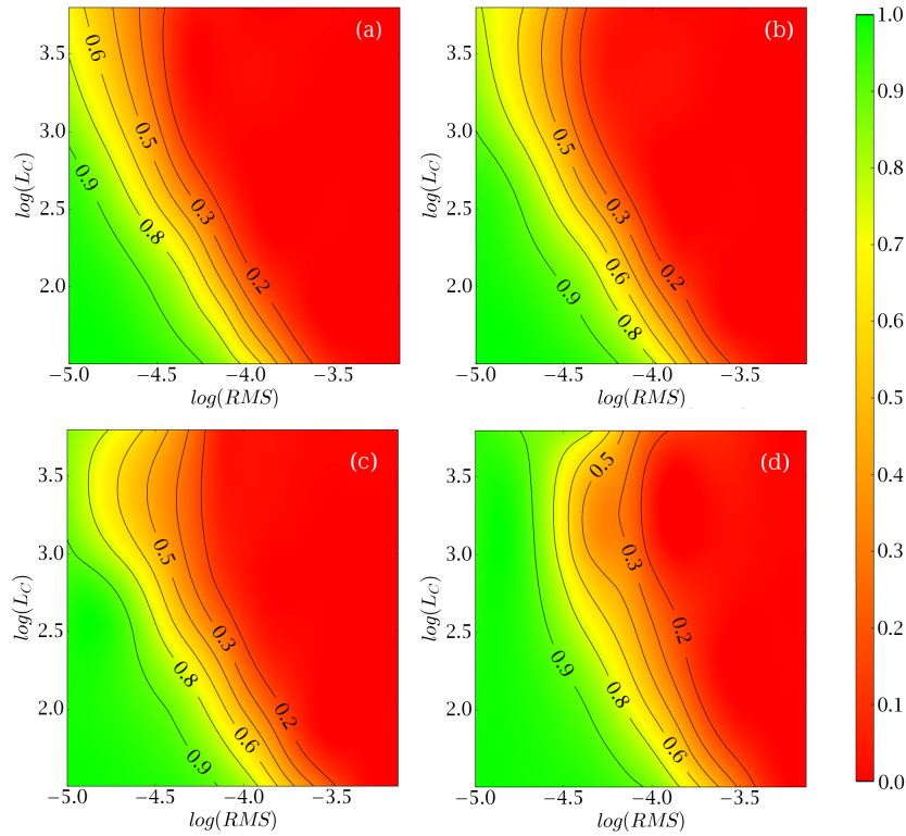
Figure 10. Figure of merit (FOM) maps for waveguide arrays of various sizes and propagation lengths. 800 waveguides, L = 10.5 cm (a); 600 waveguides, L = 8.3 cm (b); 400 waveguides, L = 6 cm (c); 200 waveguides, L = 3.8 cm (d).
