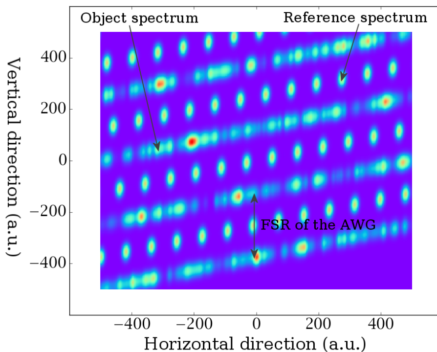
Figure 2. Artificial example of a cross-dispersed AWG main spectrum with an interleaved reference.
