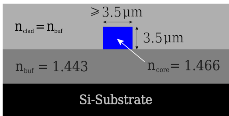
Figure 3. Cross-section of the rectangular buried channel waveguide core used in the AWG design. Core thickness is 3.5 \mu\text{m} with variable core widths of 3.5 \mu\text{m} (arrayed waveguides)— 16.03 \mu\text{m} (widest taper).
