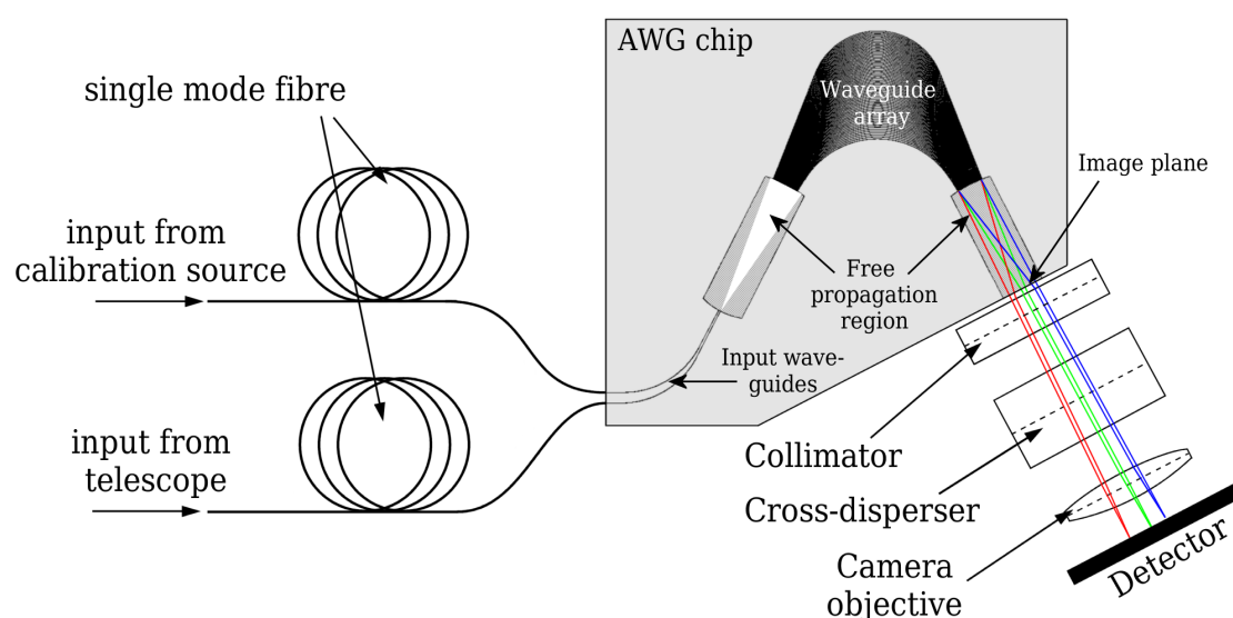
Figure 1. Schematic depiction of an arrayed-waveguide-grating (AWG)-based spectrograph assembly with cross-dispersive optics.
