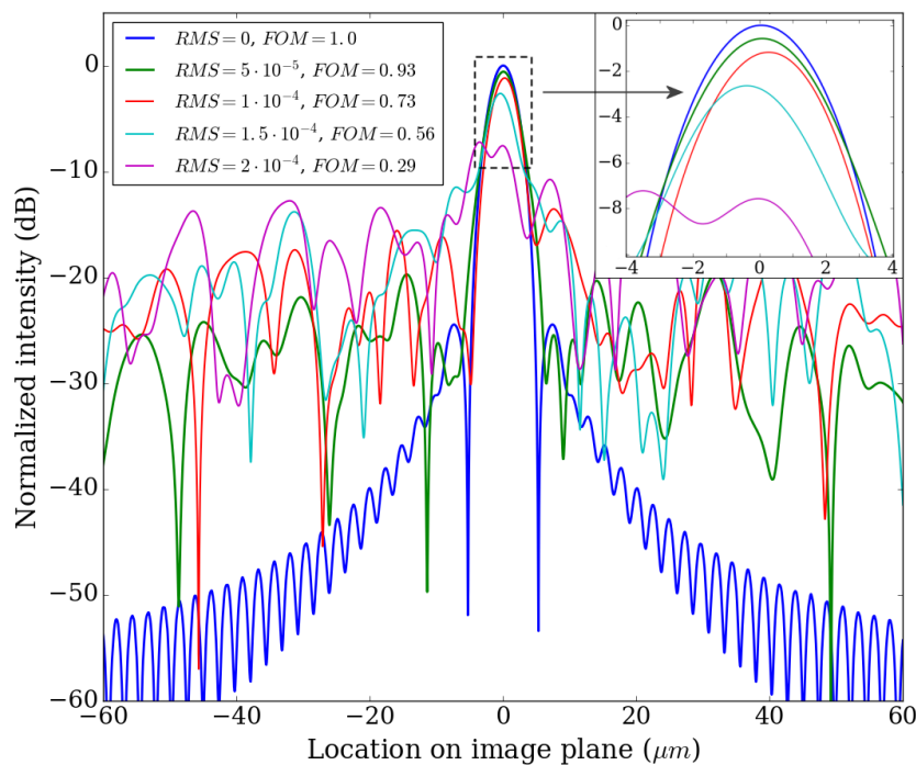
Figure 8. Optical field amplitude at the AWG output facet for various RMS values.
