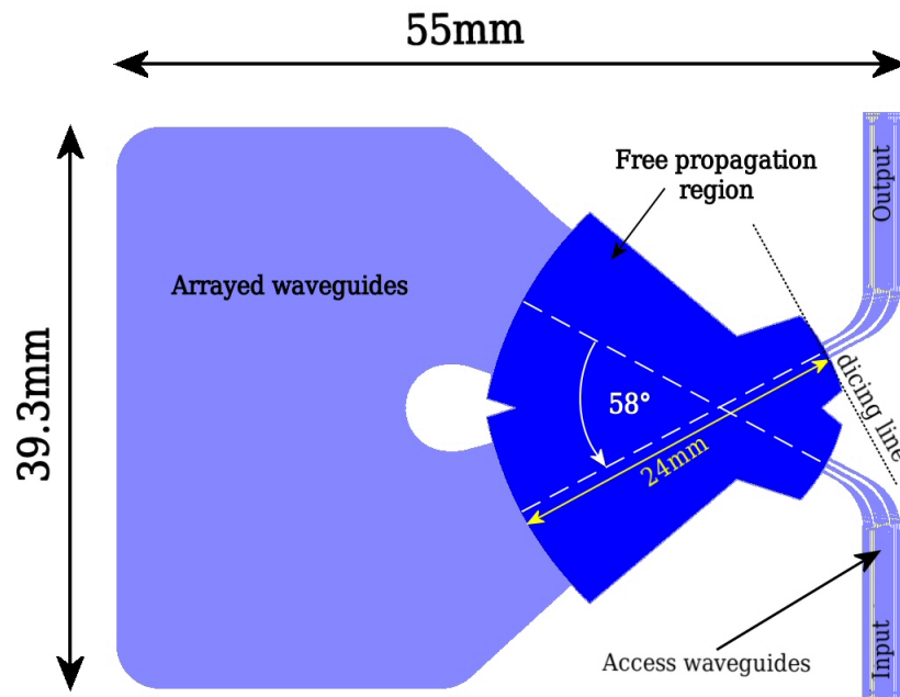
Figure 4. Layout of the high-resolution AWG device.
