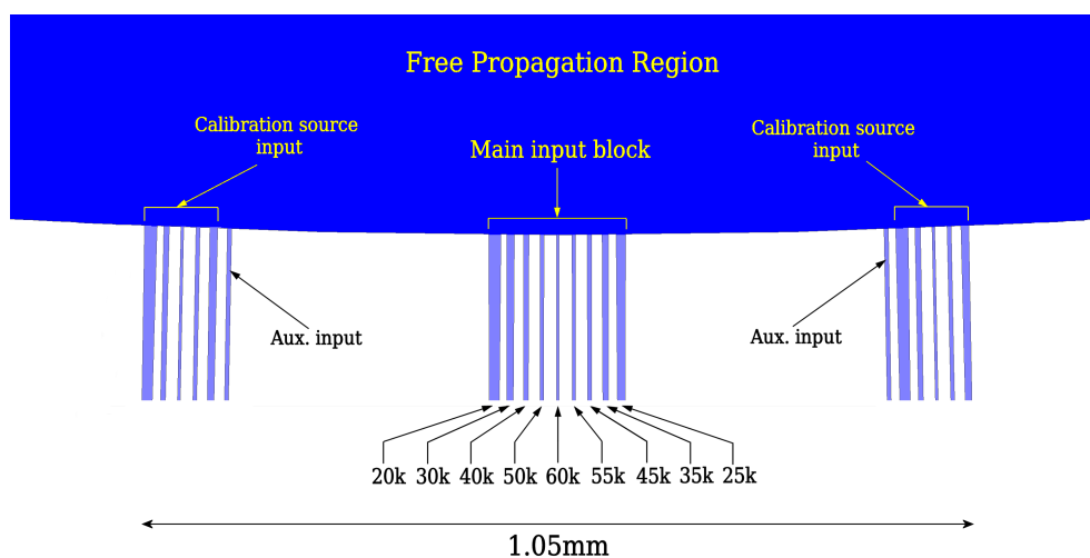
Figure 5. Input waveguide interface of the high-resolution AWG.
