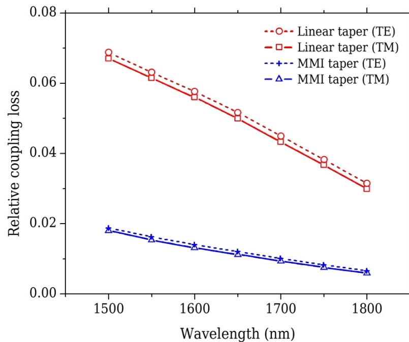
Figure 7. Comparison between the standard linear taper and the multimode interference (MMI) taper. Simulations were performed for TE and TM polarization in the wavelength range 1500 nm–1800 nm.
