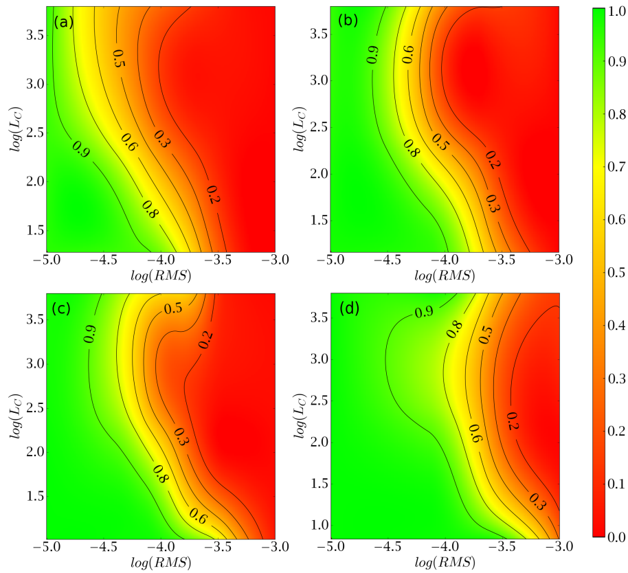
Figure 9. Simulation results for L = 24 mm (a); L = 18 mm (b); L = 12 mm (c); L = 6 mm (d).
