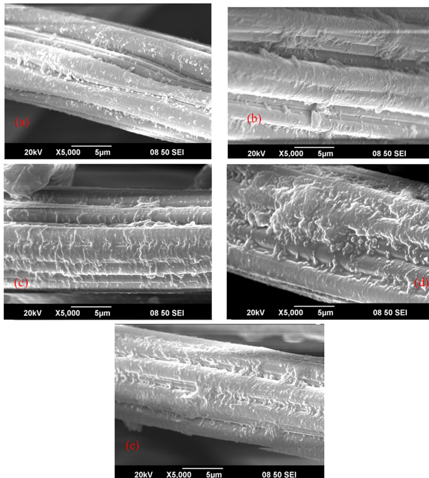
Figure 4. SEM micrographs illustrate the surface morphology of rayon flock synthetic leather after TMS plasma treatment with different discharge power: (a) untreated, (b) 30 W, (c) 40 W, (d) 50 W, (e) 60 W (treatment parameters: amount of TMS = 0.2 mL; flow rate of helium = 12.5 LPM; jet distance = 10 mm; treatment time = 30 s).
