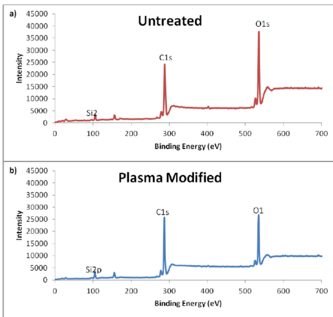
Figure 10. Surface elementary composition of (a) untreated and (b) TMS plasma-modified rayon flock synthetic leather (treatment parameters: amount of TMS = 0.2 mL; flow rate of helium = 12.5 LPM; discharge power = 50 W; jet distance = 10mm; treatment time = 30 s).
