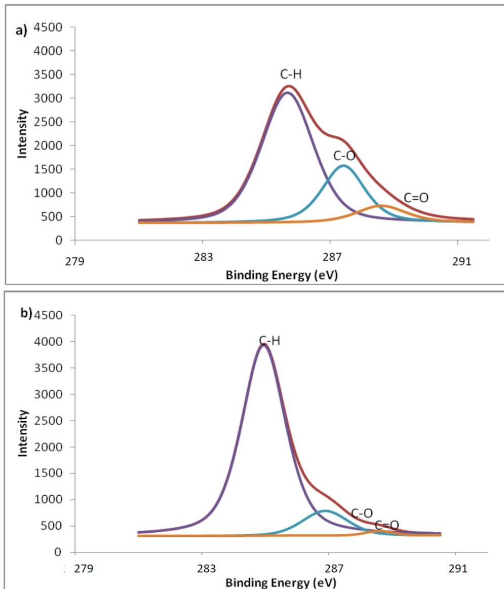
Figure 11. XPS deconvoluted C1s peak in (a) untreated sample and (b) plasma-modified rayon flock synthetic leather (treatment parameters: amount of TMS = 0.2 mL; flow rate of helium = 12.5 LPM; discharge power = 50 W; jet distance = 10 mm; treatment time = 30 s).
