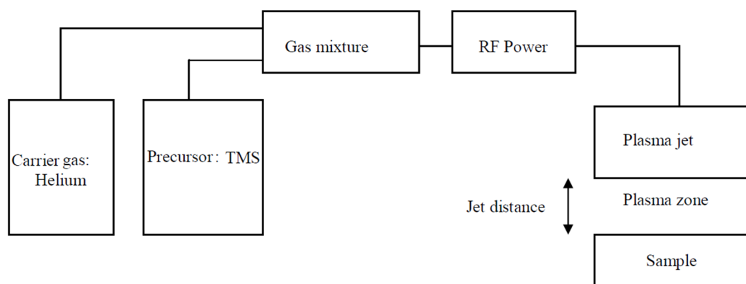
Figure 1. Schematic diagram of APP treatment.
