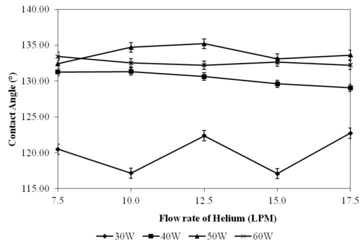
Figure 3. Contact angle of rayon flock synthetic leather after TMS plasma treatment (treatment parameters: amount of TMS = 0.2 mL; jet distance = 10 mm; treatment time = 30 s).
