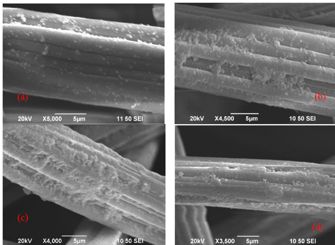
Figure 5. SEM micrographs illustrate the surface morphology of rayon flock synthetic leather after TMS plasma treatment with different treatment times: (a) 10 s, (b) 20 s, (c) 30 s, (d) 40 s (treatment parameters: amount of TMS = 0.2 mL; flow rate of helium = 12.5 LPM; jet distance = 10 mm; discharge power = 50 W).
