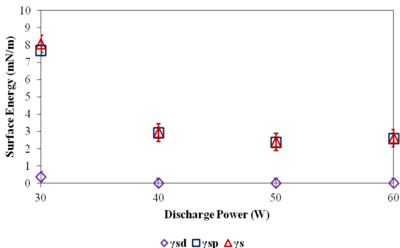
Figure 8. The change of surface energy of TMS plasma modified rayon flock synthetic leather (treatment parameter: amount of TMS = 0.2 mL; flow rate of helium = 12.5 LPM; jet distance = 10 mm; treatment time = 30 s).
