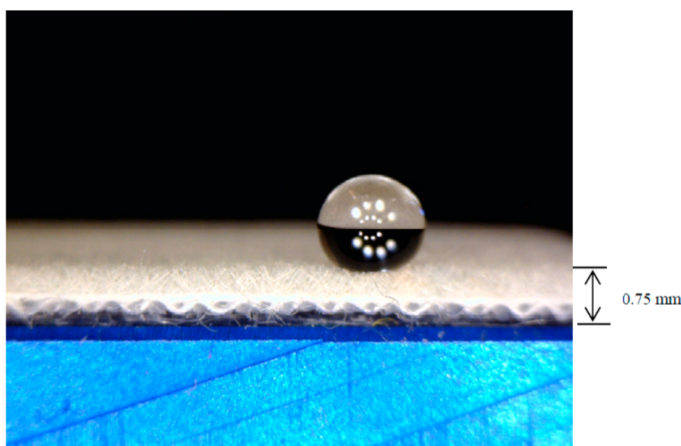
Figure 7. Photo showing contact angle of plasma-modified sample.
