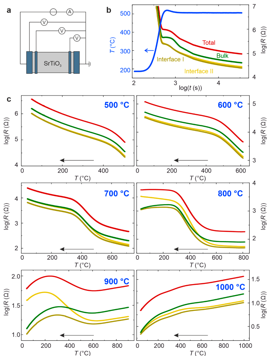
Figure 1. Four probe resistance measurements of the \text{SrTiO}_3 single crystal: (a) schematic setup; (b) total and partial resistances of the sample during the first heating to 500 °C; (c) cooling curves of the resistances after thermal reduction at increasing maximum temperatures.
