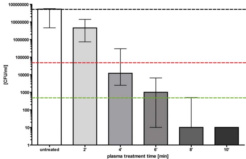
Figure 4. Decolonisation of MRSA using the FlatPlaSter plasma device. Cold atmospheric plasma treatment of MRSA (BAA-44) ( 10^{6-7} /ml) applied to ex vivo skin using the FlatPlaSter device. Different plasma treatment times were tested [min]. A CFU assay was performed immediately after the plasma treatment. Black dotted line: baseline of viable bacteria per ml; red dotted line: reduction of three \log_{10} steps of viable bacteria (99.9%); green dotted line: reduction of five \log_{10} steps of viable bacteria (99.999%). ( n=6 , median \pm interquartile range). doi:10.1371/journal.pone.0034610.g004
