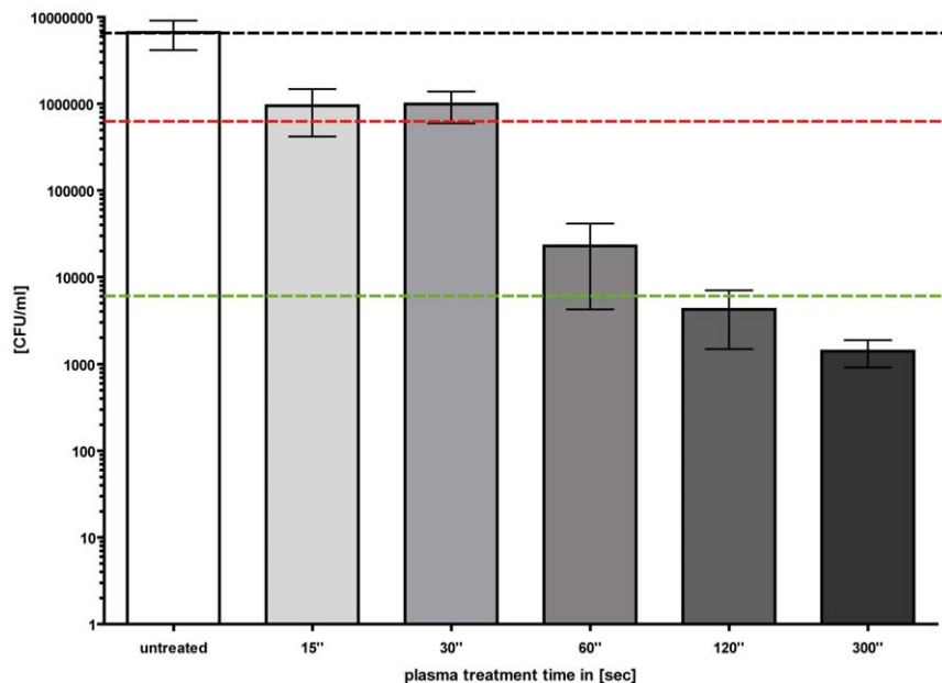
Figure 5. Decolonisation of S. aureus using the miniFlatPlaSter plasma device. Cold atmospheric plasma treatment of S. aureus ( 10^7 /ml) applied to ex vivo skin using the miniFlatPlaSter device. Different plasma treatment times were tested [sec]. A CFU assay was performed immediately after the plasma treatment. Black dotted line: baseline of viable bacteria per ml; red dotted line: reduction of one \log_{10} step of viable bacteria (90%); green dotted line: reduction of three \log_{10} steps of viable bacteria (99.9%). ( n=3 , mean value \pm standard deviation). doi:10.1371/journal.pone.0034610.g005
