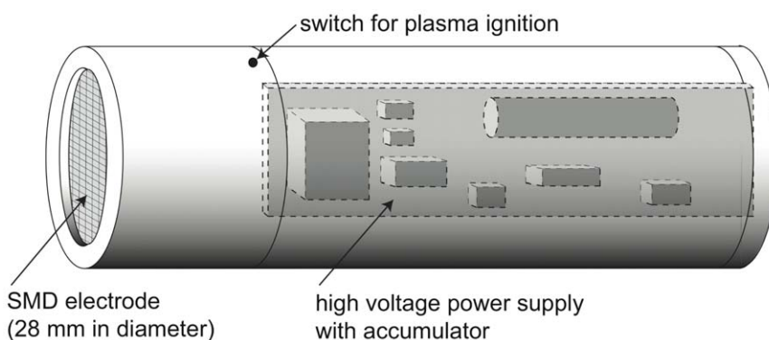
Figure 2. Schematic image of the miniFlatPlaSter plasma device. The portable plasma device is equipped with a high voltage power supply, accumulators, and a surface micro-discharge (SMD) electrode. The SMD electrode consists of a copper foil layer (around 0.2 mm thick), an Epoxy board (1 mm thick), and a stainless steel mesh of 28 mm in diameter. The plasma device was fixed above the ex vivo skin embedded in Hepes-Agar.
