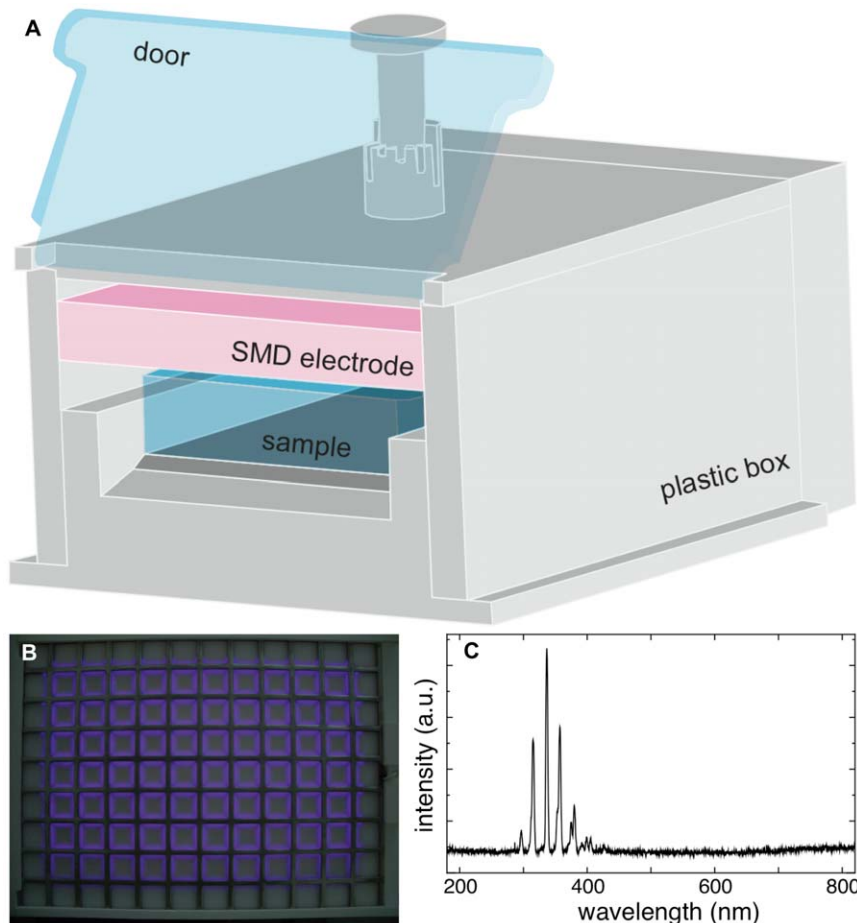
Figure 1. Schematic image of the FlatPlaSter plasma device. a) The FlatPlaSter contains one SMD electrode and the samples (to treat) are placed inside the device below the electrode. In this study the distance between the electrode and the sample surface was fixed at 6 mm. b) left: The plasma discharge is shown. On the mesh-side of the electrode, the SMD plasma was produced. c) right: The spectrum of the SMD plasma observed in front of the electrode with a distance of 6 mm is shown. The UV components in the range between 280–400 nm are mainly produced from nitrogen molecules excited by electrons.
