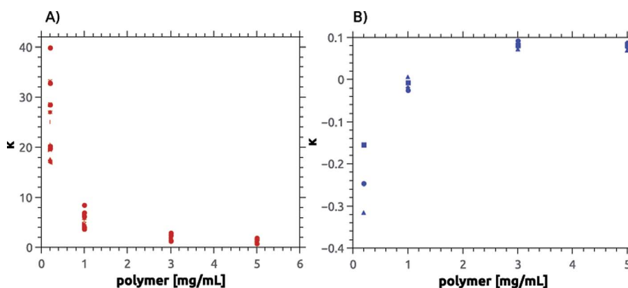
Fig. 8 Calcium dissolution per virtual monomer unit, \kappa . Panel (A) shows values for cationic, amphoteric and betainic polymers and (B) for anionic polymers. 65,88 Note the differences in the y-axis between (A) and (B).
