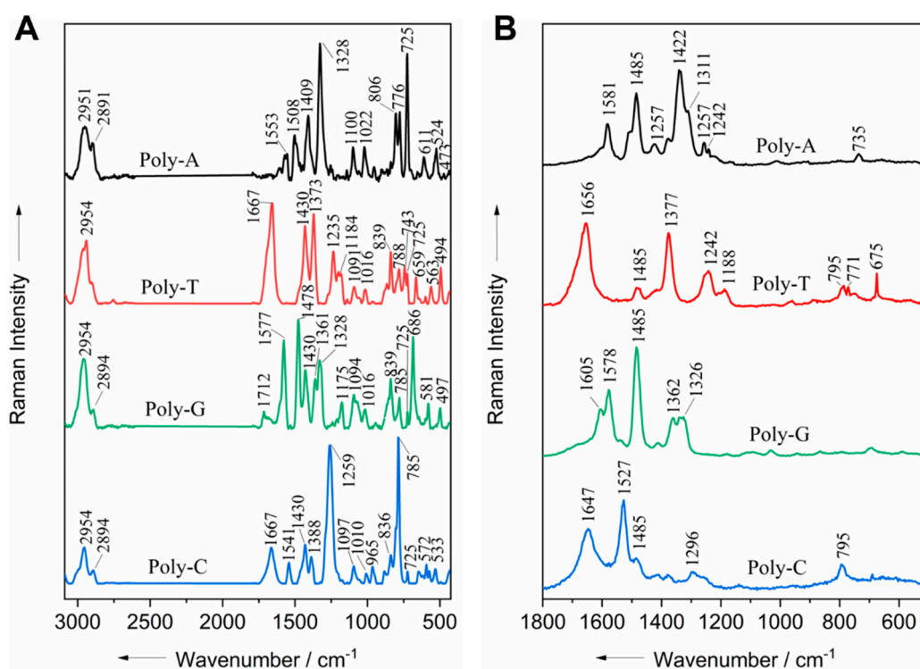
Figure 2. Raman spectra of oligonucleotides measured with visible excitation at 532 nm (A) and UVRR at 244 nm (B).
