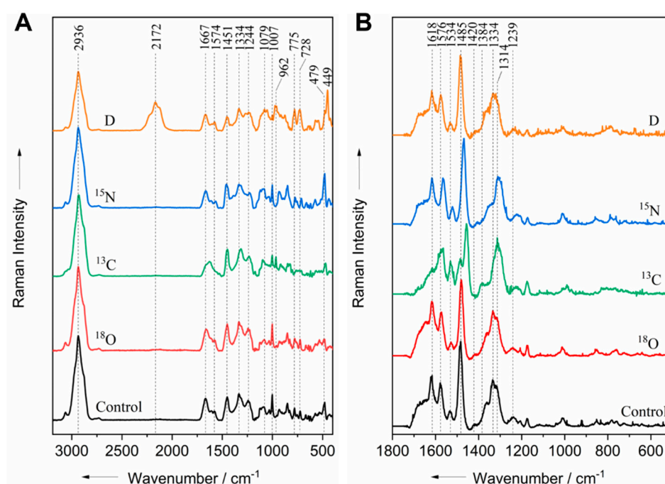
Figure 1. Raman spectra of isotopically labeled E. coli cells and unlabeled control acquired at the 532 nm (A) and 244 nm (B) excitation wavelengths.
