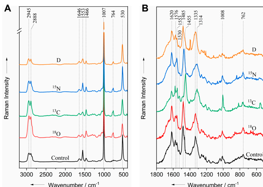
Figure 3. Raman spectra from DNA isolated from isotope-labeled bacterial cells and unlabeled control acquired at the 532 nm (A) and 244 nm (B) excitation wavelengths.
