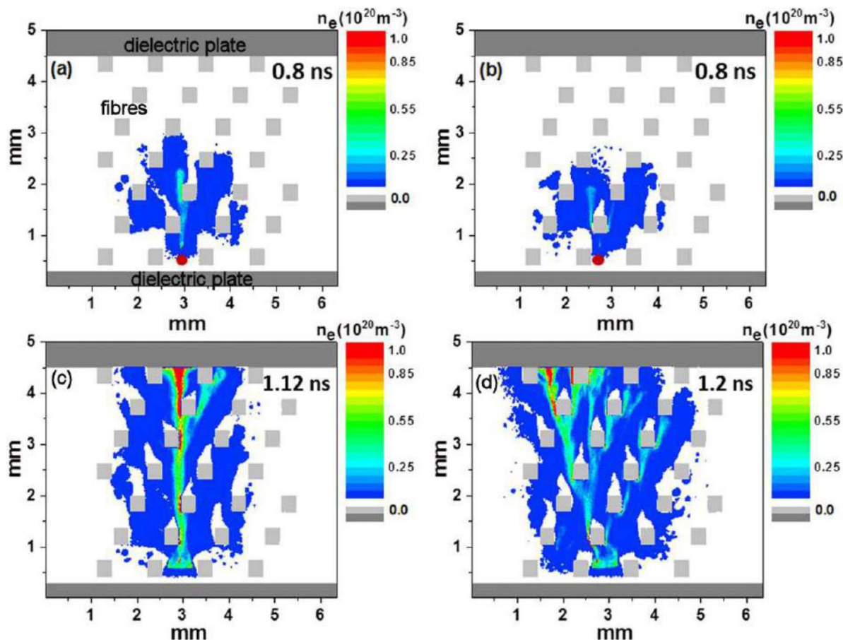
Figure 10. Predicted electron density distributions at 0.8 ns (a), (b) and when streamers reach the top of the dielectric at 1.12 ns (c) and 1.2 ns (d) in a three-dimensional fibre bed for different locations of streamer initiation (see red dots in (a), (b): at the centre of the channel (a), (c); near the edge of the channel (b), (d)). The dark-grey dielectric plates cover the electrodes, and the light-grey fibres are perpendicular to the plane of the figure. Reproduced from [68]. © IOP Publishing Ltd. All rights reserved.
