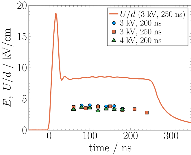
Figure 13. Electric field temporal development at 500 μm from the cathode measured by E-FISH technique (symbols) for different HV pulses compared with the electric field profile calculated as voltage over gap ratio for the 3 kV, 250 ns measurement (line). As the voltage amplitude during the plateau phase is quite similar for all three measurements (see figure 12) only one waveform is shown.
