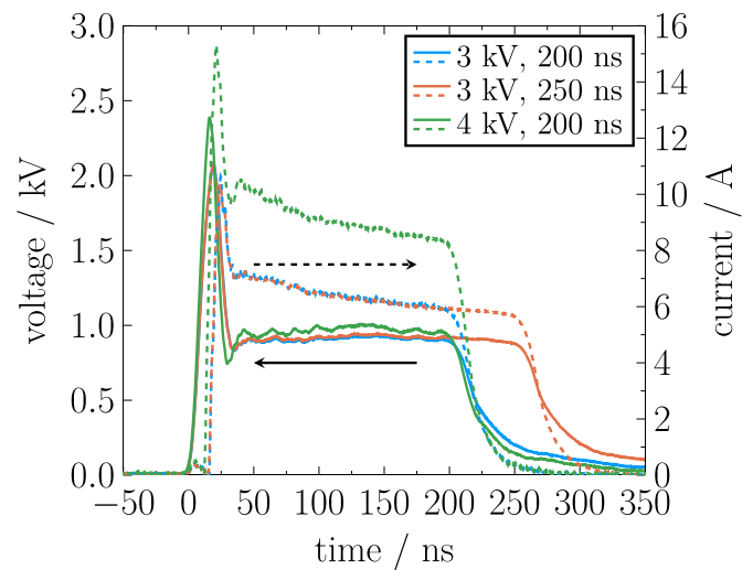
Figure 12. Voltage (solid lines) at the powered electrode and current (dashed lines) to ground during the discharge for the different applied voltage pulses. While the maximum peak voltage at the time of the breakdown increases for the higher applied voltage it can be noted that the voltage drop over the discharge gap during the following plateau is nearly the same for all three conditions. The current on the other hand is significantly higher for the 4 kV case.
