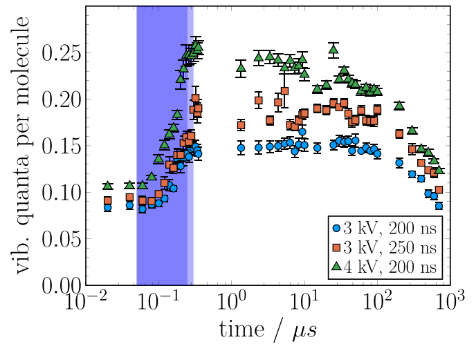
Figure 20. Vibrational quanta per molecule for all three measurements. The blue rectangles mark the on-time of the discharge pulse with 200 ns (dark shaded) and 250 ns (light shaded).
