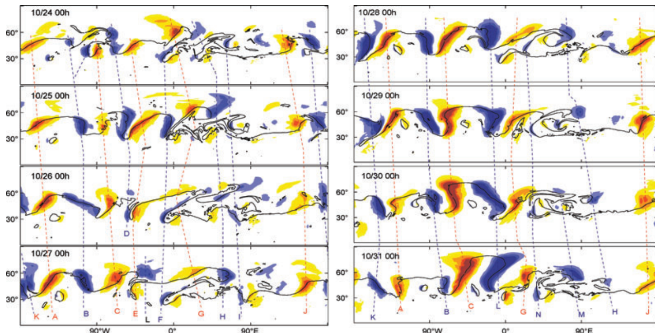
Fig. 12. Representation of the synoptic situation during the short episode from October 24 to 31 on the 330K isentropic surface. Black line: 2 PVU-contour, bluish colours: negative meridional wind [(-20, -30, -40, -50) \text{ m}^2 \text{ s}^{-2}] , reddish colours: positive meridional wind [(20, 30, 40, 50) \text{ m}^2 \text{ s}^{-2}] . The blue (negative meridional wind) and red (positive meridional wind) dashed lines denote the position of the extrema in the meridional wind, that are also indicated with the same labels in Fig. 13.
