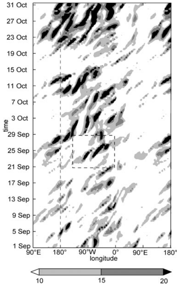
Fig. 5. Hovmöller diagram of \overline{K_e} (in 10^5 \text{ Jm}^{-2} ) for the episode September and October 2008. The data are vertically integrated between 1000 and 100 hPa and averaged over a latitude belt between 40^\circ and 60^\circ\text{N} . The temporal resolution of the data for this analysis is 12 h. The dashed box refers to the area of Fig. 8.
