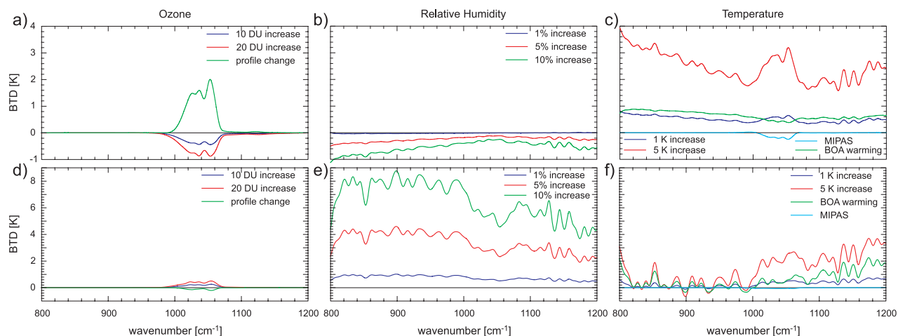
Fig. 4. Simulated BTDR resulting from subtraction of spectra obtained under the assumption of a modified profile from the reference tropical standard atmosphere. Figures a–c (top row) display the effect on the upwelling radiation at TOA while Figures d–f visualise the sensitivity of the downwelling radiation at BOA. Note that different BTDR scales are used for BOA and TOA spectra.
