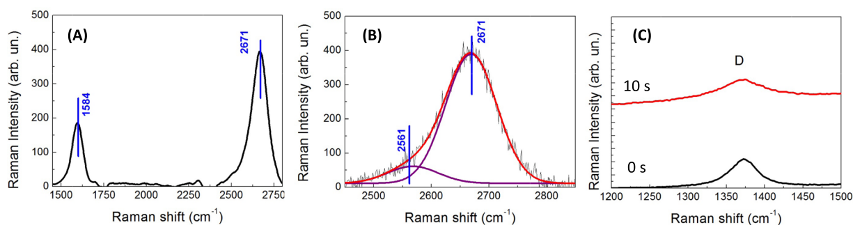
Figure 3. (A) Raman spectrum of flakes obtained after 10 s of laser irradiation and deposited on copper; (B) details of the 2D structure located around 2650\text{ cm}^{-1} (red and violet curves indicate the Gaussian fit); (C) details of the (D) structures for bulk graphite (black line) and for Graphene bi-layer produced after 10 s of laser irradiation.
