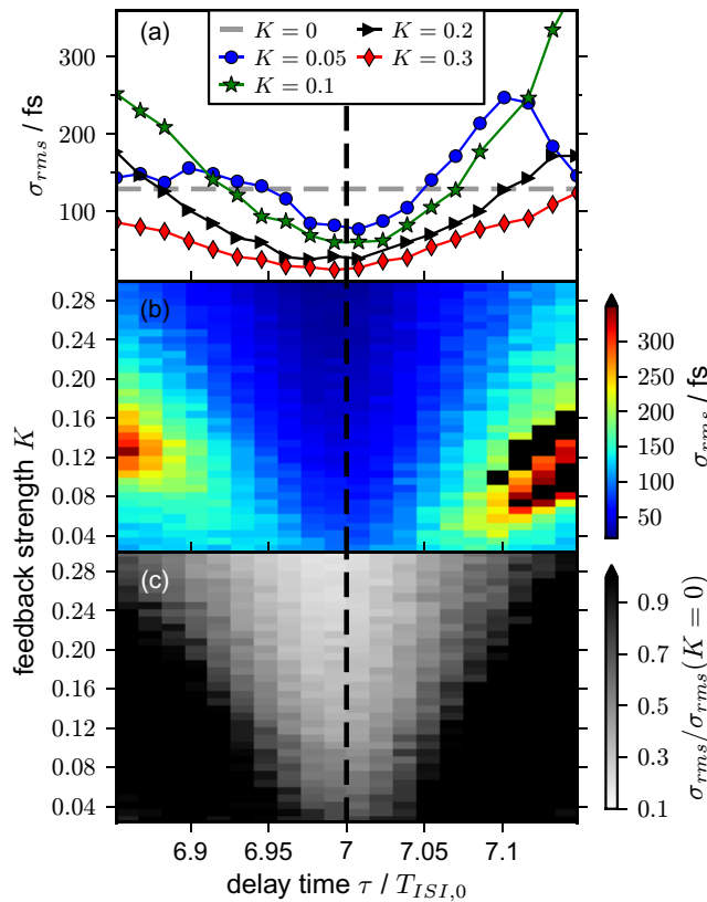
Figure 13. The rms timing jitter \sigma_{rms} as a function of the delay time \tau in an interval around the main resonance with \tau = 7T_{ISI,0} for a noise strength of D = 0.05 . ( T_{ISI,0} is the inter-spike interval time for the solitary laser.) (a) \sigma_{rms} for various feedback strengths K . (b) Density plot of \sigma_{rms} (color code) as a function of \tau and K . (c) Density plot of \sigma_{rms} (color code) normalized to the rms-timing jitter of the solitary laser ( \sigma_{rms}(K = 0) ).
