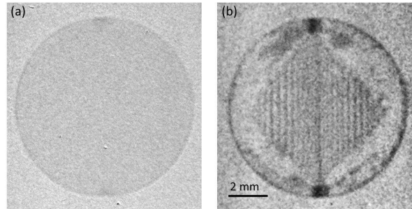
Fig. 3. Absorption contrast image (a) and darkfield image (b) of a FeSi sheet.
