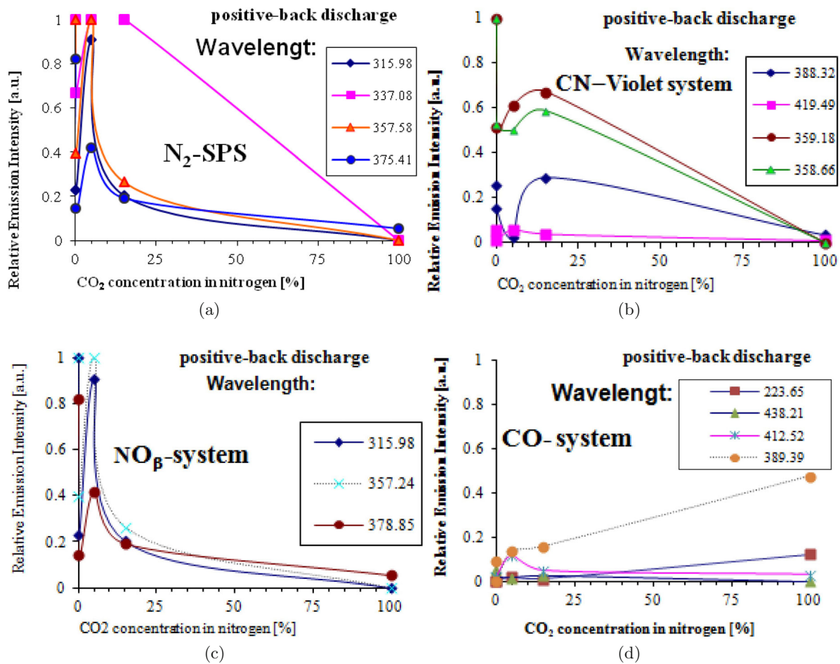
Fig. 13. Relative emission intensity of various gas compounds (a) N_2 , (b) CN, (c) NO, and (d) CO, as function of CO_2 concentration at atmospheric pressure for positive polarity of the discharge electrode. Supply voltage 30 kV.
