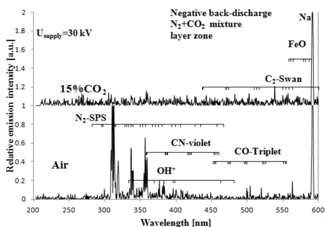
Fig. 10. Comparison of back discharge emission spectra in 15% CO_2 + 85% N_2 and in air for negative polarity of discharge electrode, taken from in the layer zone. Supply voltage -30 kV.
