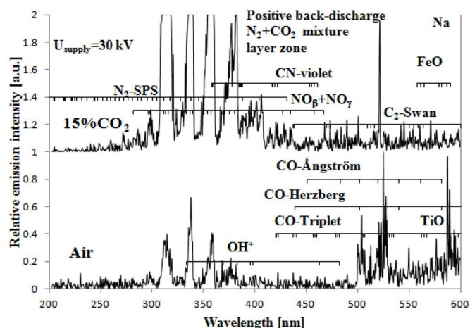
Fig. 11. Comparison of back discharge emission spectra in 15% CO_2 + 85% N_2 and in air for positive polarity of discharge electrode, taken from in the layer zone. Supply voltage +30 kV.
