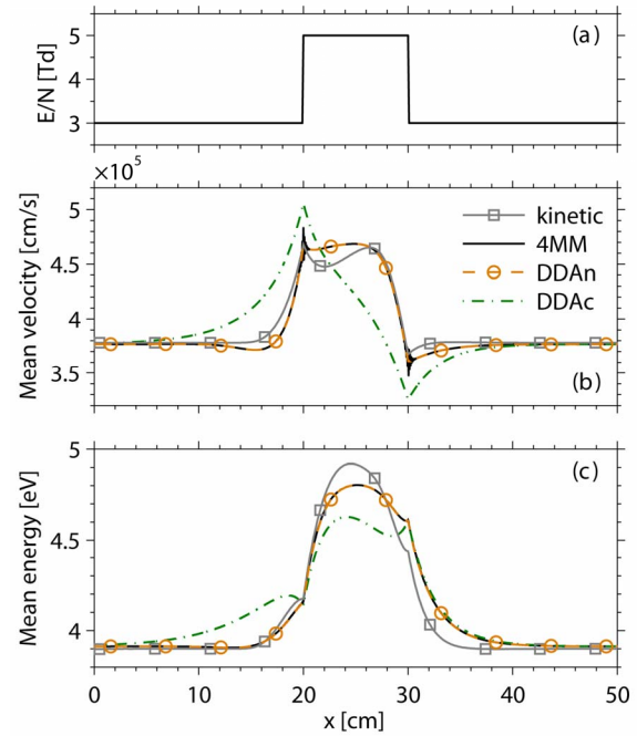
Figure 3. Prescribed electric field (a) and comparison of results for the mean velocity (b) and energy (c) of the electrons obtained by the four-moment model 4MM and drift-diffusion models DDAn and DDAc with kinetic results.
