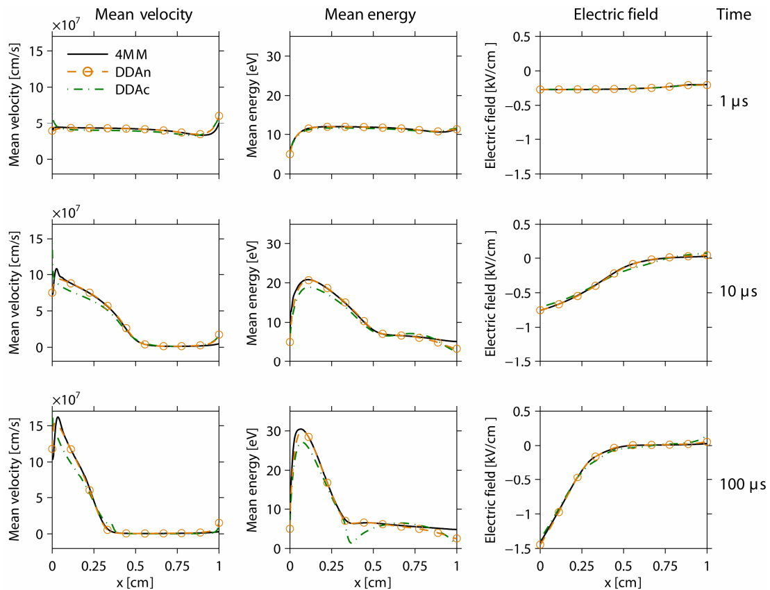
Figure 4. Comparison of results obtained by the fluid models 4MM, DDAn and DDAc for an abnormal glow discharge in argon at pressure of 133 Pa and applied voltage of -250 V.
