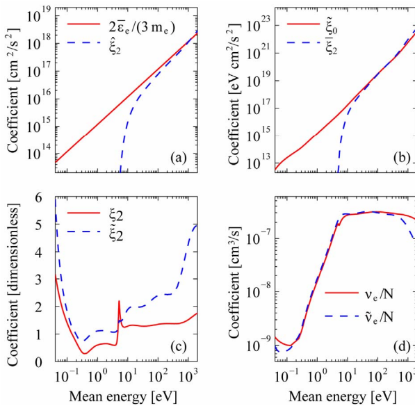
Figure 2. Argon transport coefficients for electron particle flux in drift-diffusion approximation DDAn (a); energy flux in drift-diffusion approximation DDAn (b); particle and energy fluxes in four-moment model 4MM (c); and dissipation frequencies for particle and energy fluxes (d).
