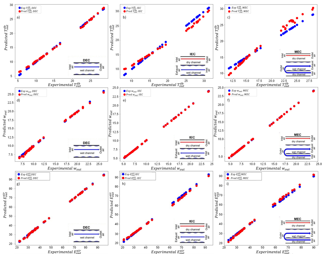
Figure 13. Assessment of the E-AC systems(DEC, IEC, and MEC) based on the experimental and predicted results considering the output features of (a–c) T_{out}^{db} , (d–f) w_{out} , and (g–i) E_{out}^{air} .
