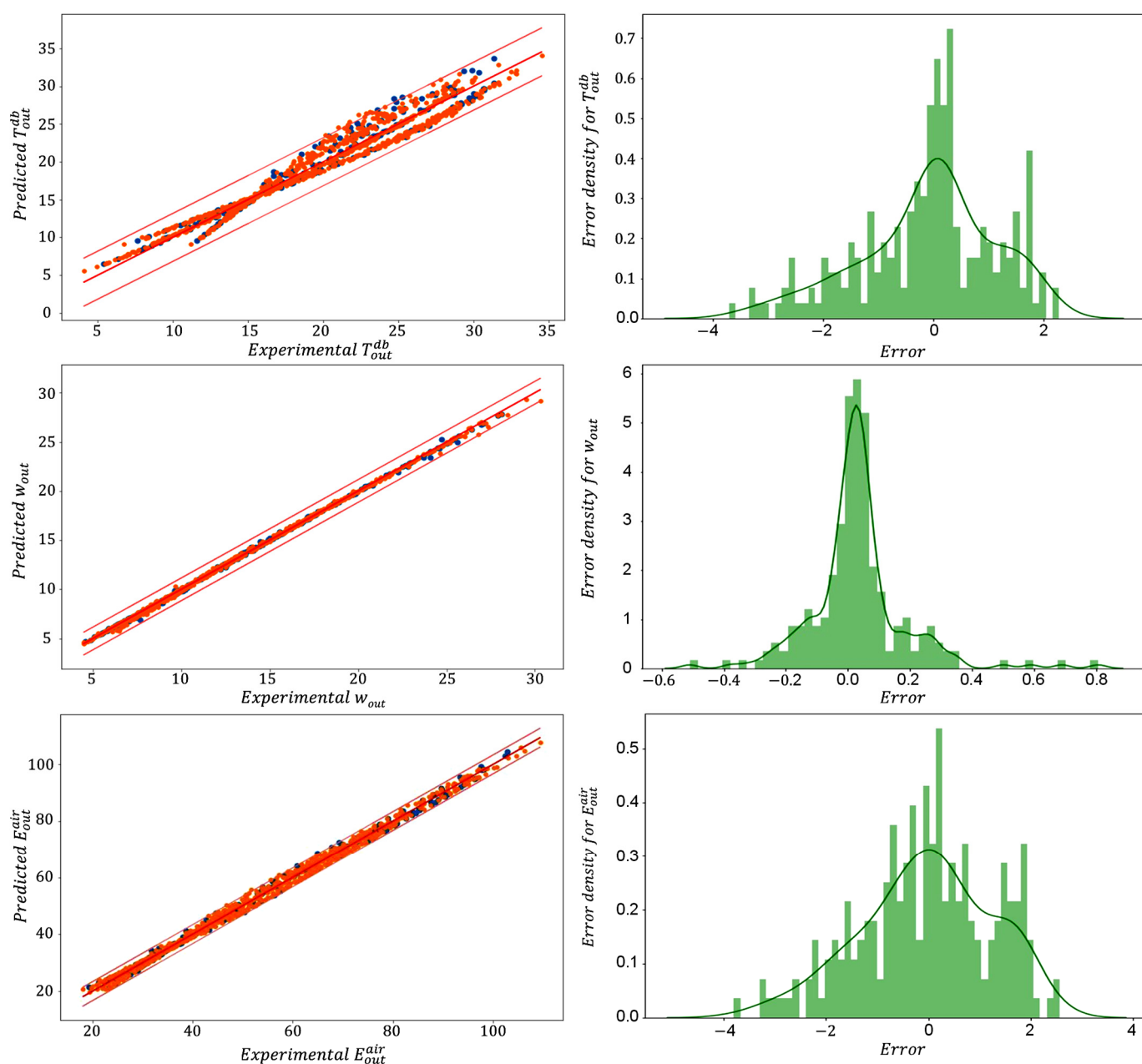
Figure 12. Analysis of the correlation coefficients and error densities of the developed AI model.
