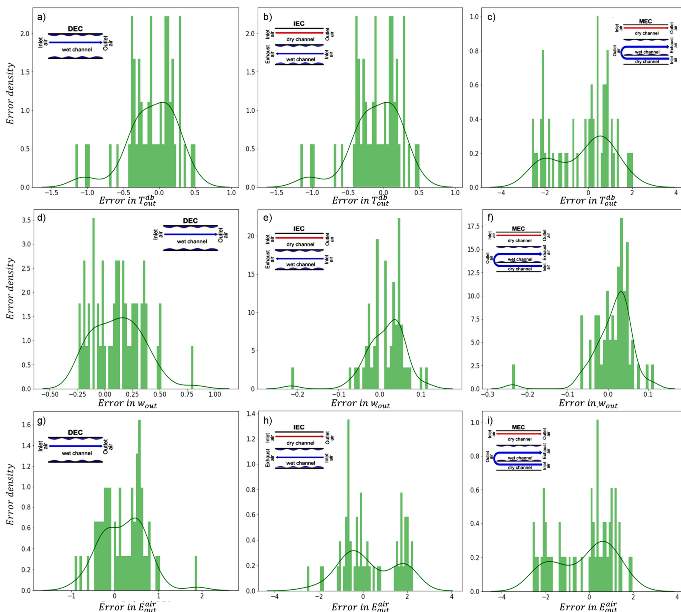
Figure 14. Error density analysis in output features (a–c) T_{out}^{db} , (d–f) w_{out} and (g–i) E_{out}^{air} produced by developed AI model for predicting the thermal performances of the E-AC systems (DEC, IEC, and MEC).
