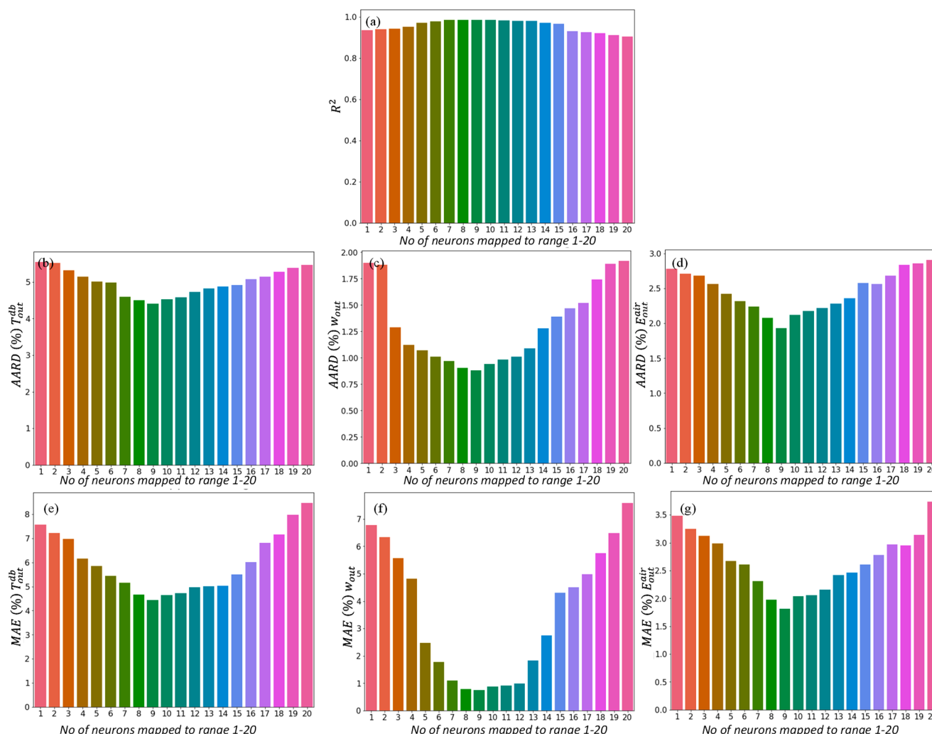
Figure 11. Variations in (a) R^2 , (b–d) AARD\% , and (e–g) MAE\% with different numbers of neurons in the hidden layers.
