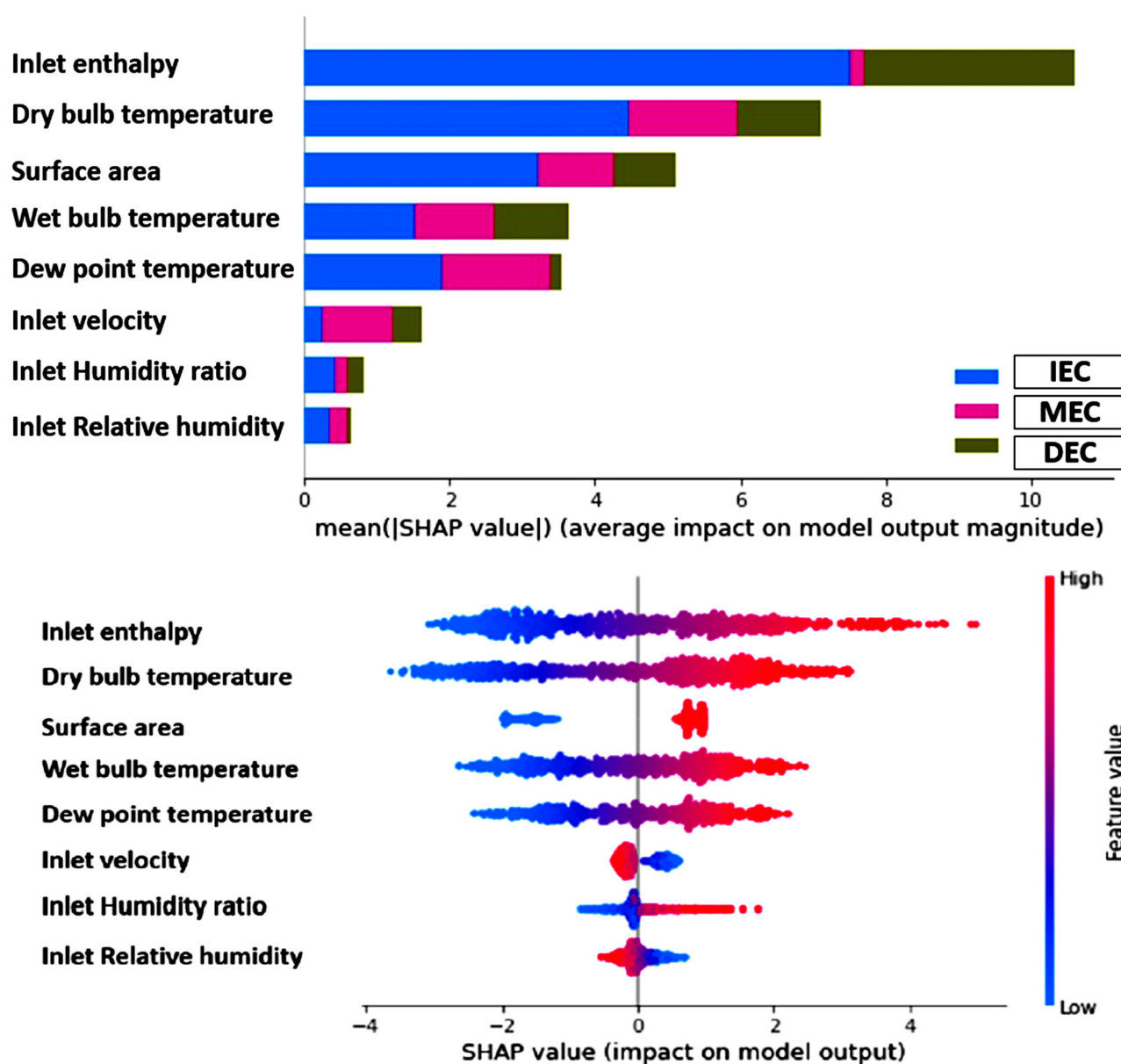
Figure 15. Average impact of each feature on the model's output for the three E-AC systems.
