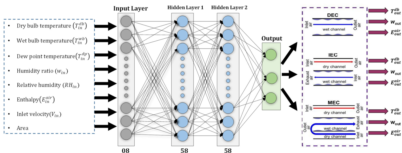
Figure 9. Structure of the optimal deep learning model.
