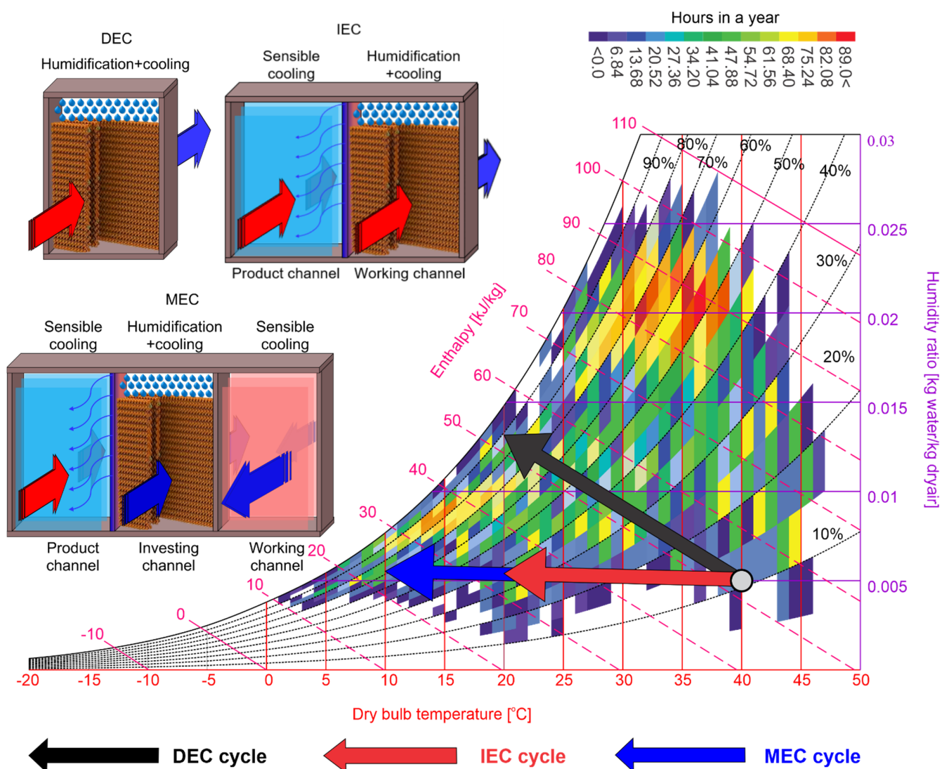
Figure 1. Working principles of E-AC systems and their open-cycle psychrometric presentations with hourly variations of the ambient conditions in Pakistan.
