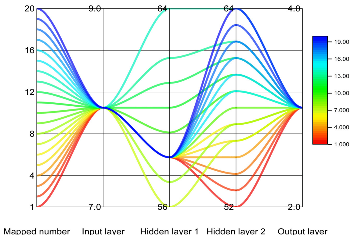
Figure 8. Mapping of the number of neurons in the hidden layers.
