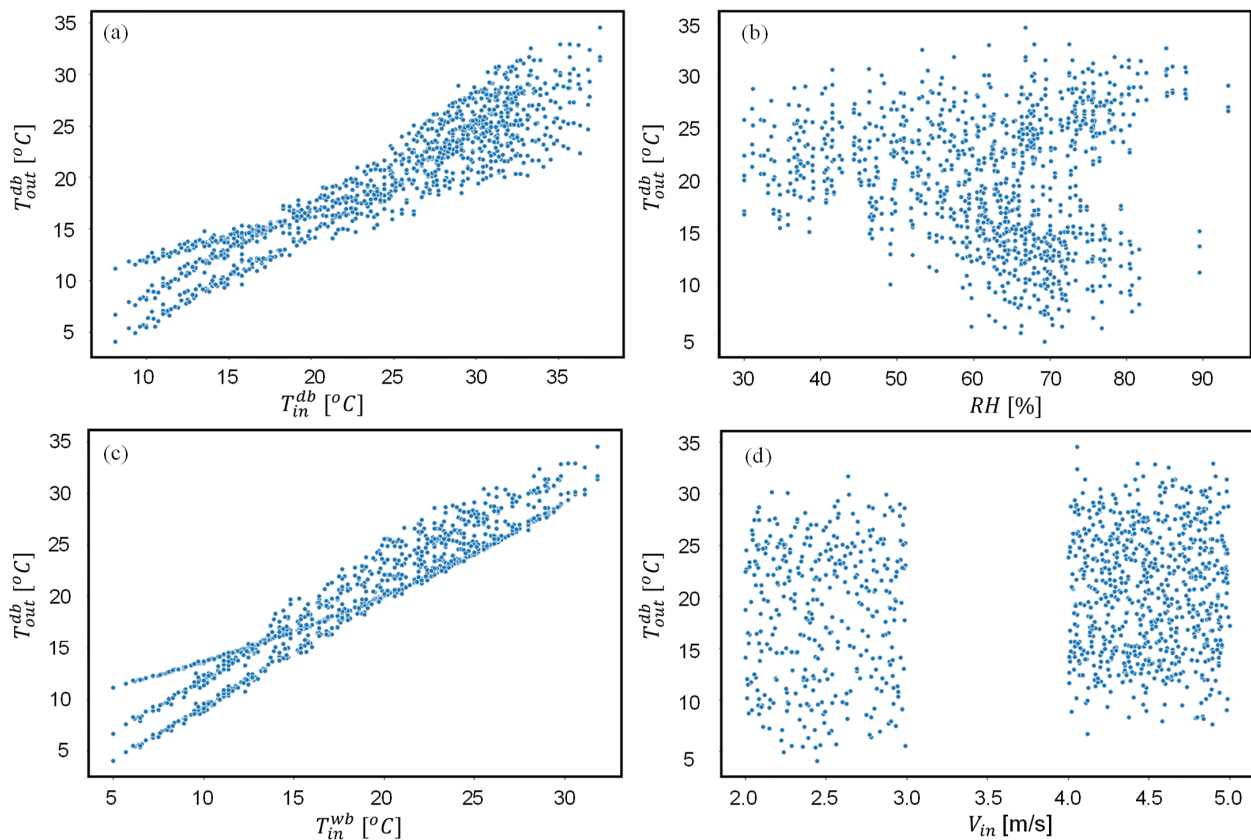
Figure 6. Plotting of the E-AC systems' output dry-bulb temperatures with respect to the inlet (a) dry-bulb temperature, (b) relative humidity, (c) wet-bulb temperature, and (d) velocity.
