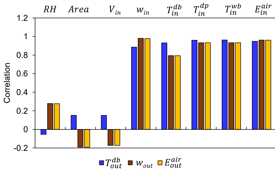
Figure 5. Correlation graph of the most influential input features corresponding to the output features.
