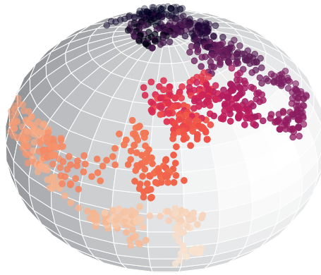
Figure 1: Typical random walk on the unit sphere with initial position \eta_0 = 0 and \phi_0 = \pi/2 . One thousand steps were taken with an arc length of 0.06. The colours indicate the time evolution, going from dark to light.
