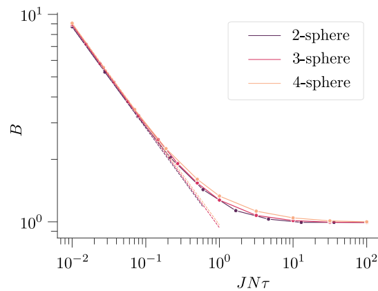
Figure 5: The relation between B and JN\tau yielding Born's rule when the stochastic process is interpreted as a random walk on either a 2-, 3-, or 4-sphere. The dashed lines show fits of the low- JN\tau regime of the form B = \gamma/(JN\tau)^\alpha . The best-fit values for the 2-sphere are \gamma = 0.919 and \alpha = 0.49 , while those for the 3-sphere are \gamma = 0.936 and \alpha = 0.49 , and we find \gamma = 0.966 and \alpha = 0.49 for the 4-sphere.
