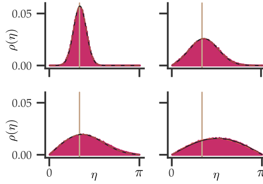
Figure 2: Probability distribution for the latitude angle \eta , after a random walk on the sphere with 10, 500, 1000, and 10000 steps of arc length 0.03. Here, we used the initial values \eta_0 = \pi/3 (indicated by a vertical light brown line) and \phi_0 = \pi/2 . The black line shows the Ansatz of equation 13 with \sigma^2 = d_{\text{step}}^2 t/2 and |n|_{\text{max}} = 500 . The orange dashed line indicates only the n = 0 term and is seen to diverge from both the numerical average and the black line only at late times.
