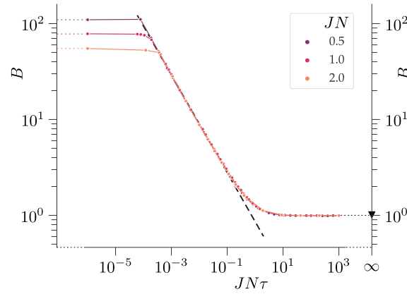
Figure 4: Parameter values yielding Born's rule. The simulation is carried out for JN = 0.5 (dark), JN = 1 (middle), and JN = 2 (light). In each case, three regimes can be identified, corresponding to large, medium and small values of JN\tau . The dashed black line indicates a fit for the central regime, of the form B = \gamma/(JN\tau)^\alpha with \gamma \approx 0.92 and \alpha = 0.50 . The downward triangle on the right side indicates the exact result B = 1 for the limit JN\tau \rightarrow \infty , corresponding to constant noise or macroscopic measurement machines. The relation between JN\tau and B can be seen to become non-universal (dependent on JN ) for small values of JN\tau , where the approximation of a continuous noise process using finite step size breaks down. Each circular point along the curves represents the value of B giving Born's rule as determined using a bisection method at fixed \theta_0 , and probabilities after averaging over 100000 evolutions using arc length steps of 0.05 for the noise.
