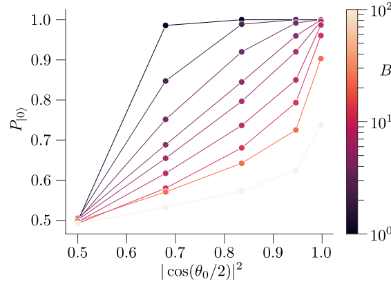
Figure 3: Probability of evolving towards the stable fixed point corresponding to the pointer state |0\rangle , as a function of the initial value \theta_0 . The colours indicate different values for B , ranging from 1 to 100. For each instance of the state evolution, 2000 time steps in the evolution of \theta are considered to determine its final state, and each point in the figure corresponds to the final state average of 10000 such evolutions. To minimise the effect of the fixed step size in the evolution of the noise, the noise takes 100 steps of arc length 0.1 before each new step in the evolution of the state.
