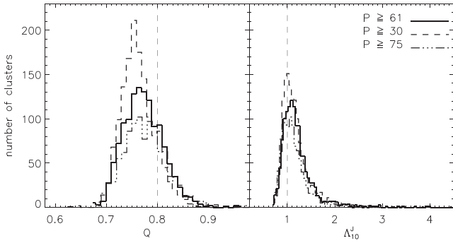
Figure A2. The dependence of the distribution of the structure parameter Q (left-hand panel) and of the mass segregation ratios \Lambda_{10}^J (right-hand panel) on the choice of the stellar membership probability, P . The fiducial case corresponds to the case with P \geq 61 per cent (full line, 1276 clusters). A higher/smaller value of the threshold probability reduces/increases the number of clusters in the sample. For P \geq 30 per cent and P \geq 75 per cent, the number of clusters is 1464 and 998, respectively. The vertical dotted lines show the division between hierarchical and centrally concentrated clusters at Q = 0.8 and the division between non-mass-segregated and mass-segregated clusters at \Lambda_{10}^J = 1 , respectively.
