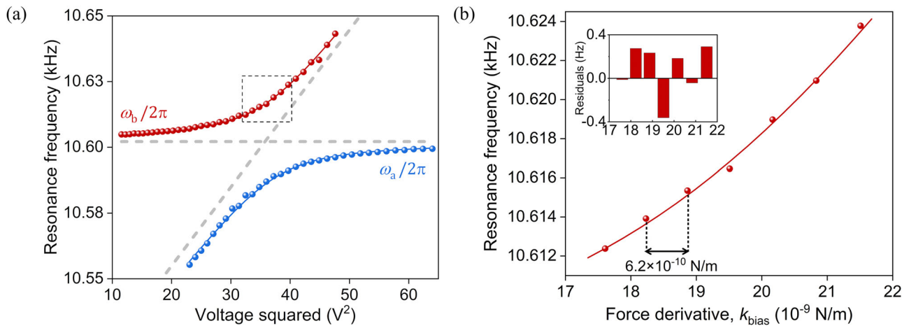
Fig. 2 Frequencies of coupled modes. The measurements of device #1 are shown where spheres and solid lines refer to measurements and fitted curves, respectively. a Avoided level crossing of \omega_a (shown in blue) and \omega_b (shown in red) controlled by the bias voltage V . The cantilever frequency and the nanowire (NW) frequency \omega_{\text{NW}}^2 = (k_{\text{NW}} + k_{\text{bias}})/m_{\text{NW}} are indicated by gray dashed lines. b Magnified view of the section indicated by the dashed rectangle in a . The horizontal axis, i.e., the V -induced interaction, is represented as k_{\text{bias}} = rV^2 . Here, r = 5.4 \times 10^{-10} \text{ Nm}^{-1}\text{V}^{-2} as extracted from curve fitting. In the inset, \omega_b residuals are shown.
