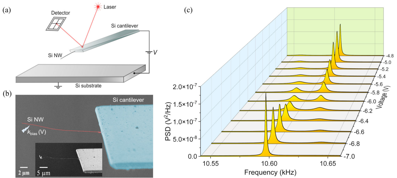
Fig. 1 Experimental setup and V-dependent frequency response. a Scheme of the detection technique where thermal fluctuations are read at the cantilever in a conventional scanning probe microscopy (SPM) device. b Scanning electron microscopy (SEM) image of a coupled oscillator consisting of a silicon nanowire (Si NW) and a tip-less Si cantilever (device #1). The lightning bolt symbol indicates a bias voltage-induced force derivative acting on the coupled oscillator as described by k_{bias} . Inset: The same coupled oscillator after frequency matching by electron-beam-assisted deposition onto the NW free end. c Waterfall plot of cumulative curve fitting of the V-dependent power spectral density (PSD) of the thermal noise measured optically at the cantilever of device #1 at room temperature.
