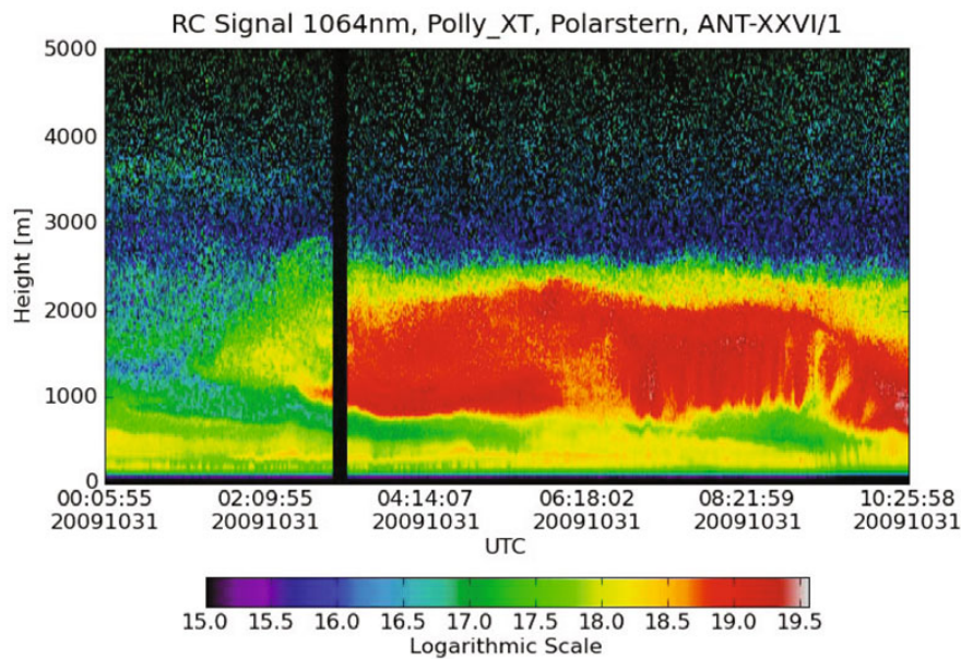
Fig. 4. Backscatter profile of the POLLY-XT lidar during the passage below a Saharan dust Storm event. Diagram by Thomas Kanitz.
