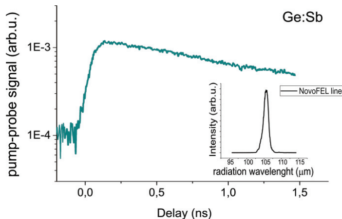
Fig. 2. Pump-probe signal vs. delay time for Ge:Sb sample at 105 \text{ } \mu\text{m} wavelength, recorded at NovoFEL. Sample temperature: 5 K. Inset: NovoFEL emission line.
