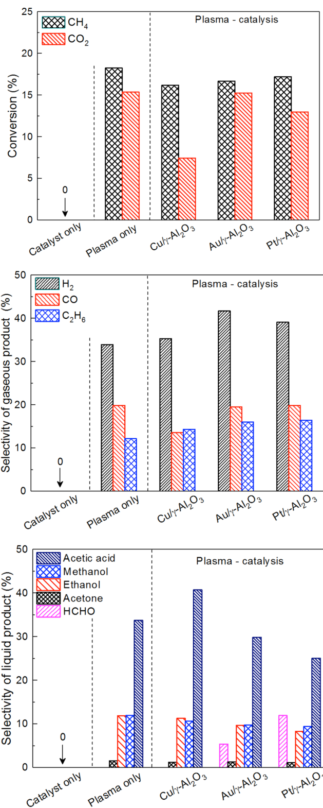
Figure 7. Conversion of CO 2 and CH 4 (top) and selectivity of gaseous products (middle) and liquid products (bottom) for catalyst only, plasma only, and plasma catalysis for three different catalyst materials in a DBD at 30 °C and atmospheric pressure. 31
