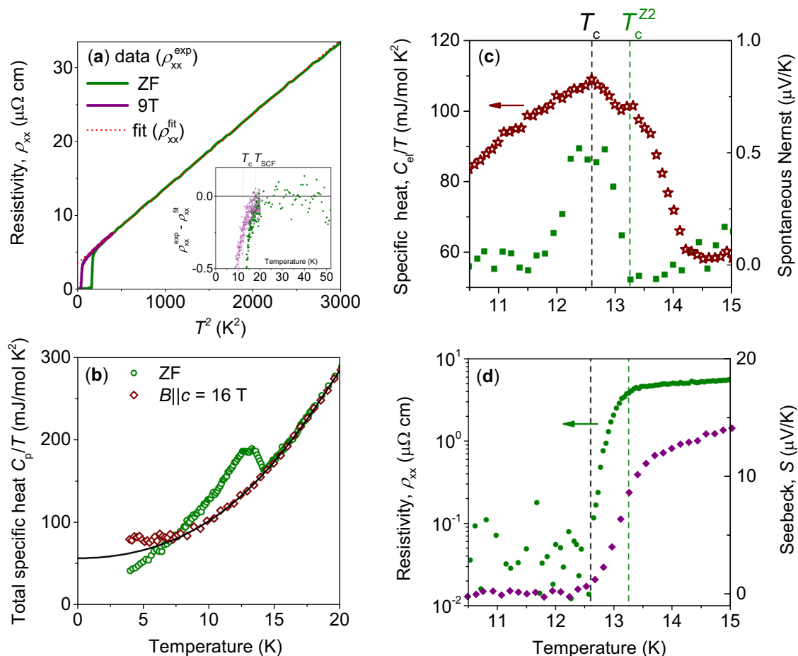
Fig. 2 | Two phase transitions in \text{Ba}_{1-x}\text{K}_x\text{Fe}_2\text{As}_2 . The figure shows the experimental data for S2 sample. a The longitudinal electrical resistivity vs. temperature squared measured in zero and B||c = 9 \text{ T} field applied along the crystallographic c -axis. The inset shows the temperature dependence of the difference between the fit curves and the experimental data. The resistivity deviates from the normal state behavior at the crossover temperature T_{\text{SCF}} associated with the onset of superconducting fluctuations. b Temperature dependence of the specific heat measured in zero and B||c = 16 \text{ T} field. The solid line is a fit to approximate the normal state behavior. A two-step anomaly is seen in the zero-field specific heat data. c (left axis)
