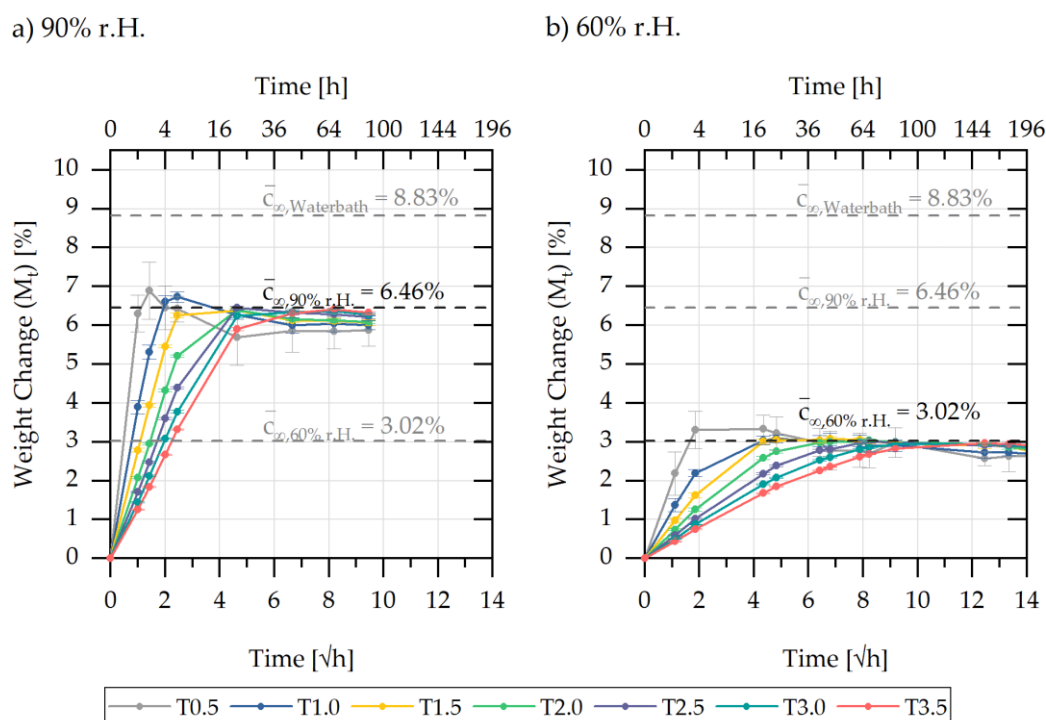
Figure 7. Sorption curves of the different bar specimens and the step-shaped specimen stored in (a) 90% r.H. and (b) 60% r.H. in a climate chamber at 84 °C.
