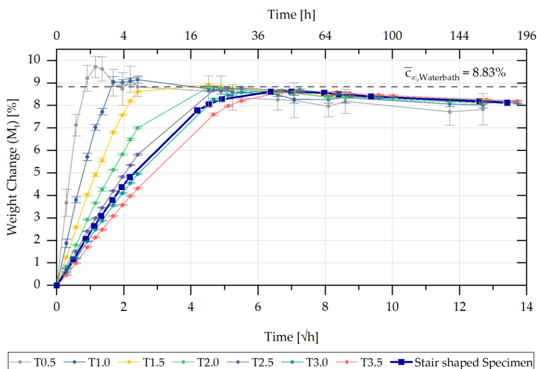
Figure 6. Sorption curves of the different bar specimens and the step-shaped specimen stored in a water bath at 81 °C.
