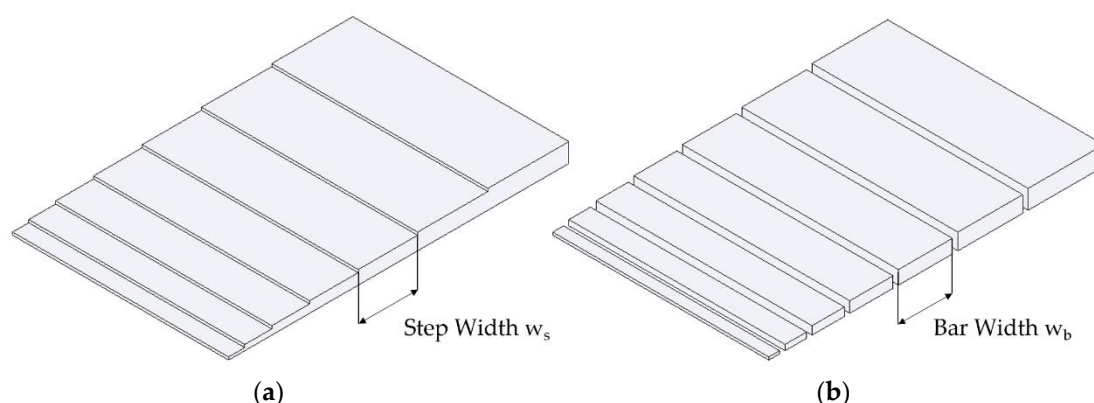
Figure 4. Step shaped part geometry (a) and bar-shaped samples cut from step part (b).
