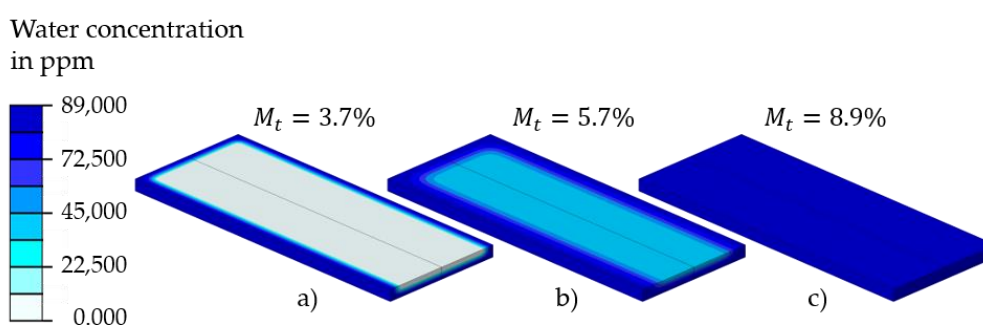
Figure 11. Water concentration of a T2.0 sample for the computation steps: (a) t = 1.4 \sqrt{h} , (b) t = 2.4 \sqrt{h} , (c) t = 12 \sqrt{h} .
