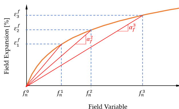
Figure 3. Determination of the expansion coefficient [40].
