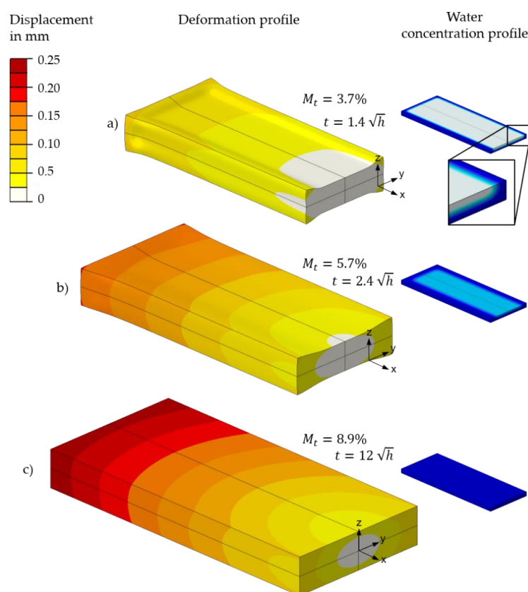
Figure 14. 50× enlarged illustration of the swelling-induced deformation for the corresponding water concentration distributions at the computation steps: (a) t = 1.4 \sqrt{h} , (b) t = 2.4 \sqrt{h} , (c) t = 12 \sqrt{h} .
