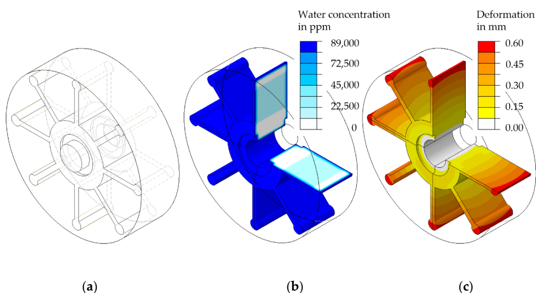
Figure 16. Illustration of a (a) pump impeller and its (b) calculated water absorption as well as the (c) swelling-induced deformation.
