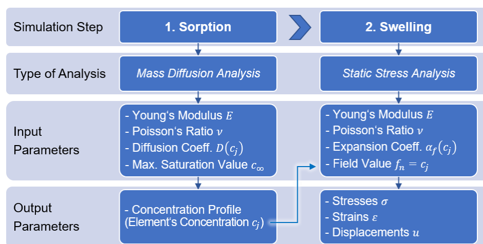
Figure 2. Schematic representation of the successive simulations to calculate the sorption and swelling behaviour of PA6 in water using Abaqus.
