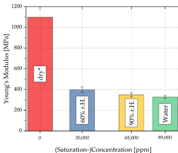
Figure 10. Concentration-dependent Young's moduli for the different ambient humidities. * The value for dry material is based on data sheet values.
