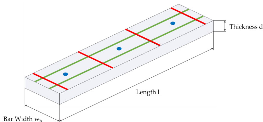
Figure 5. Measurement points for the test specimens, green tactile, red, and blue determined using a digital microscope.
