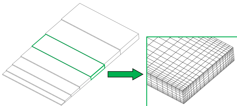
Figure 12. Schematic illustration of the mesh refinement to the boundary layer of a calculated part.
