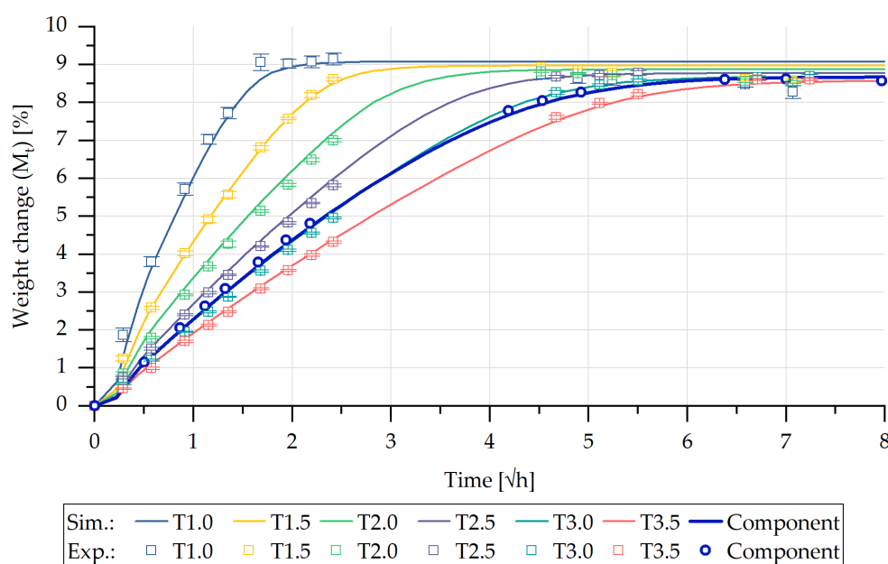
Figure 13. Comparison of the experimentally and computationally determined sorption curves of the individual bar geometries and step-shaped part.
