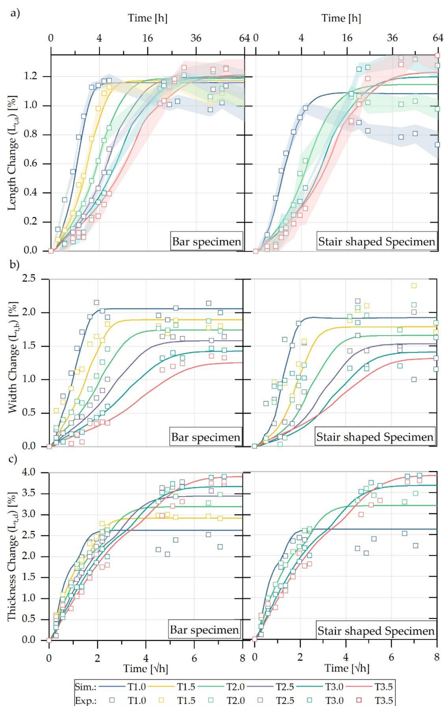
Figure 15. Comparison of the experimentally and computationally determined swelling curves of the different bar geometries and step-shaped part: (a) longitudinal, (b) width, and (c) thickness direction.
