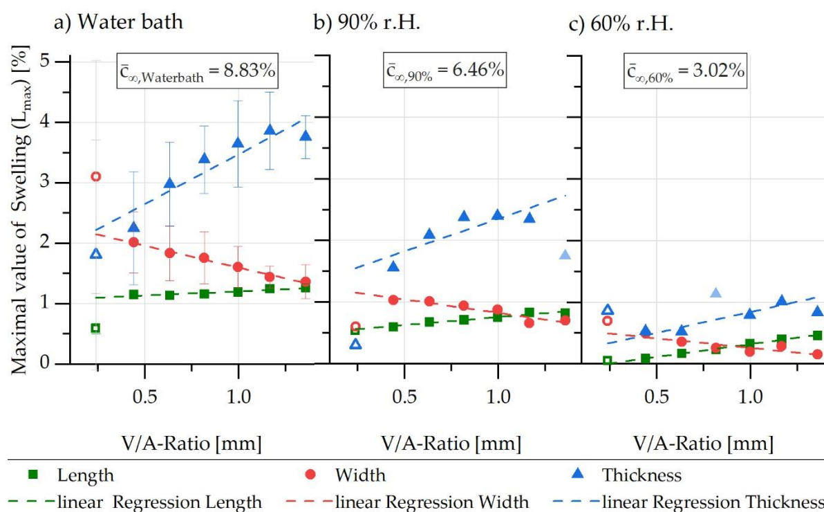
Figure 9. Maximal values of swelling in length, width, and thickness direction for different V/A ratios (a) in water bath, (b) in 90% r.h. and (c) in 60% r.h.
