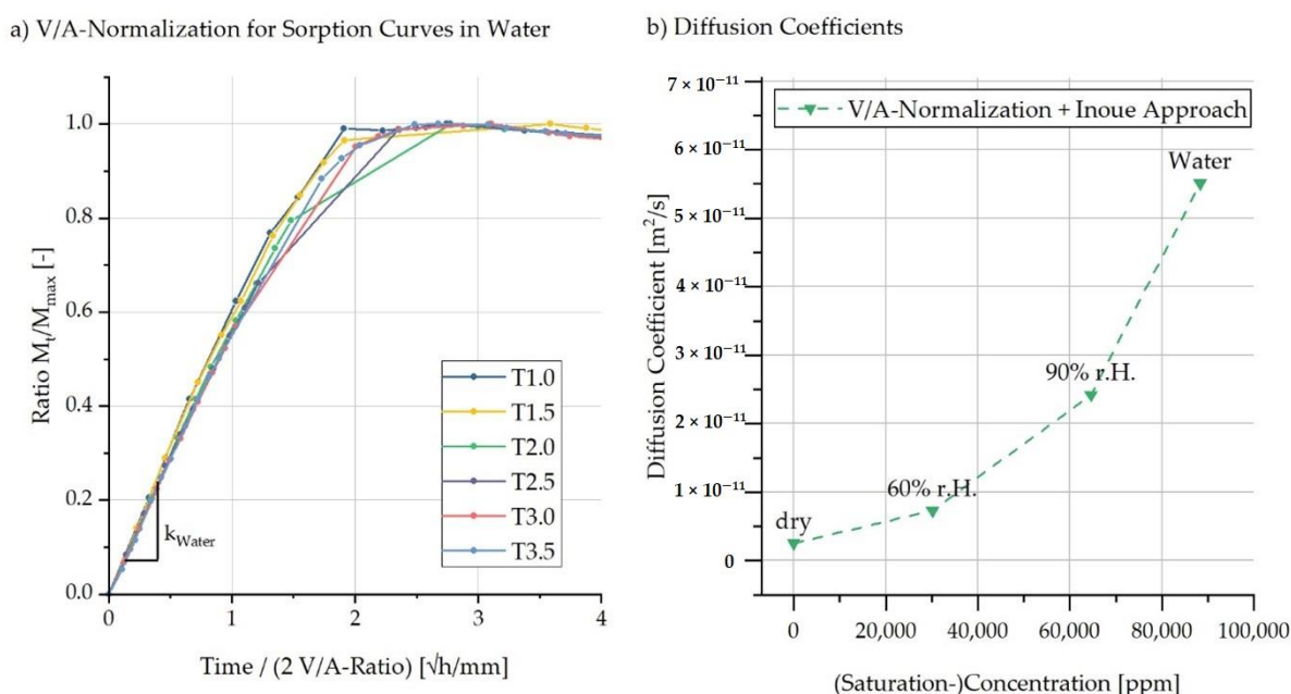
Figure 8. Determination of factor k using V/A normalisation for (a) sorption curves in water and (b) diffusion coefficients determined by V/A normalisation and the Inoue approach for different (saturation) concentrations.
